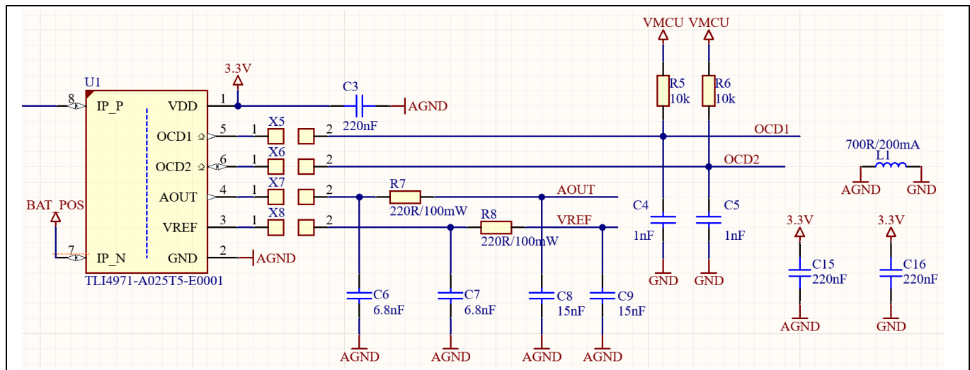
Figure 12 Current sensor for SoC and SoH estimation
