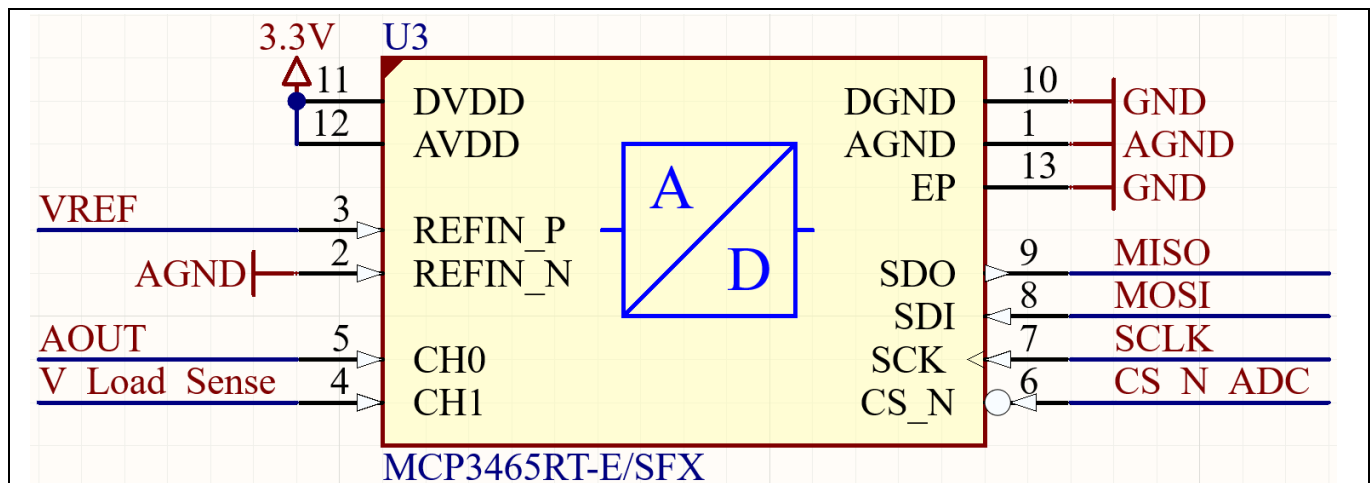
Figure 13 16-bit ADC for accurate SoC and SoH estimation
