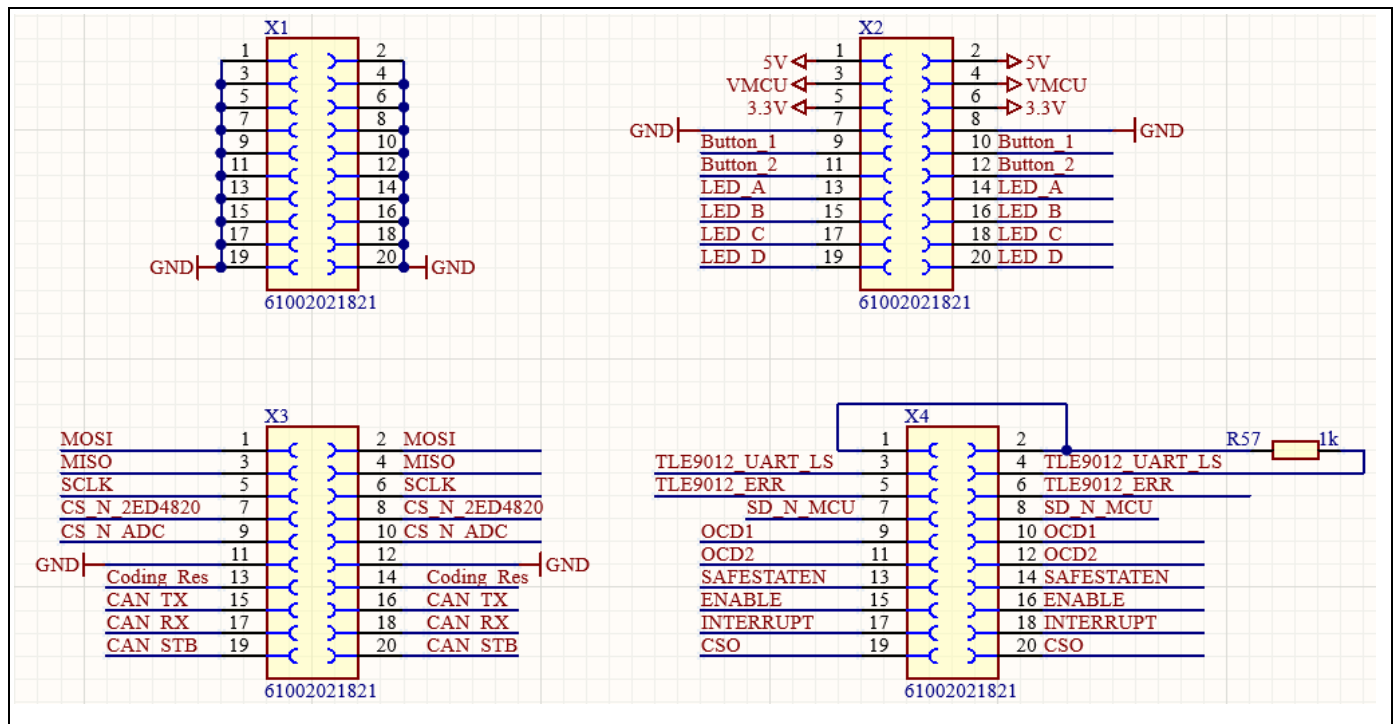
Figure 17 Interface to the piggyback board
