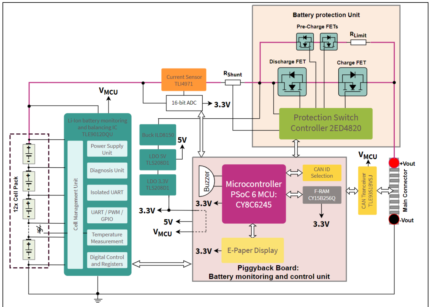
Figure 5 Block diagram of the full BMS, showing both DEMO_IMR_BMSPWR_V1 and DEMO_IMR_BMSCTRL_V1 board
