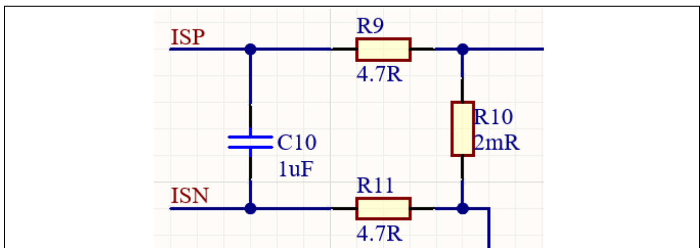
Figure 14 Shunt resistor for 2ED4820-EM
