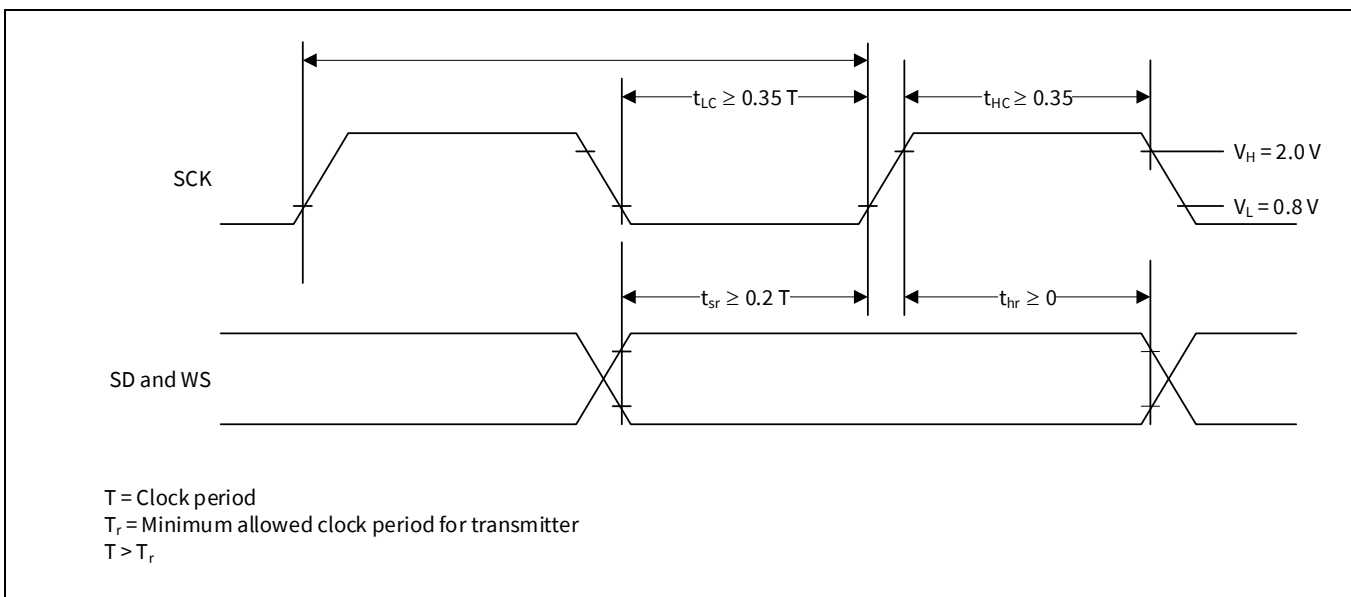
Figure 16 I²S receiver timing
