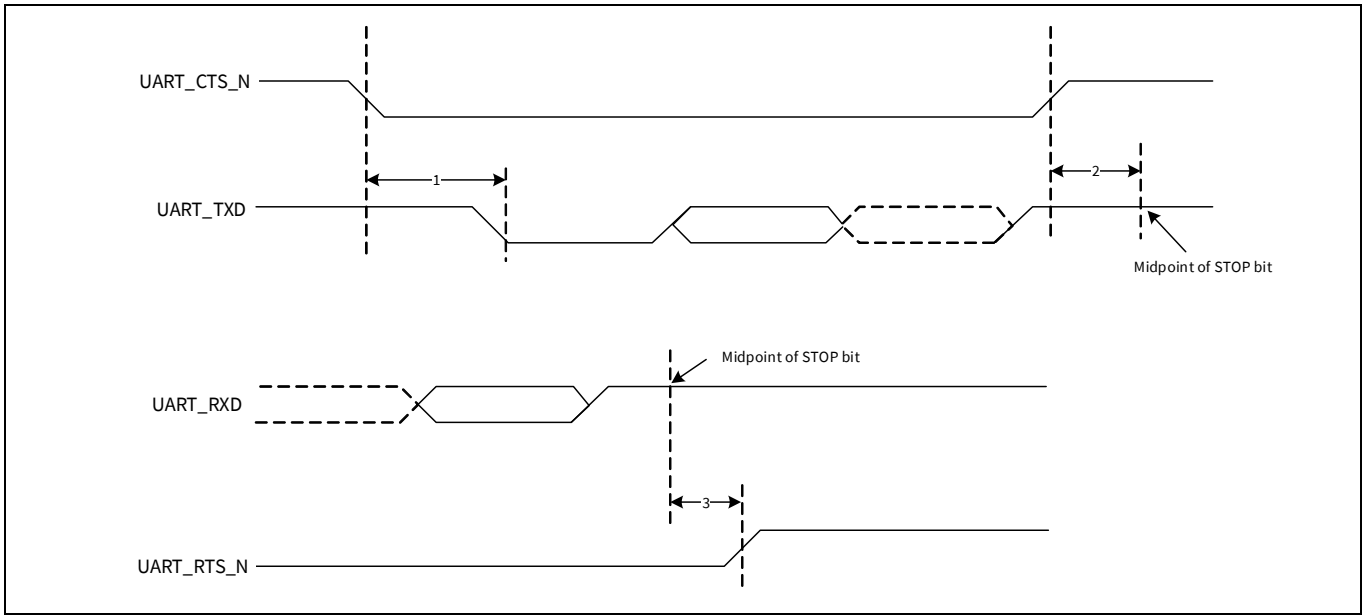
Figure 11 UART timing
