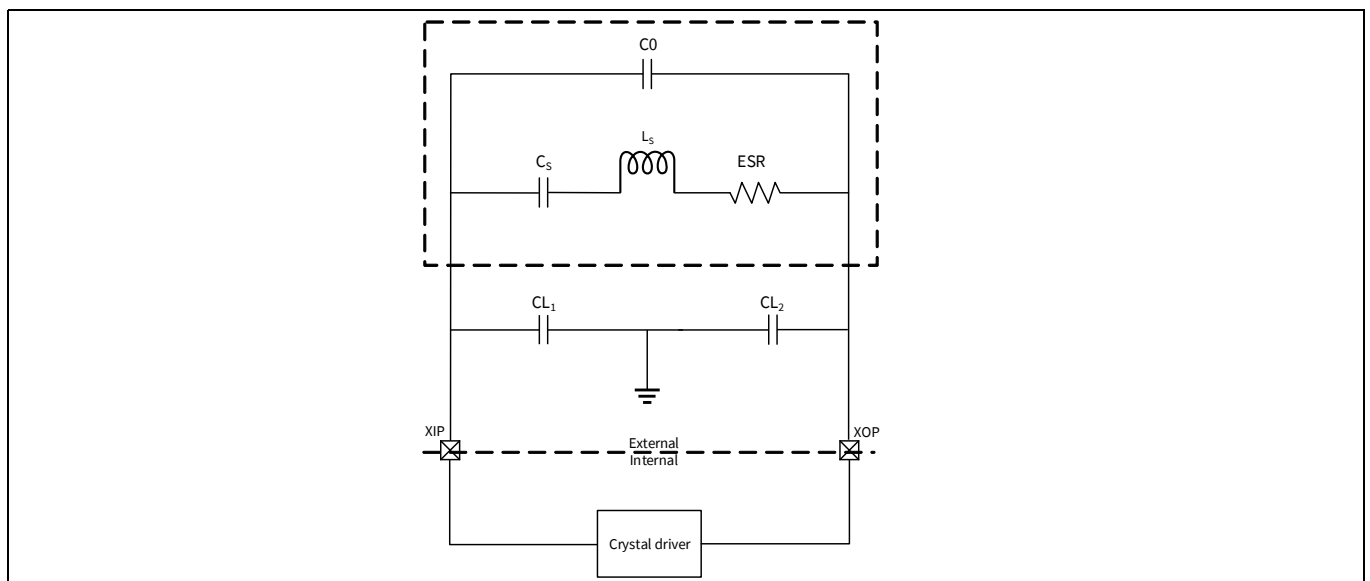
Figure 3 Oscillator circuits
