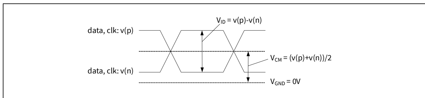
Figure 7 LVDS VCM and VID illustration
