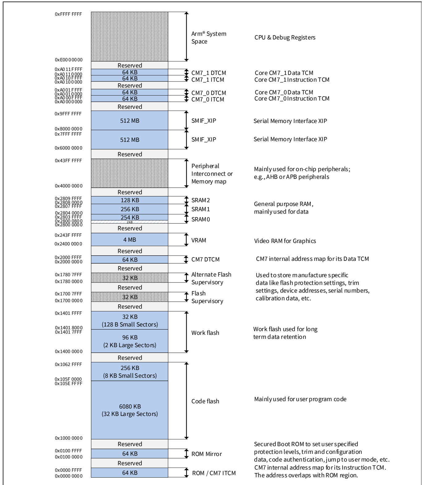
Figure 4-1 CYT4DN address map [19, 20]
