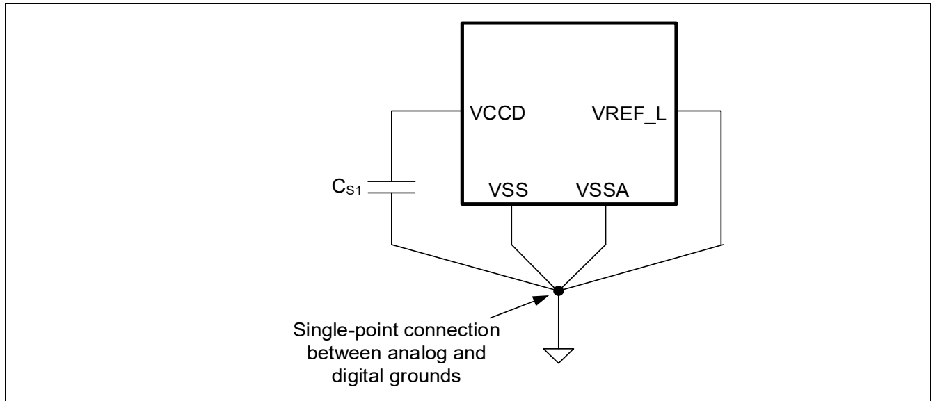
Figure 26-2 Smoothing capacitor
