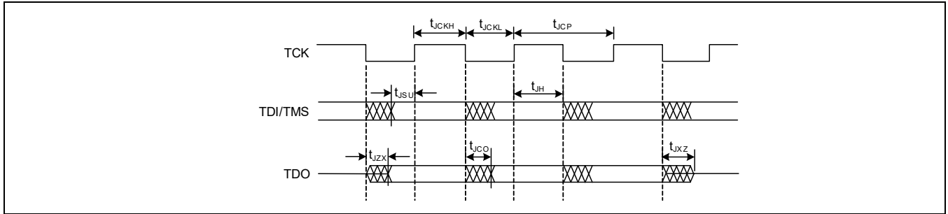
Figure 26-21 JTAG specifications
