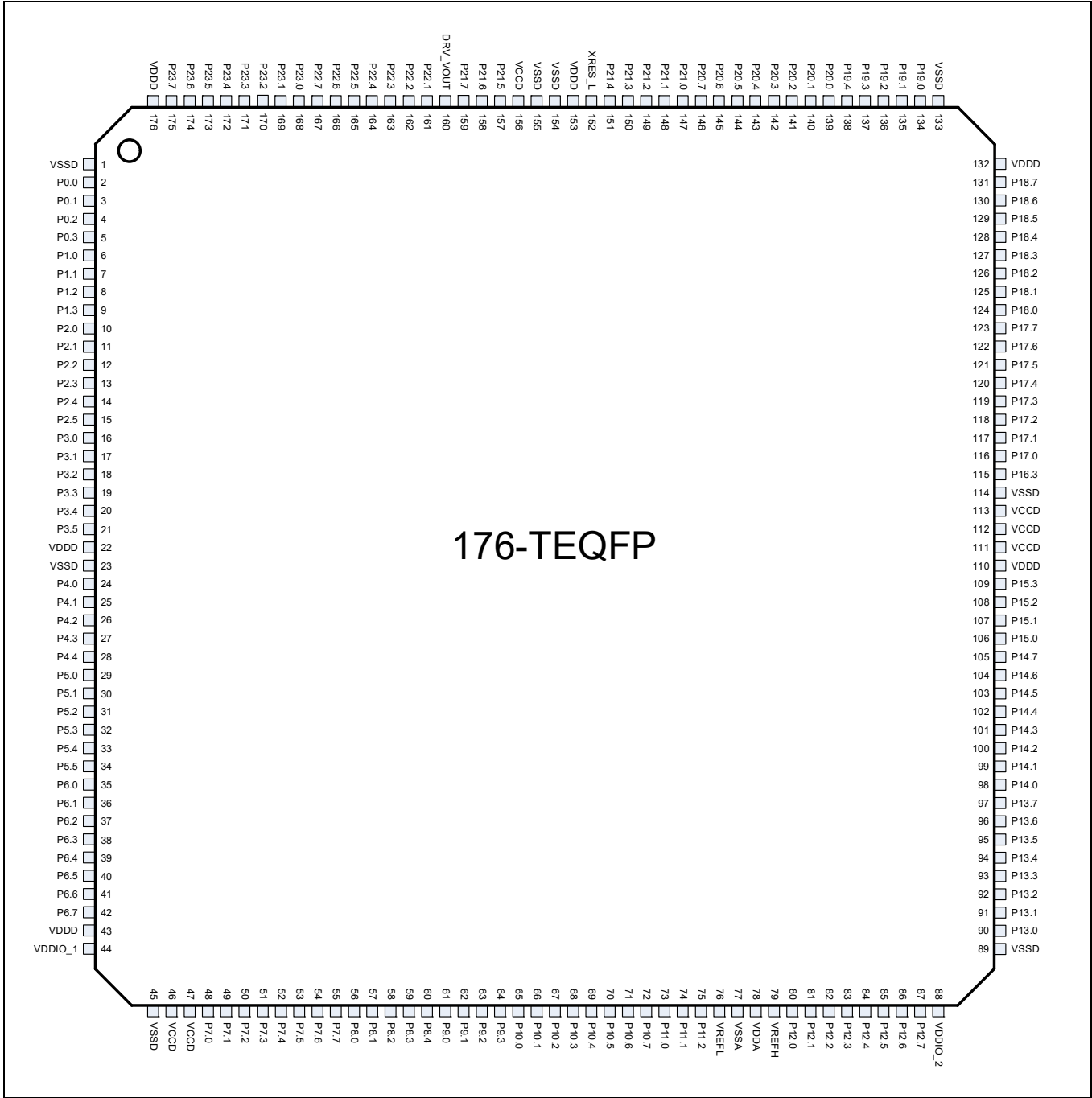
Figure 5 176-TEQFP pin assignment
