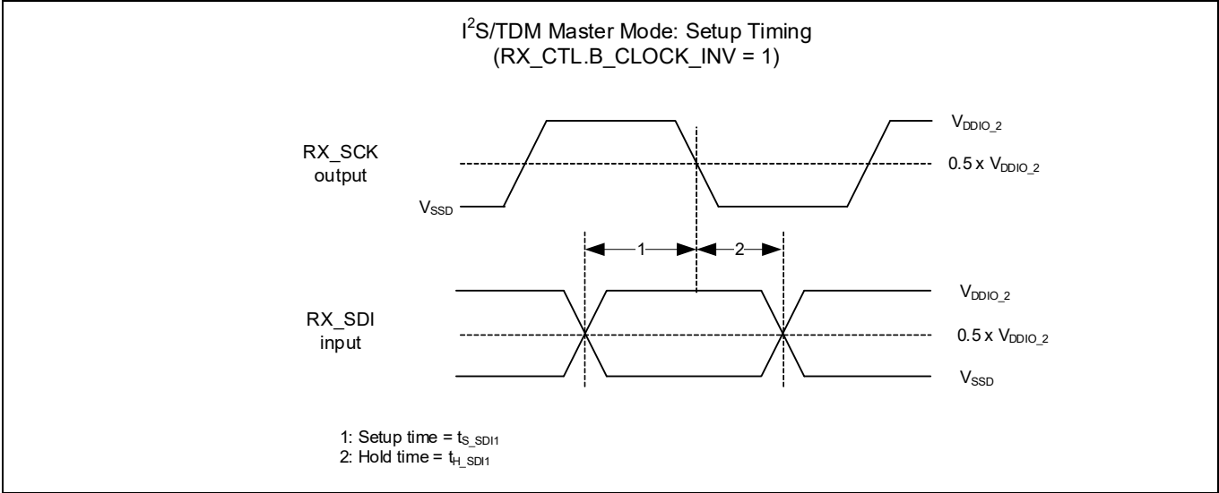
Figure 47 Master setup with clock inversion
