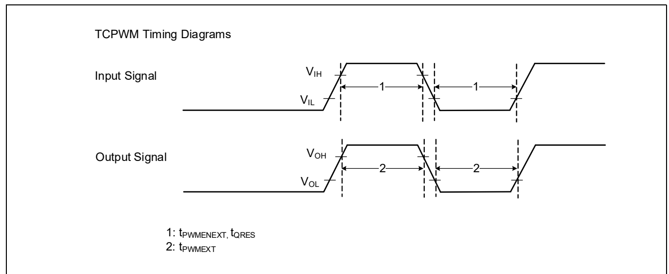
Figure 18 TCPWM timing diagrams
