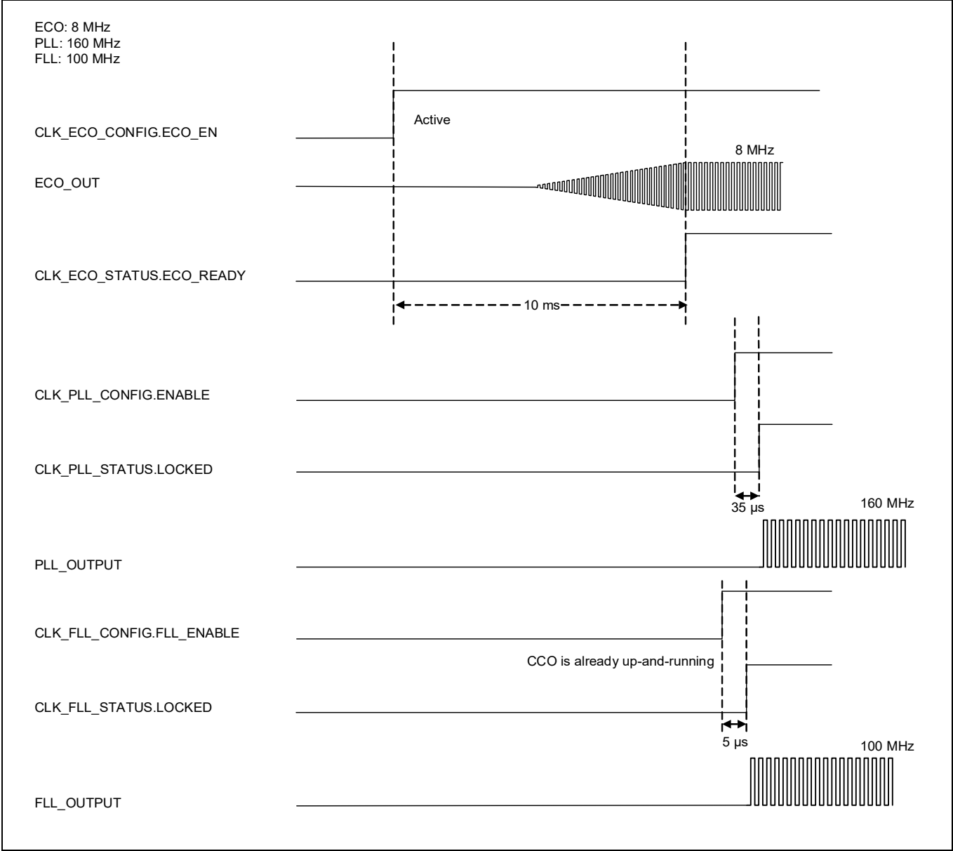
Figure 34 ECO to PLL or FLL diagram
