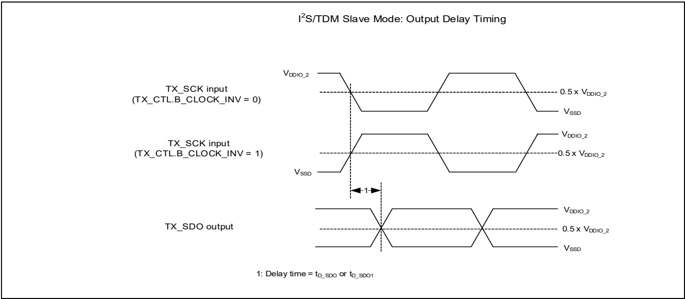
Figure 48 Slave output delay
