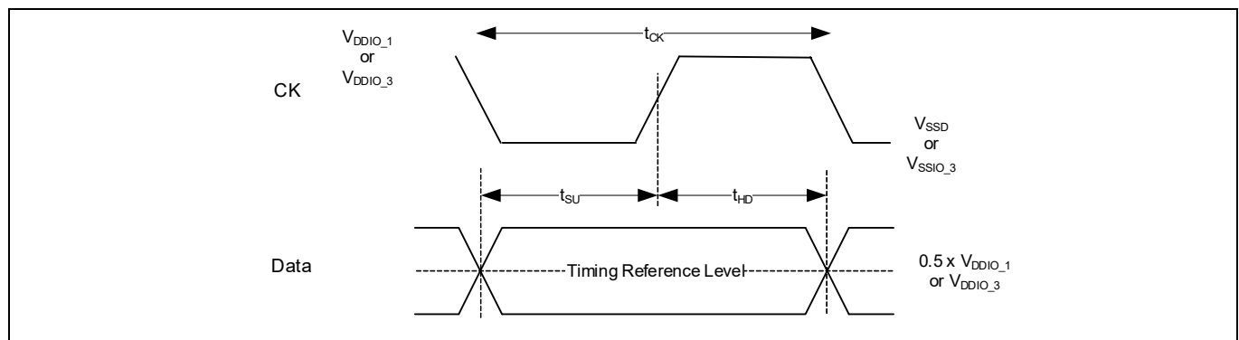
Figure 50 SDR write timing reference level
