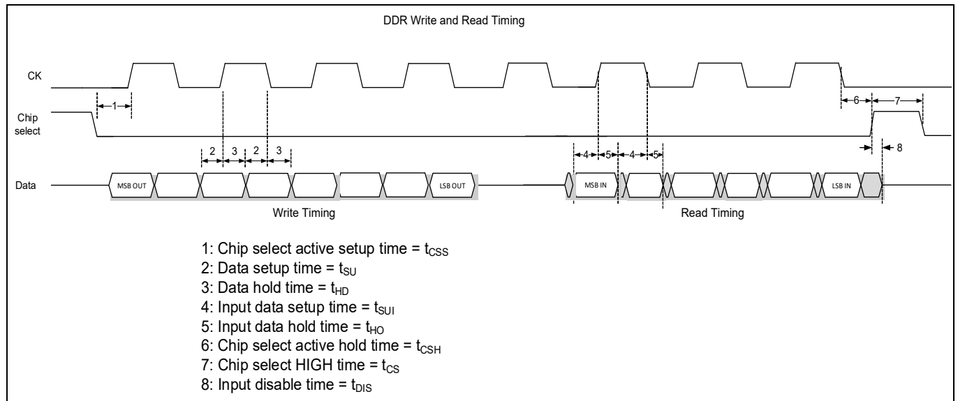
Figure 55 DDR write and read timing diagram
