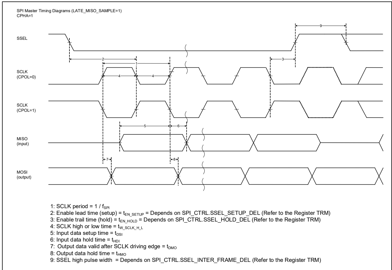
Figure 21 SPI master timing diagrams with HIGH clock phase
