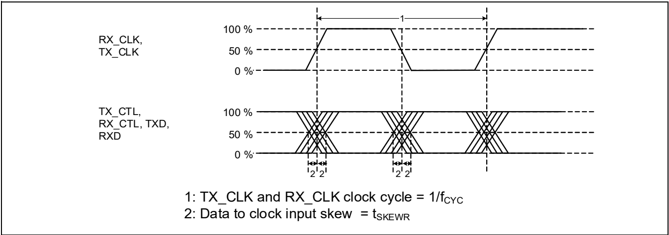
Figure 40 RGMII Rx timing diagram
