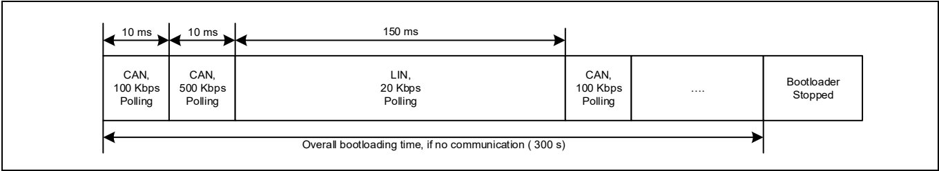
Figure 61 Bootloading sequence
