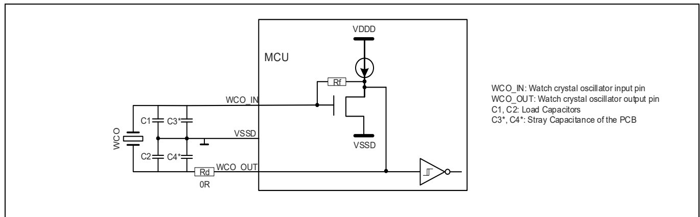
Figure 33 WCO connection scheme [67]
