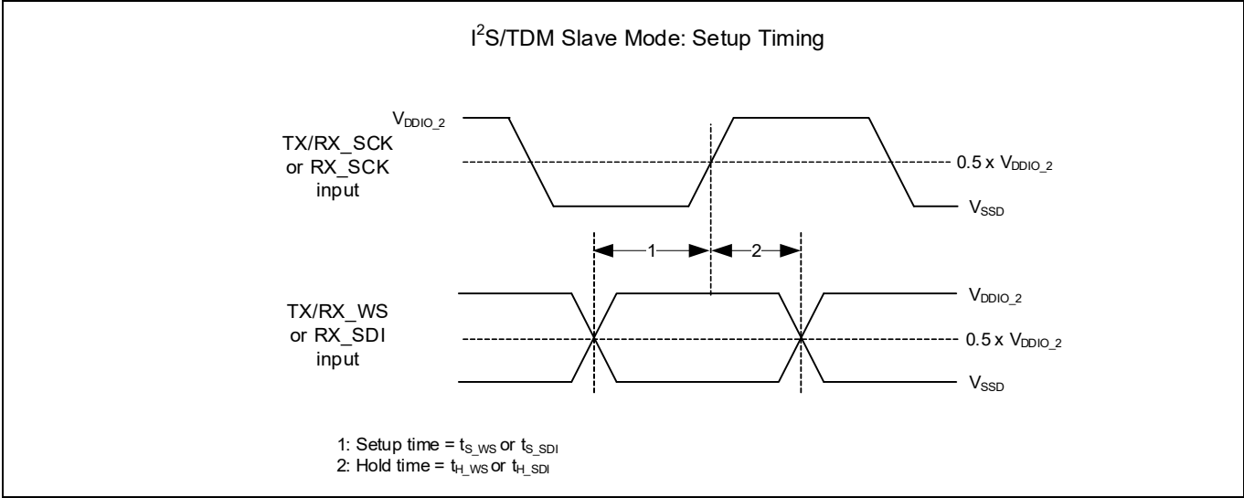
Figure 49 Slave setup
