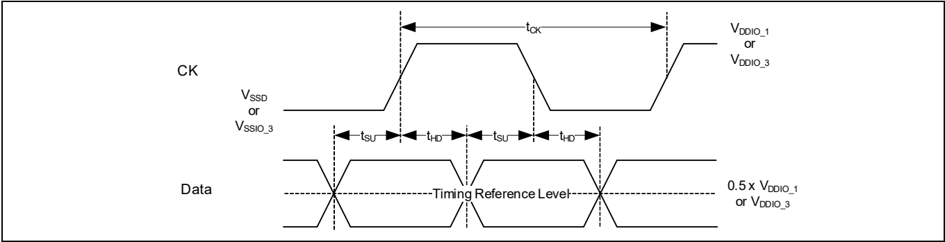
Figure 52 DDR write timing reference level
