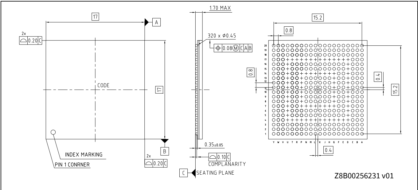
Figure 60 Package outline - 320-BGA
