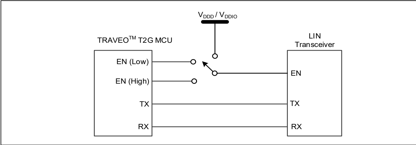
Figure 63 MCU to LIN transceiver connections
