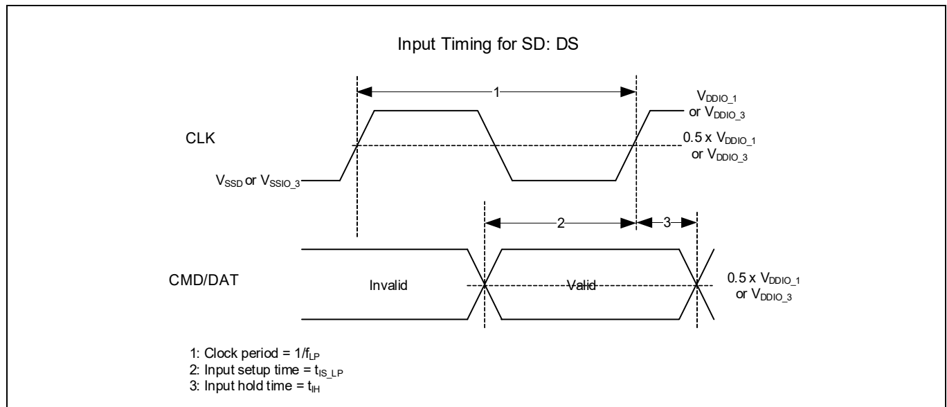
Figure 41 SD default speed input timing
