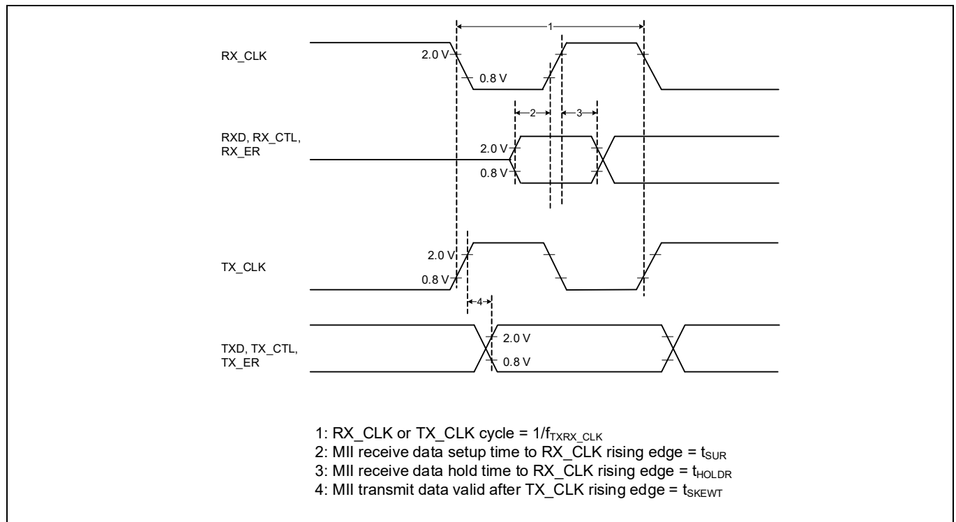
Figure 36 MII timing diagram
