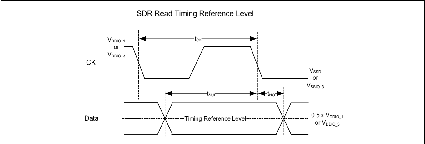
Figure 51 SDR read timing reference level
