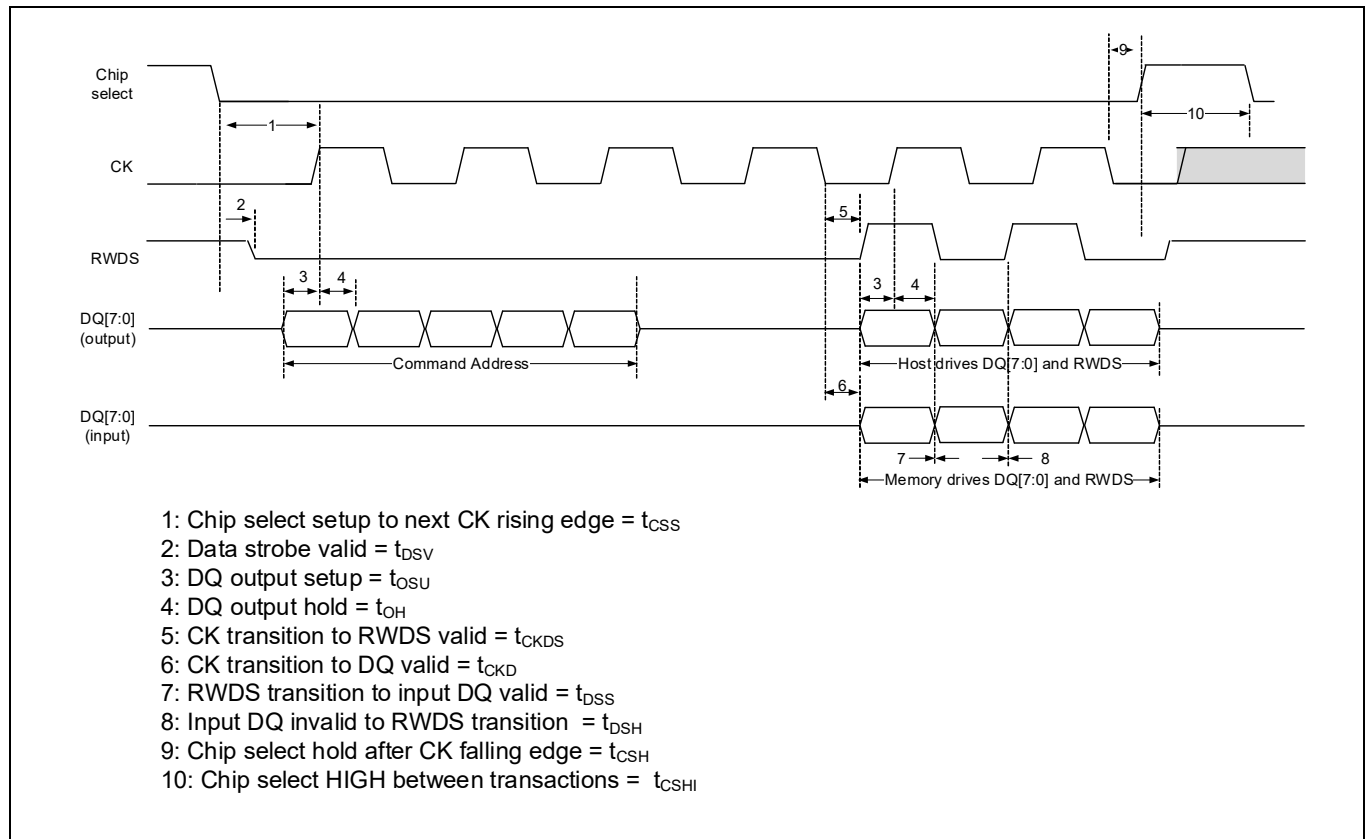
Figure 57 HYPERBUS™ timing diagram
