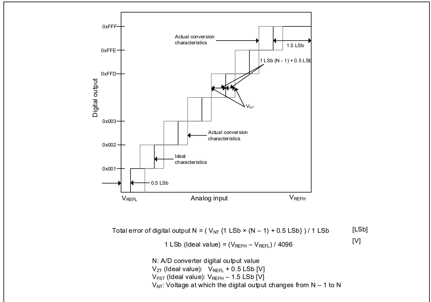
Figure 14 ADC characteristics and error descriptions
