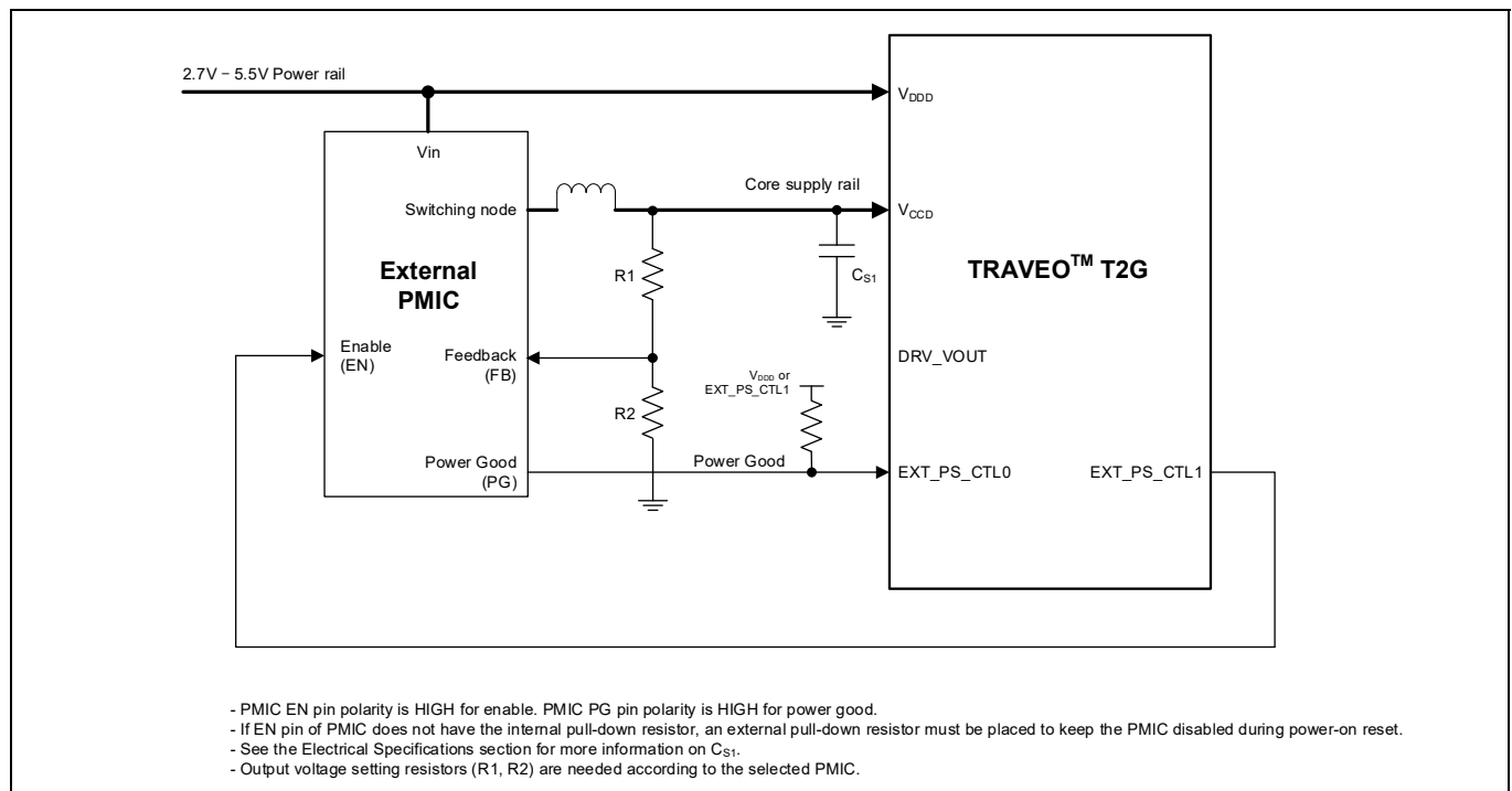
Figure 2 Sample core external regulator with PMIC/LDO
