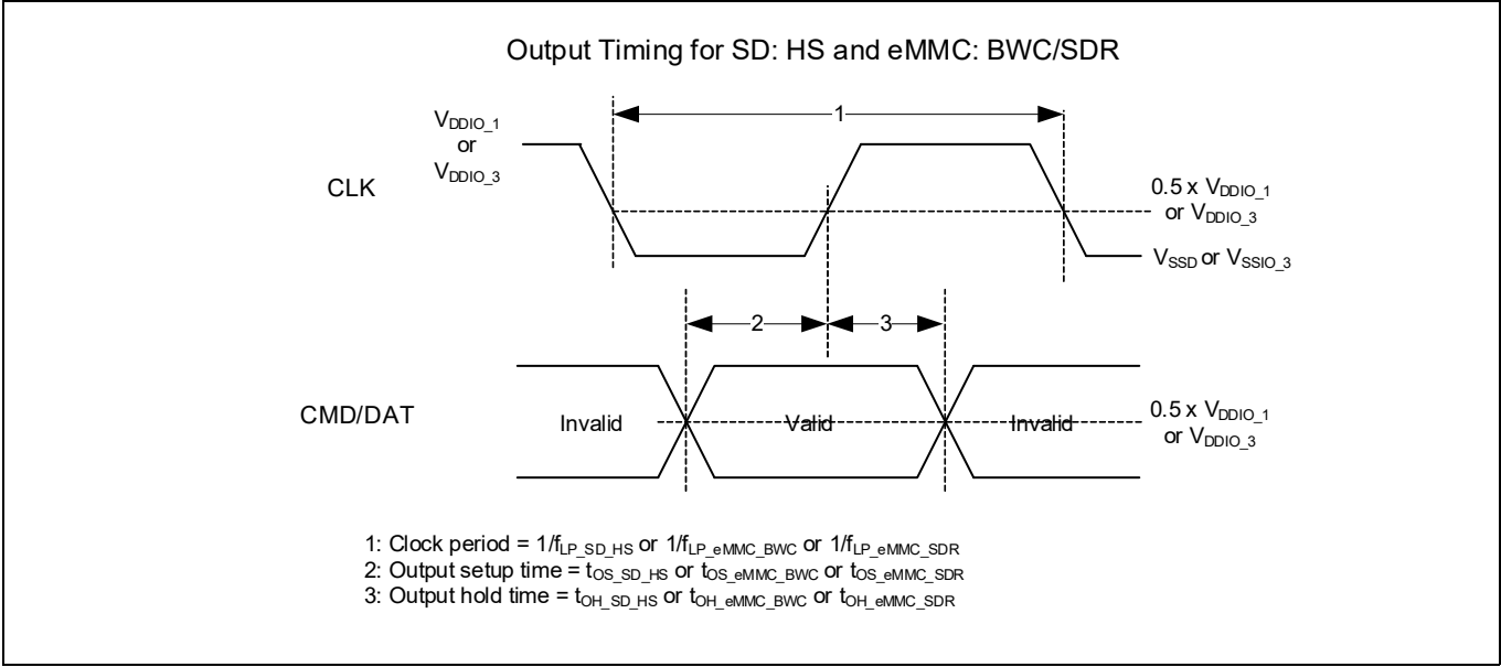
Figure 44 SD high-speed and eMMC BWC/SDR output timing
