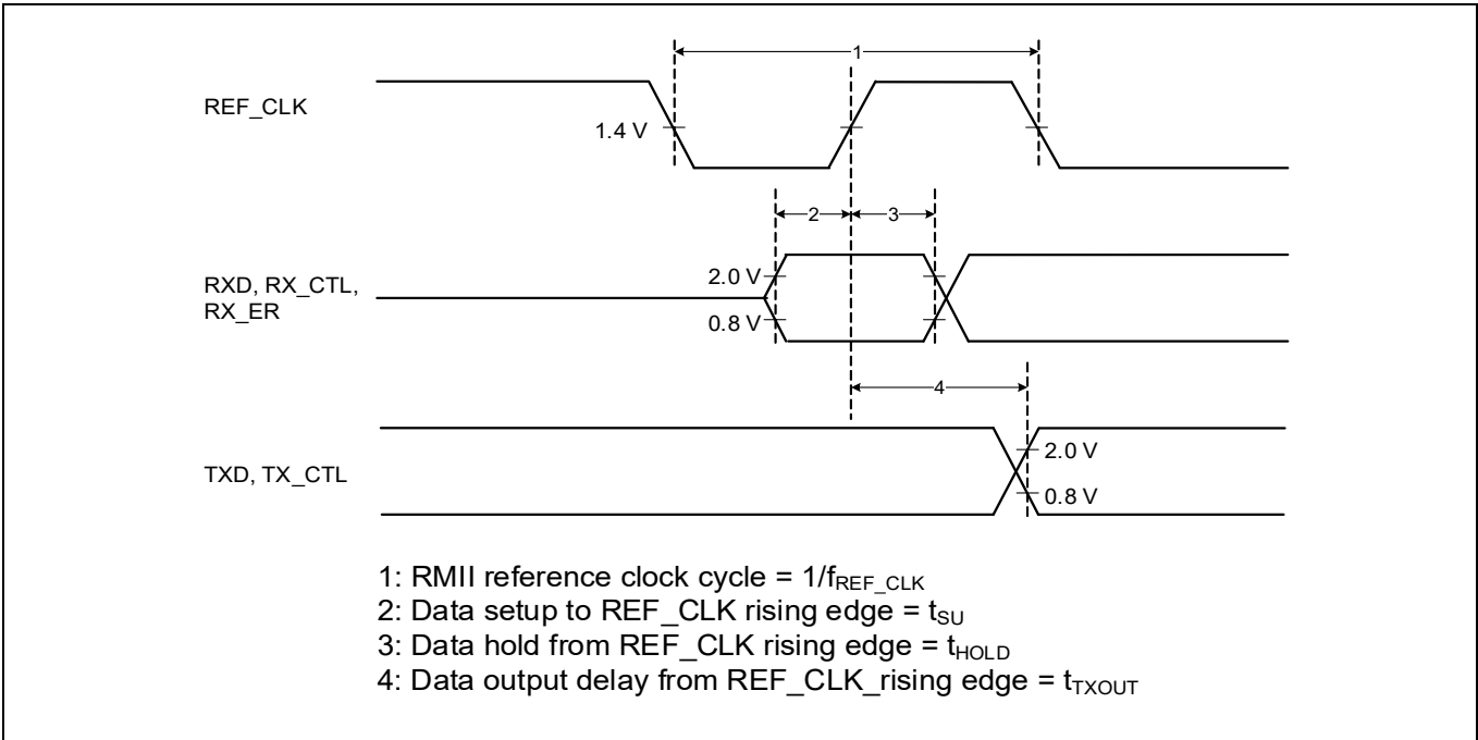
Figure 38 RMII timing diagram
