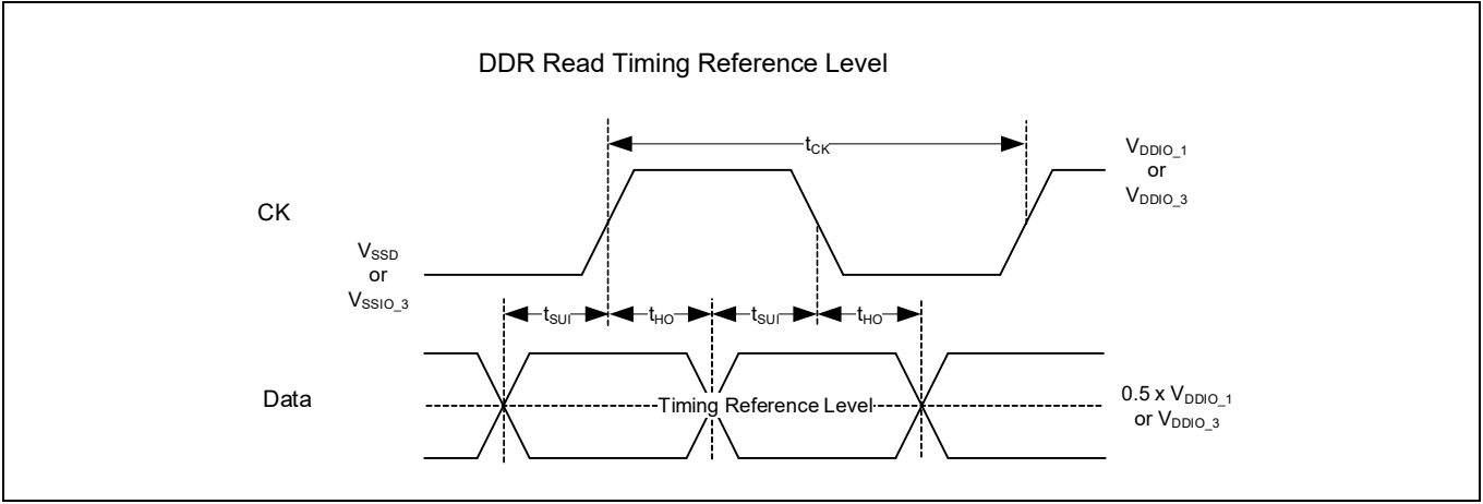
Figure 53 DDR read timing reference level
