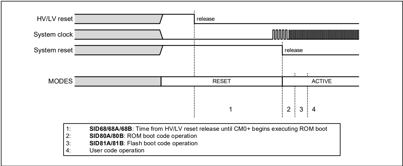
Figure 13 Reset sequence
