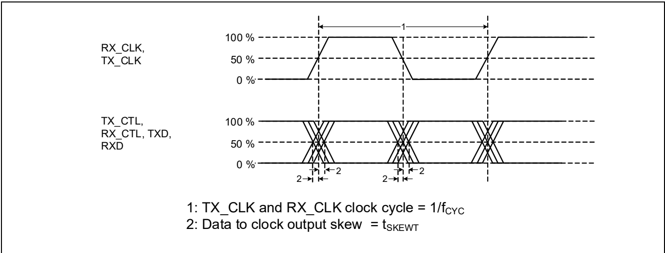
Figure 39 RGMII Tx timing diagram
