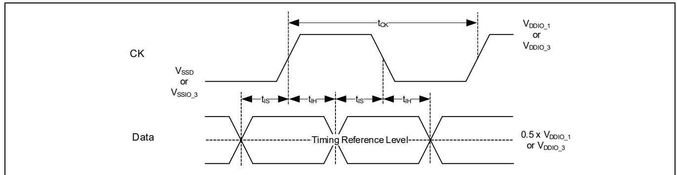
Figure 56 HYPERBUS™ timing reference level
