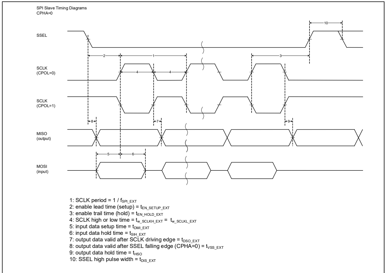
Figure 22 SPI slave timing diagrams with LOW clock phase
