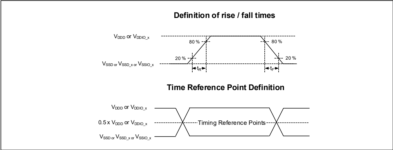
Figure 17 AC timings specifications
