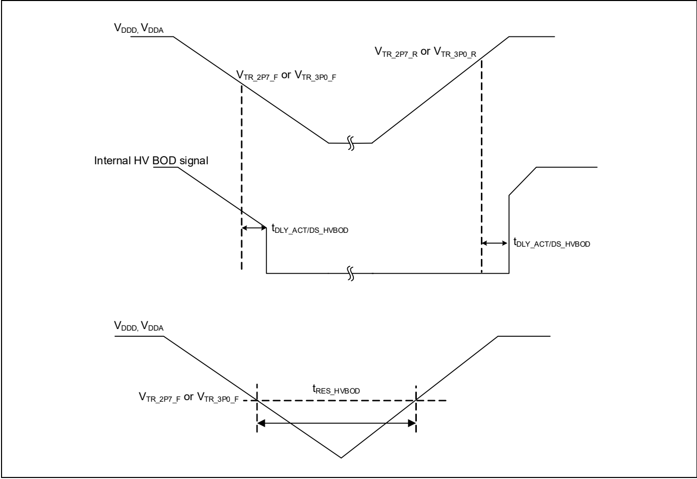
Figure 26 High-voltage BOD specifications
