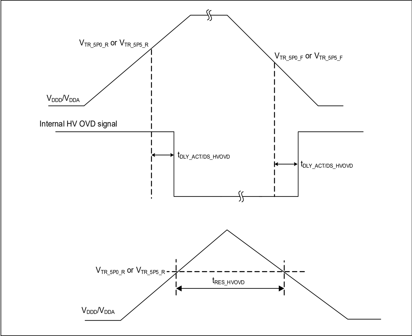
Figure 28 High-voltage OVD specifications
