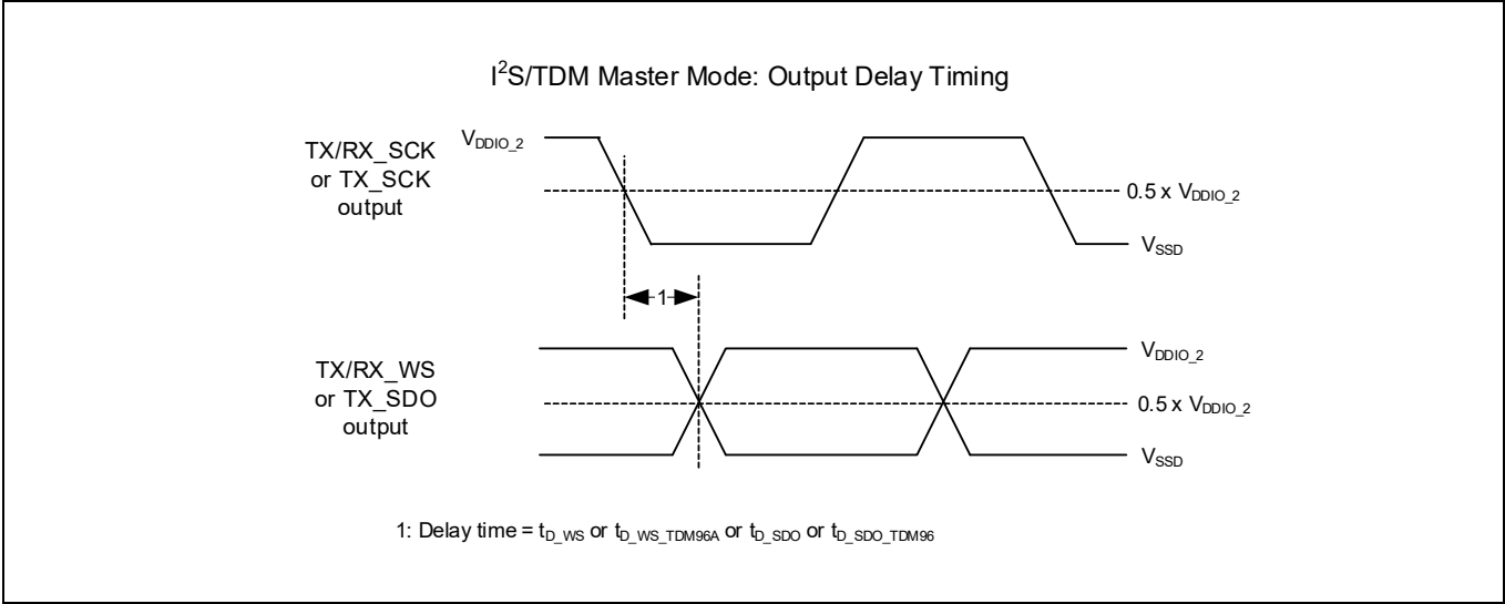
Figure 45 Master output delay
