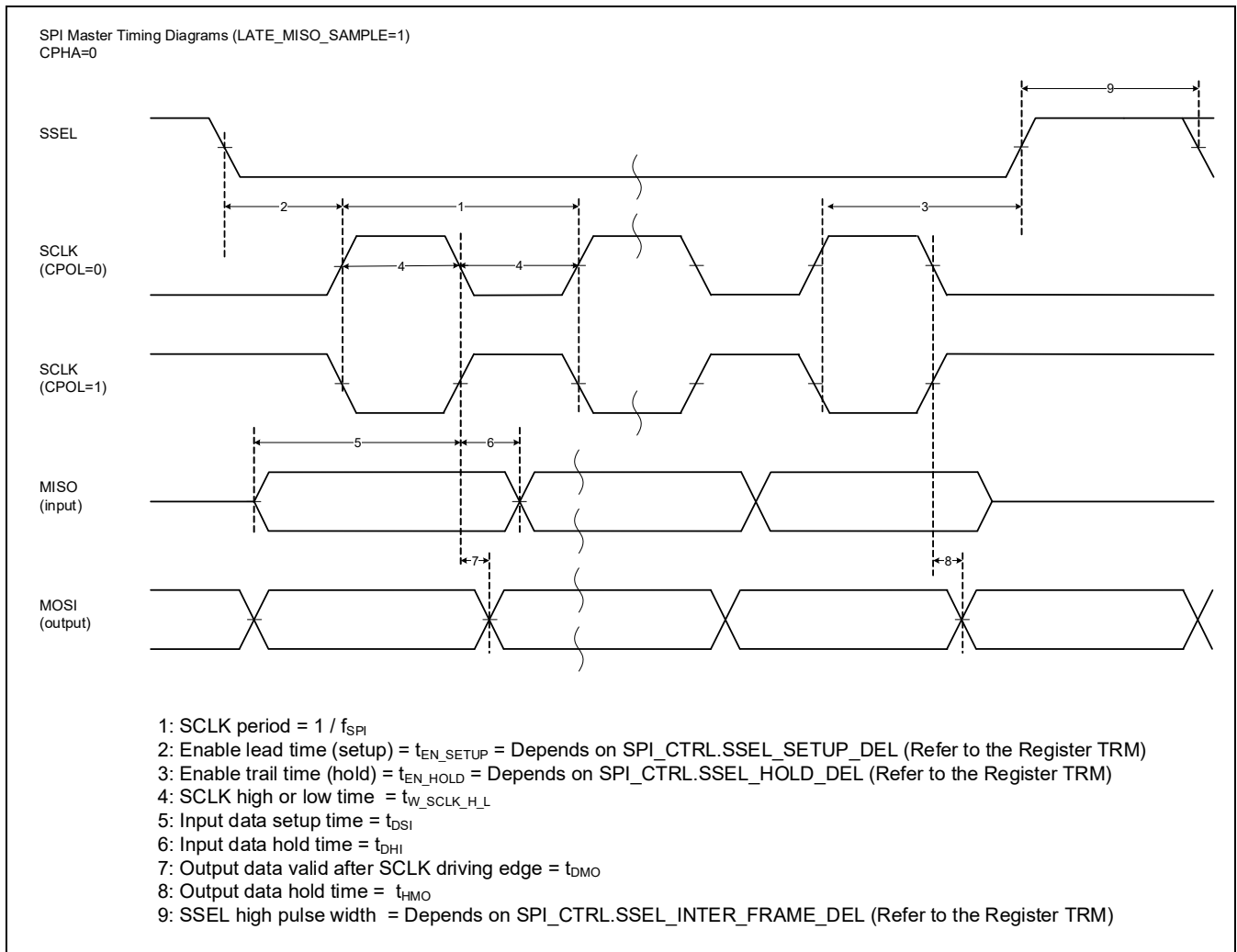
Figure 20 SPI master timing diagrams with LOW clock phase
