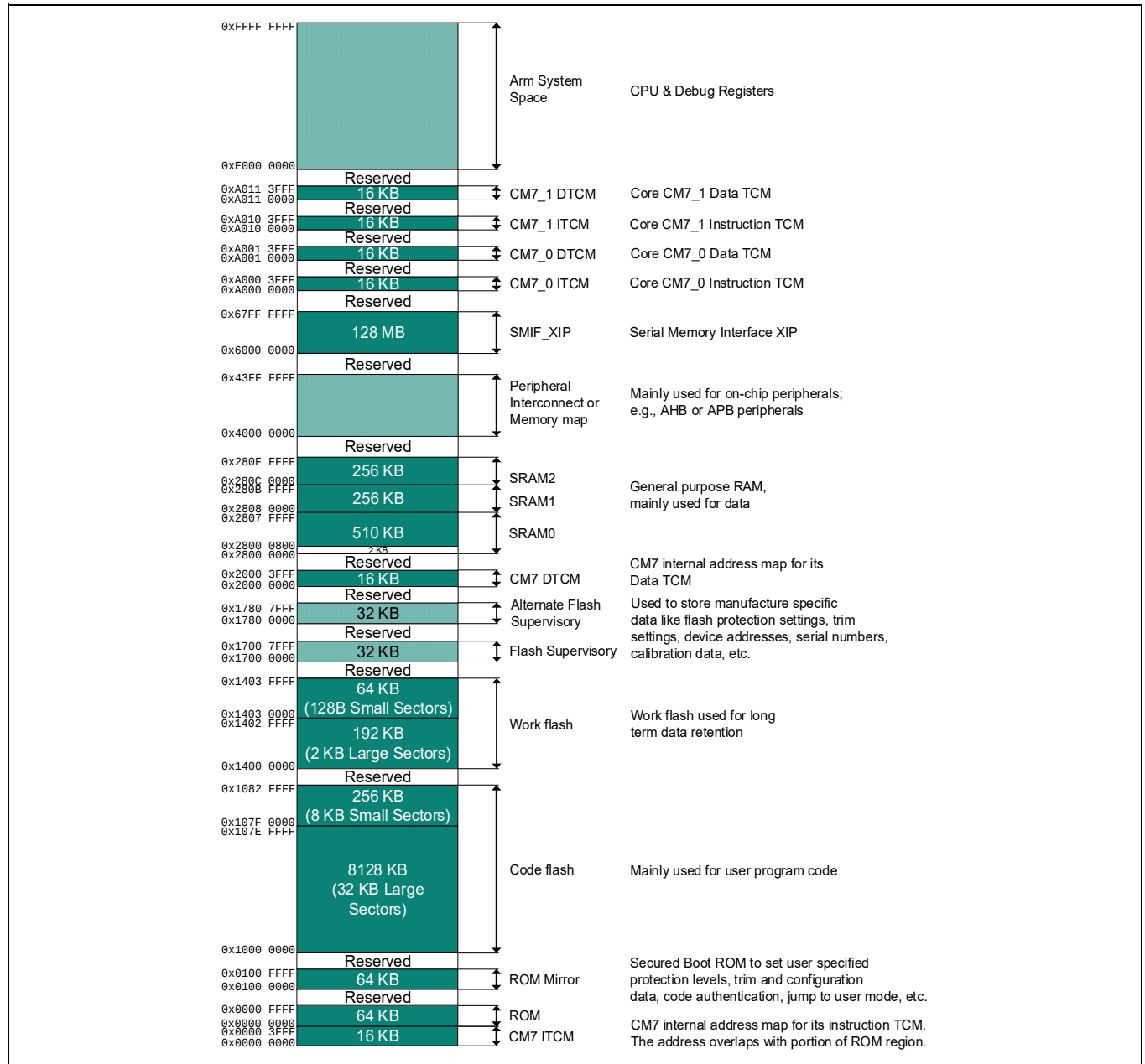
Figure 3 CYT4BF address map [13, 14]
