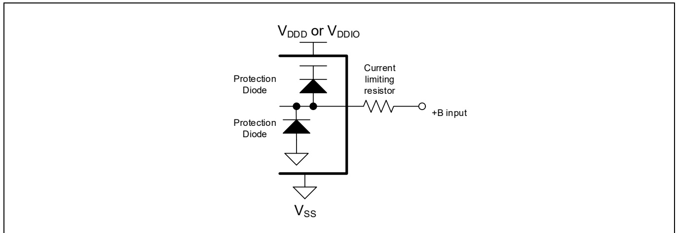
Figure 11 Example of a recommended circuit [45]
