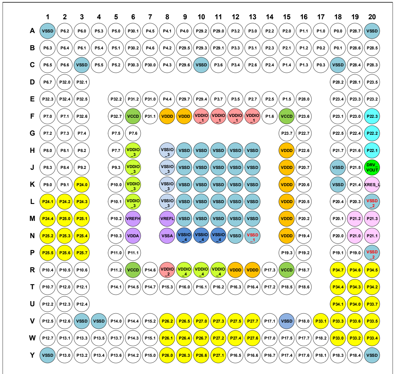
Figure 8 320-BGA ball map
