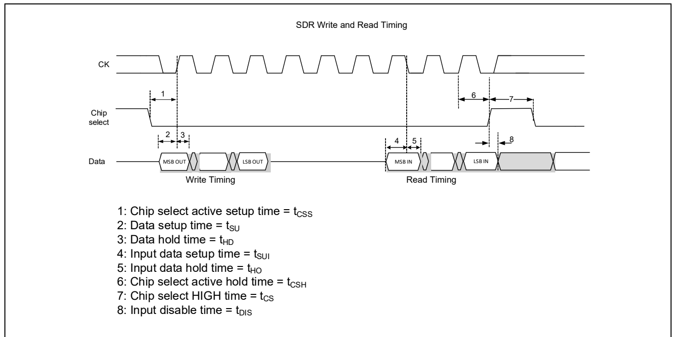
Figure 54 SDR write and read timing diagram
