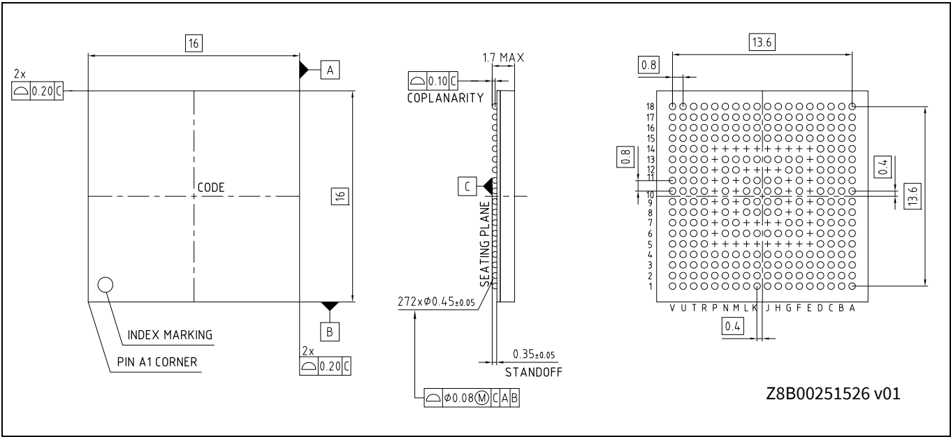
Figure 59 Package outline – 272-BGA
