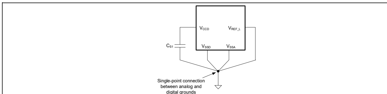
Figure 12 Smoothing capacitor
