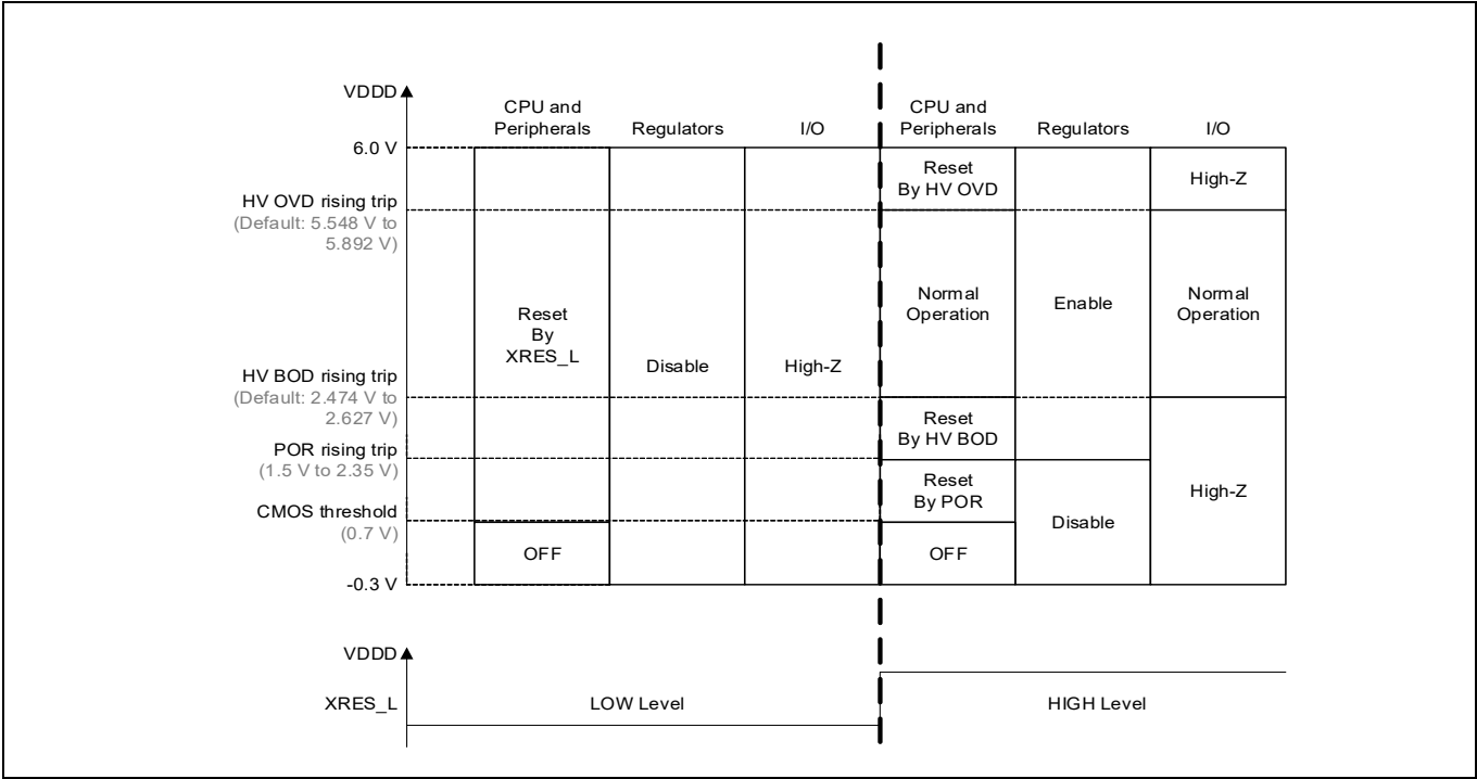
Figure 24 Device operations supply range
