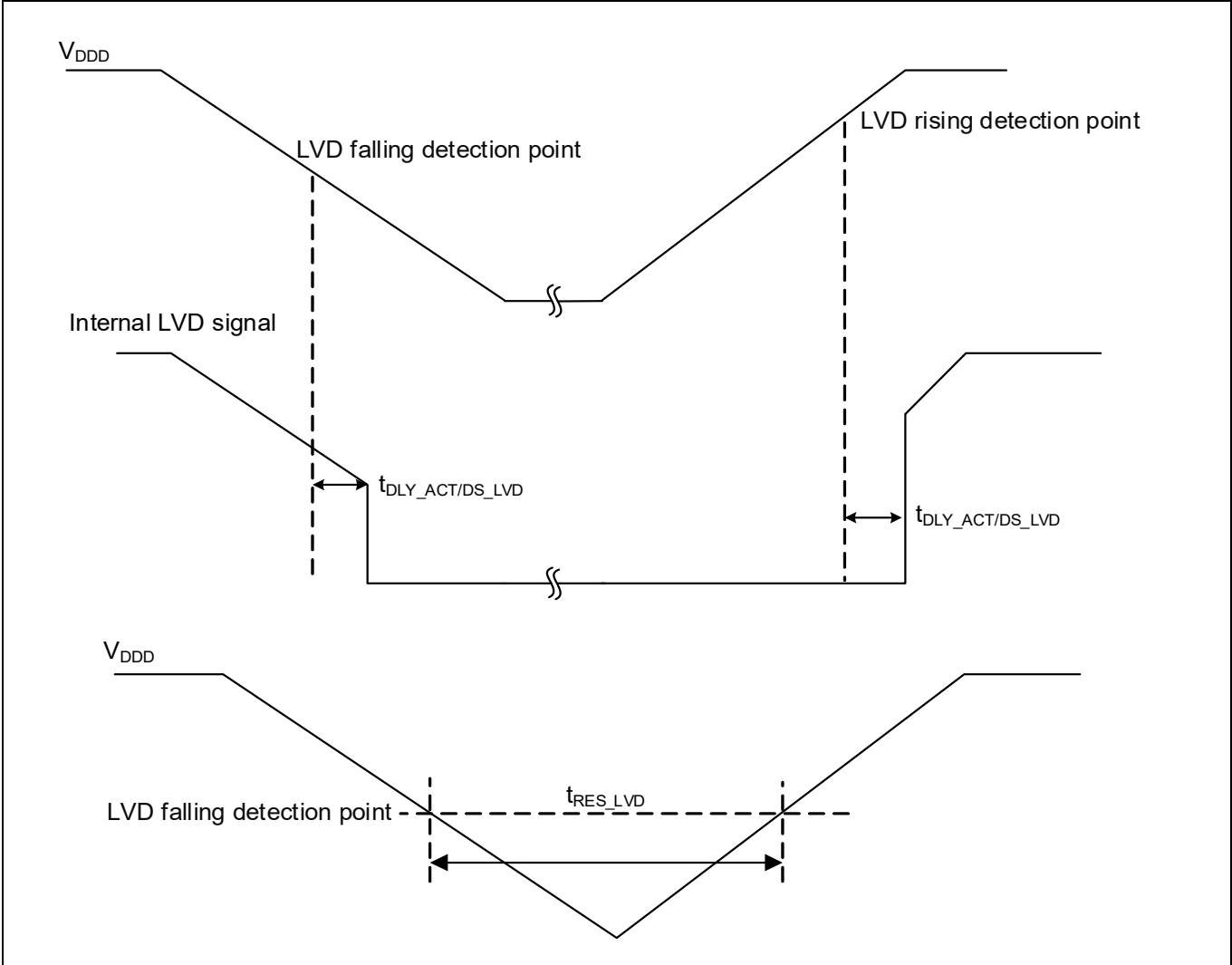
Figure 30 LVD specifications
