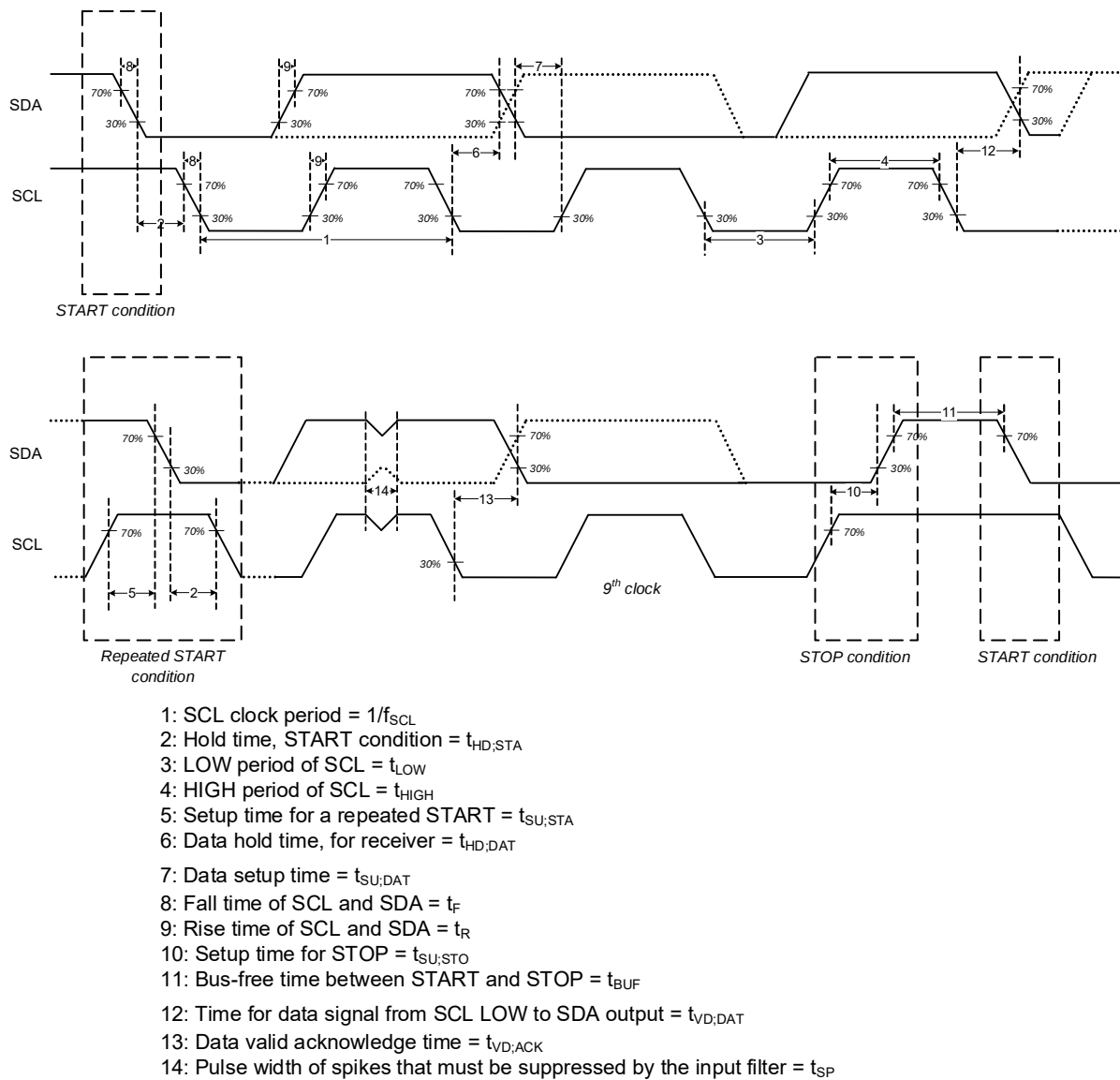
Figure 19 I 2 C timing diagrams
