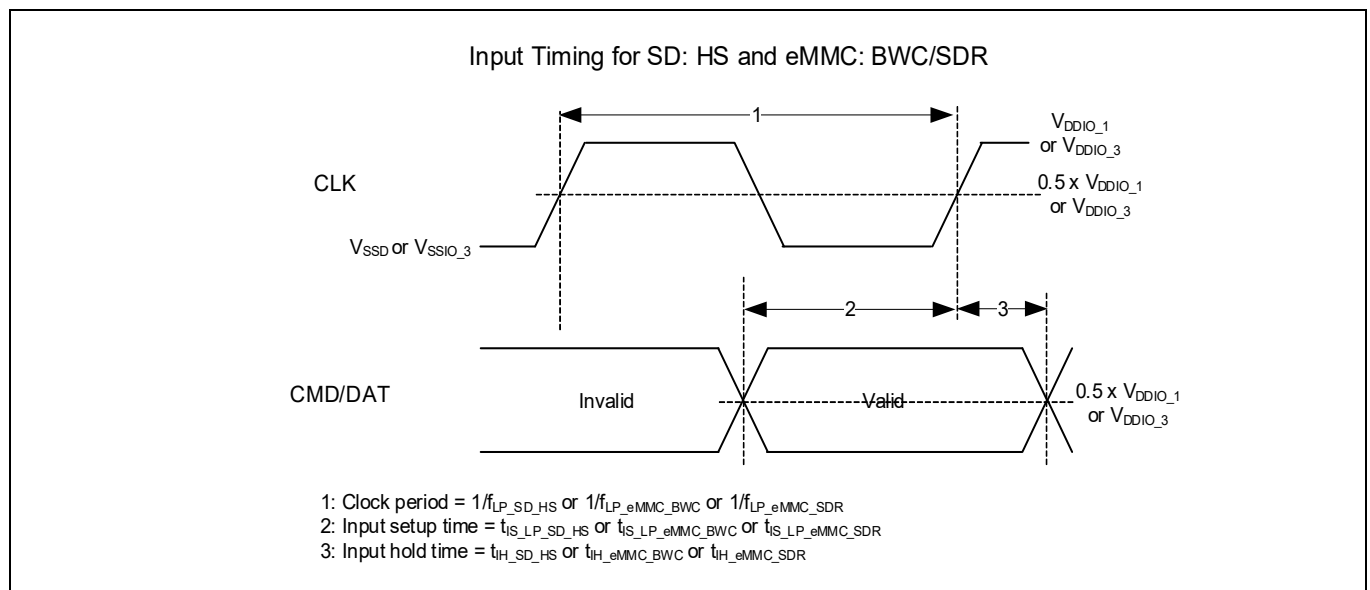
Figure 43 SD high-speed and eMMC BWC/SDR input timing
