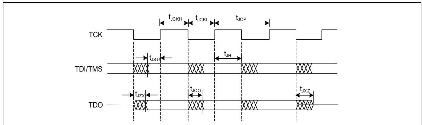
Figure 31 JTAG specifications
