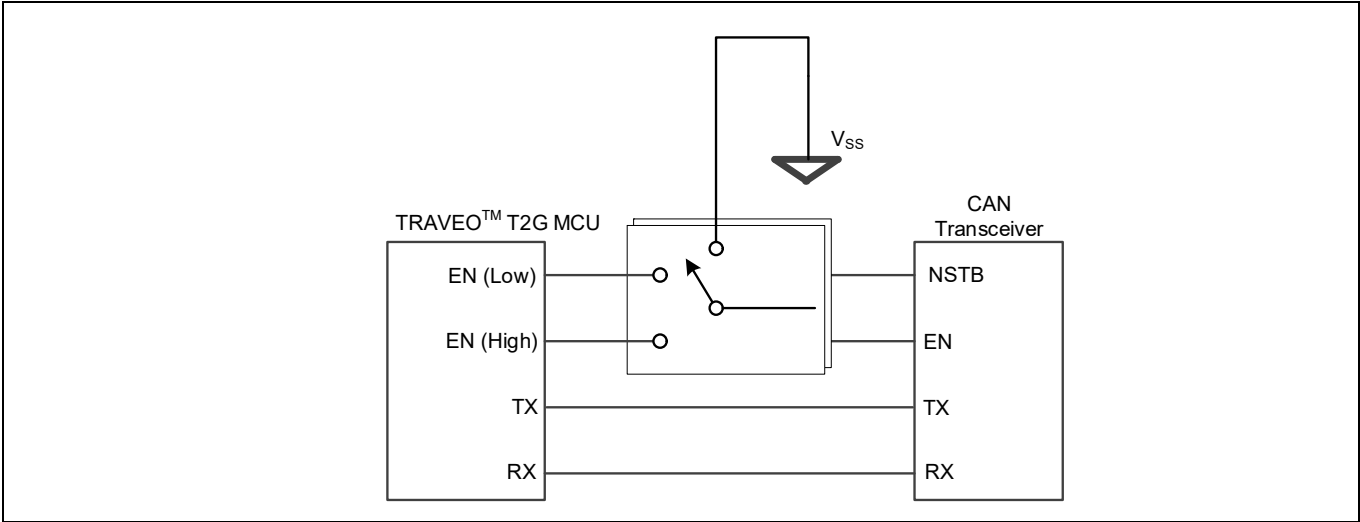
Figure 62 MCU to CAN transceiver connections
