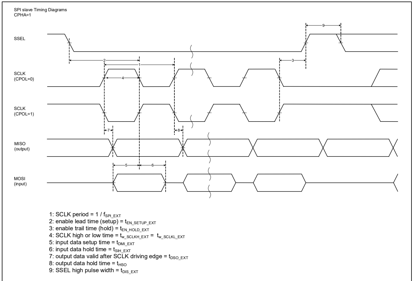
Figure 23 SPI slave timing diagrams with HIGH clock phase
