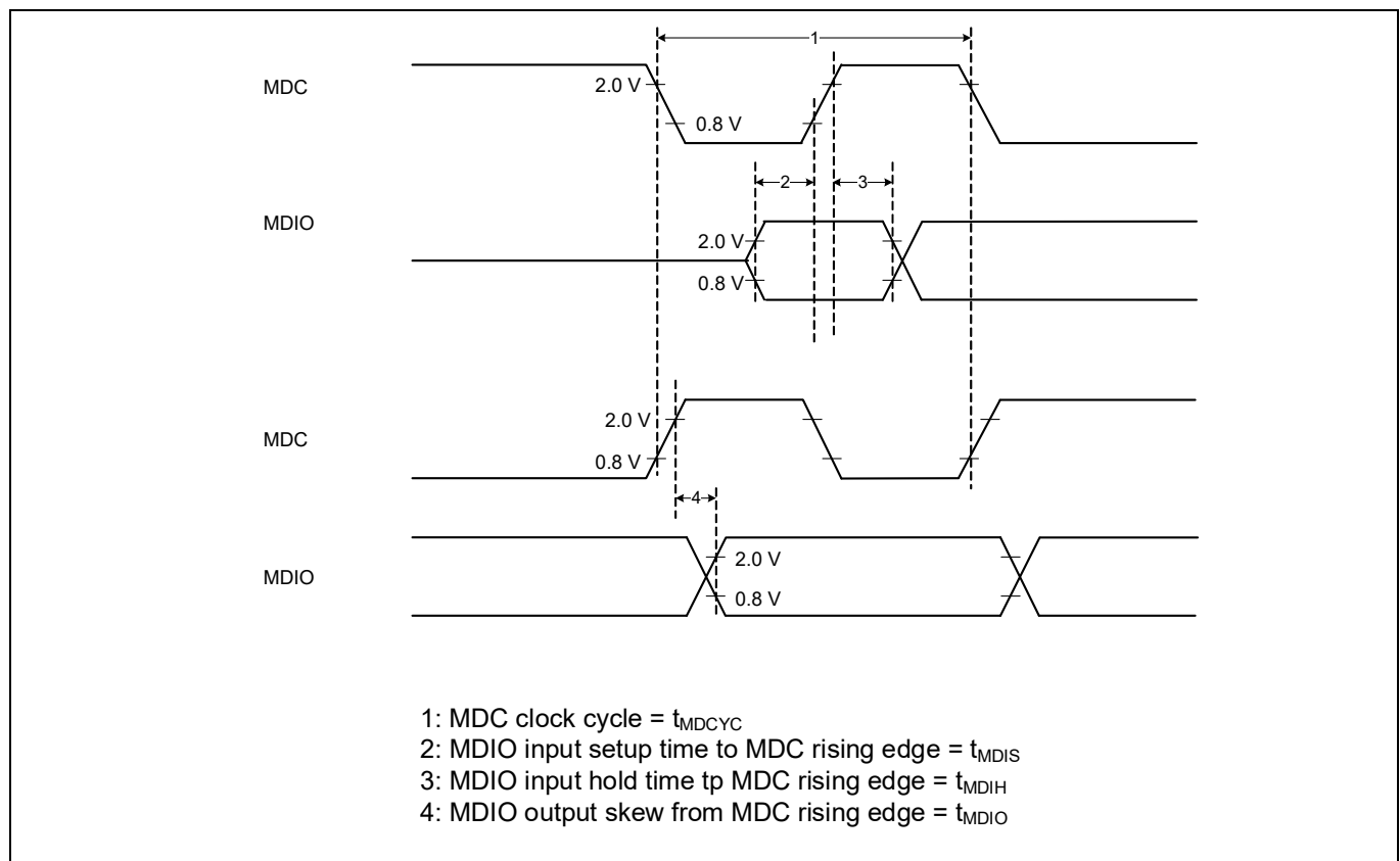
Figure 37 MDIO timing diagram
