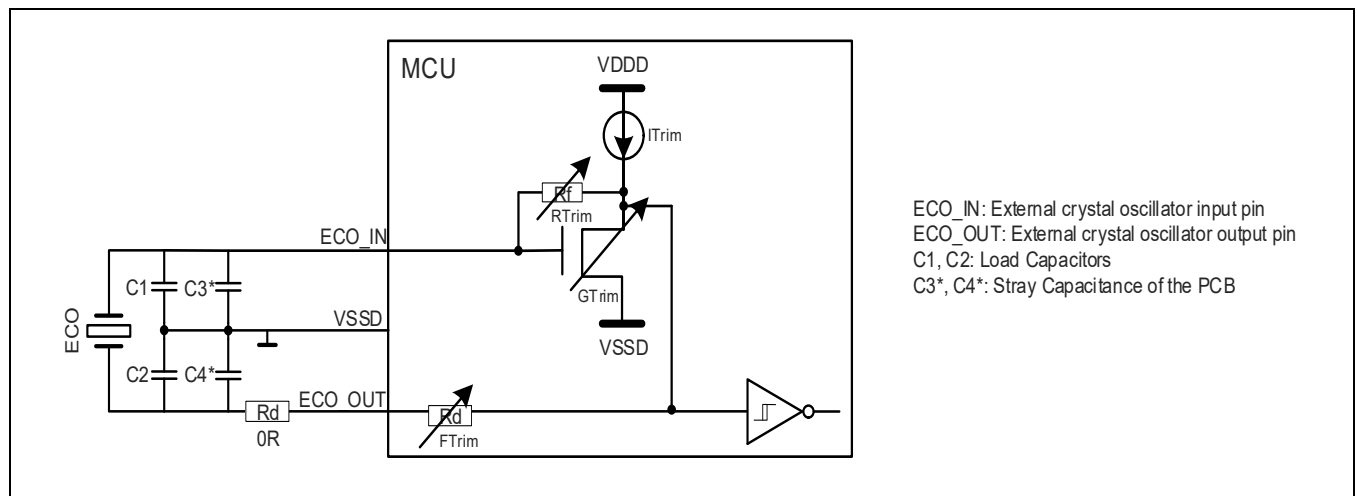
Figure 32 ECO connection scheme [65]
