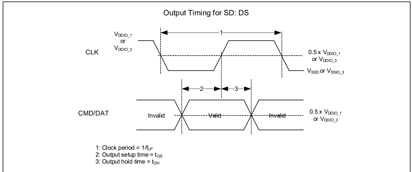
Figure 42 SD default speed output timing
