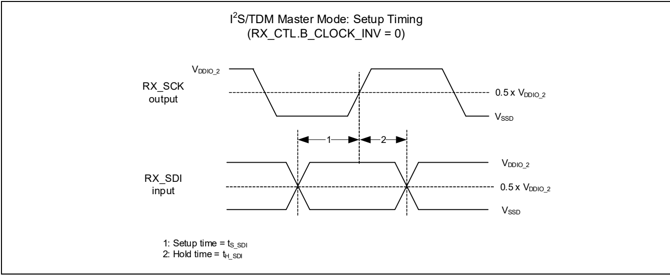
Figure 46 Master setup without clock inversion
