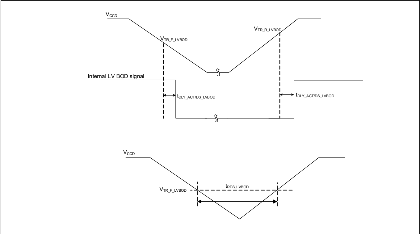
Figure 27 Low-voltage BOD specifications
