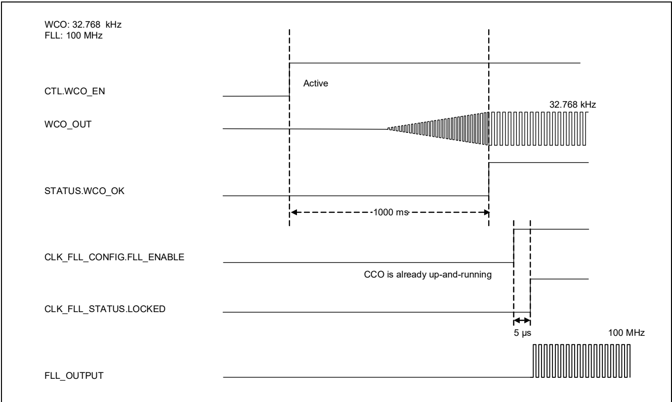
Figure 35 WCO to FLL diagram
