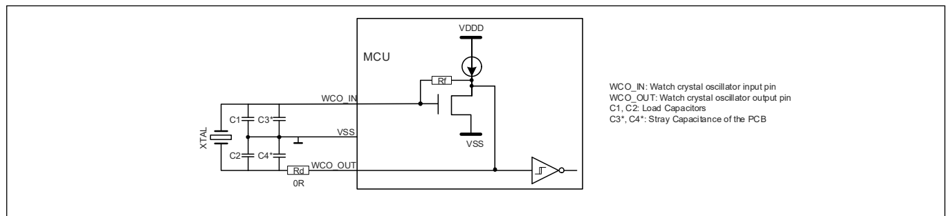
Figure 33 WCO connection scheme [77]
