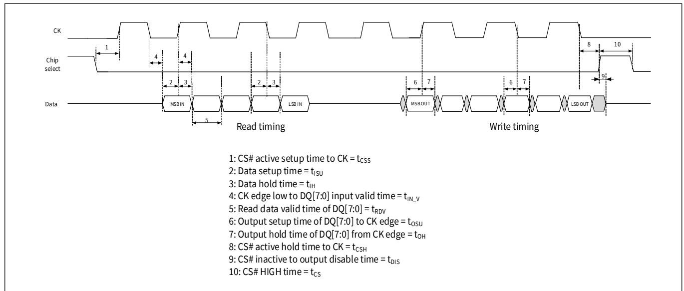
Figure 43 DDR write and read timing diagram
