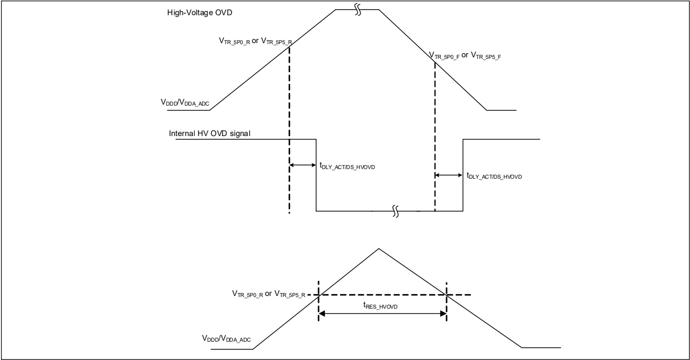
Figure 27 High-voltage OVD specifications
