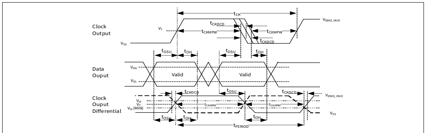
Figure 39 xSPI master data output timing reference level (JEDEC)
