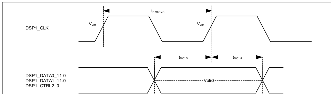
Figure 44 TTL display out timing
