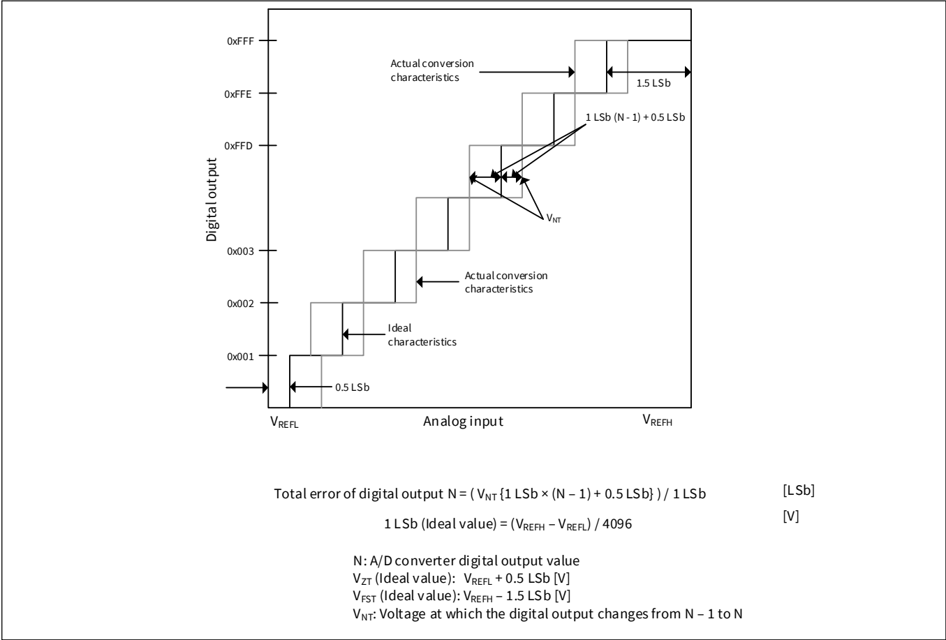
Figure 13 ADC characteristics and error descriptions
