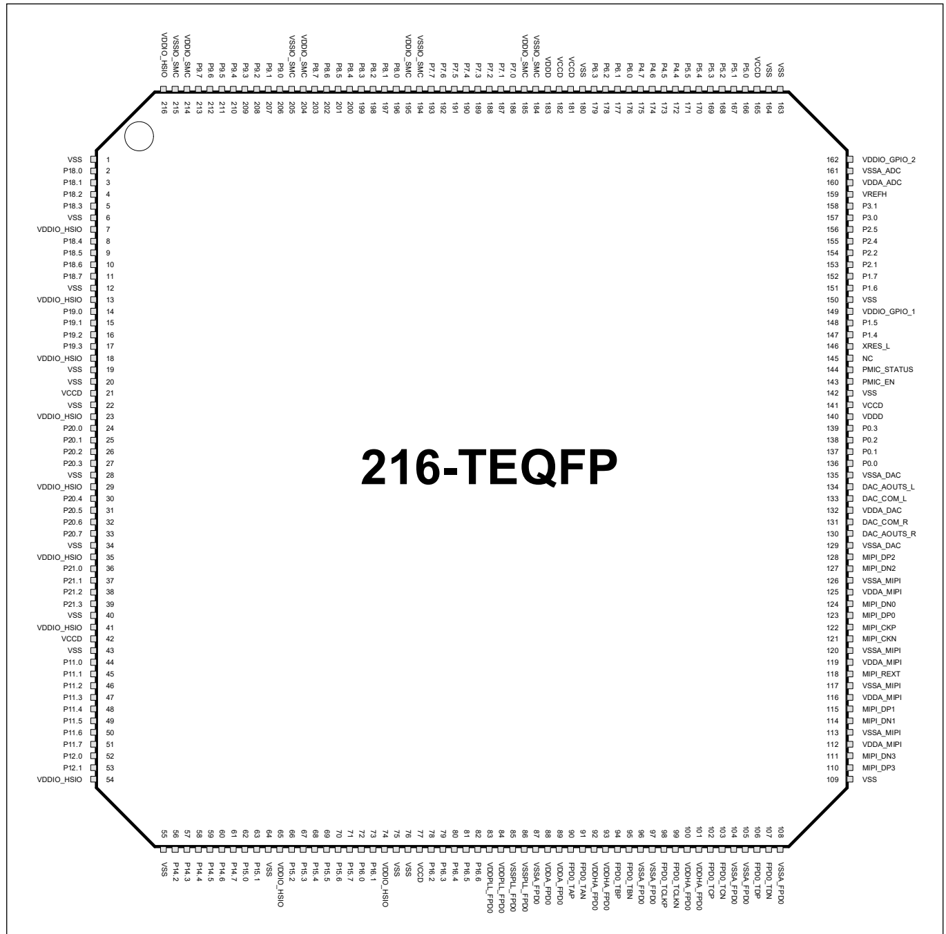
Figure 5 216-TEQFP pin assignment [22]
