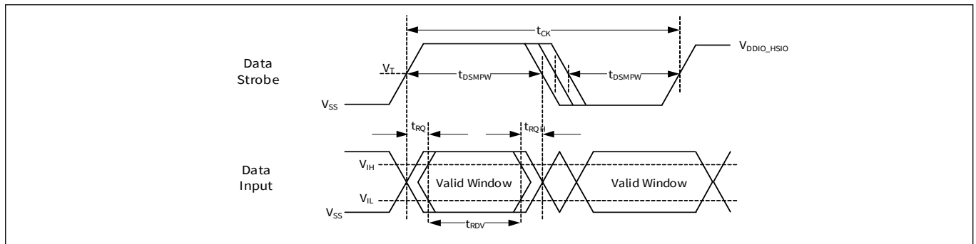
Figure 38 xSPI master data input timing reference level (JEDEC)
