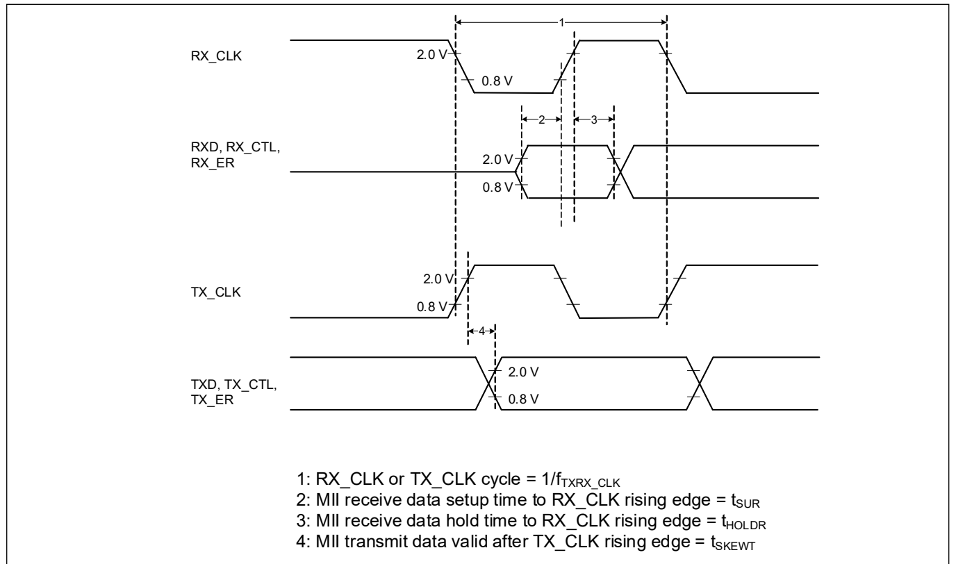
Figure 34 MII timing diagram
