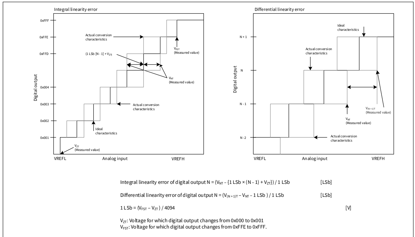
Figure 14 Integral and differential linearity errors
