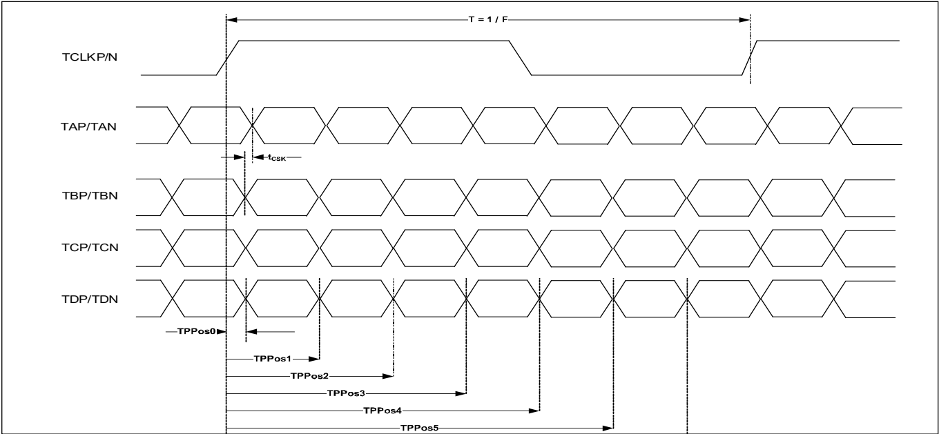
Figure 46 FPD-link output pulse position error and channel-to-channel skew
