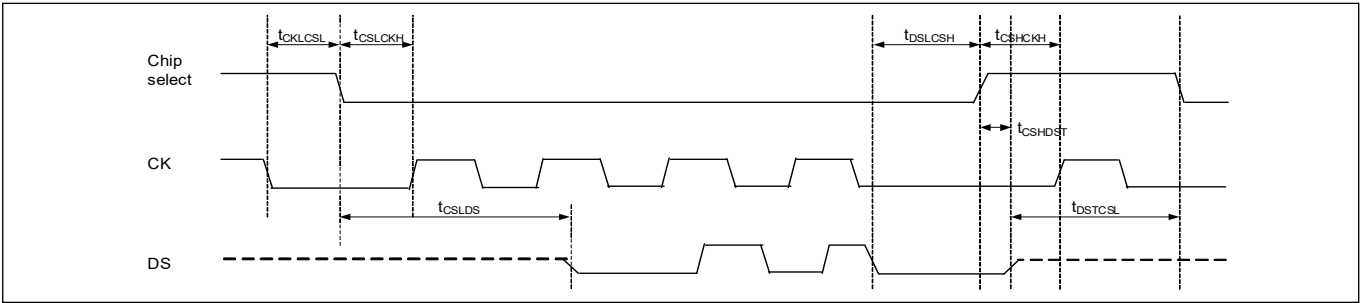
Figure 41 xSPI data strobe to chip select timing diagram
