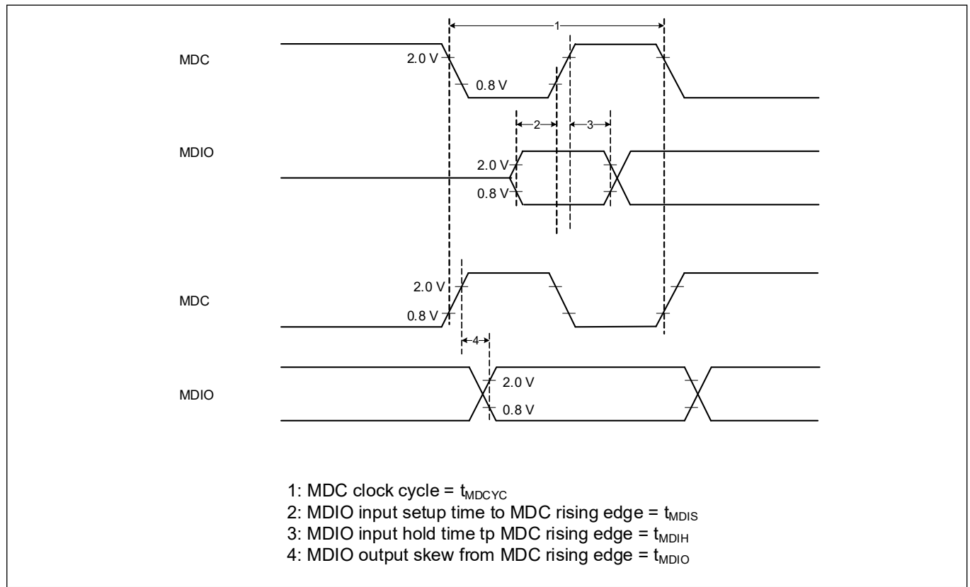
Figure 35 MDIO timing diagram
