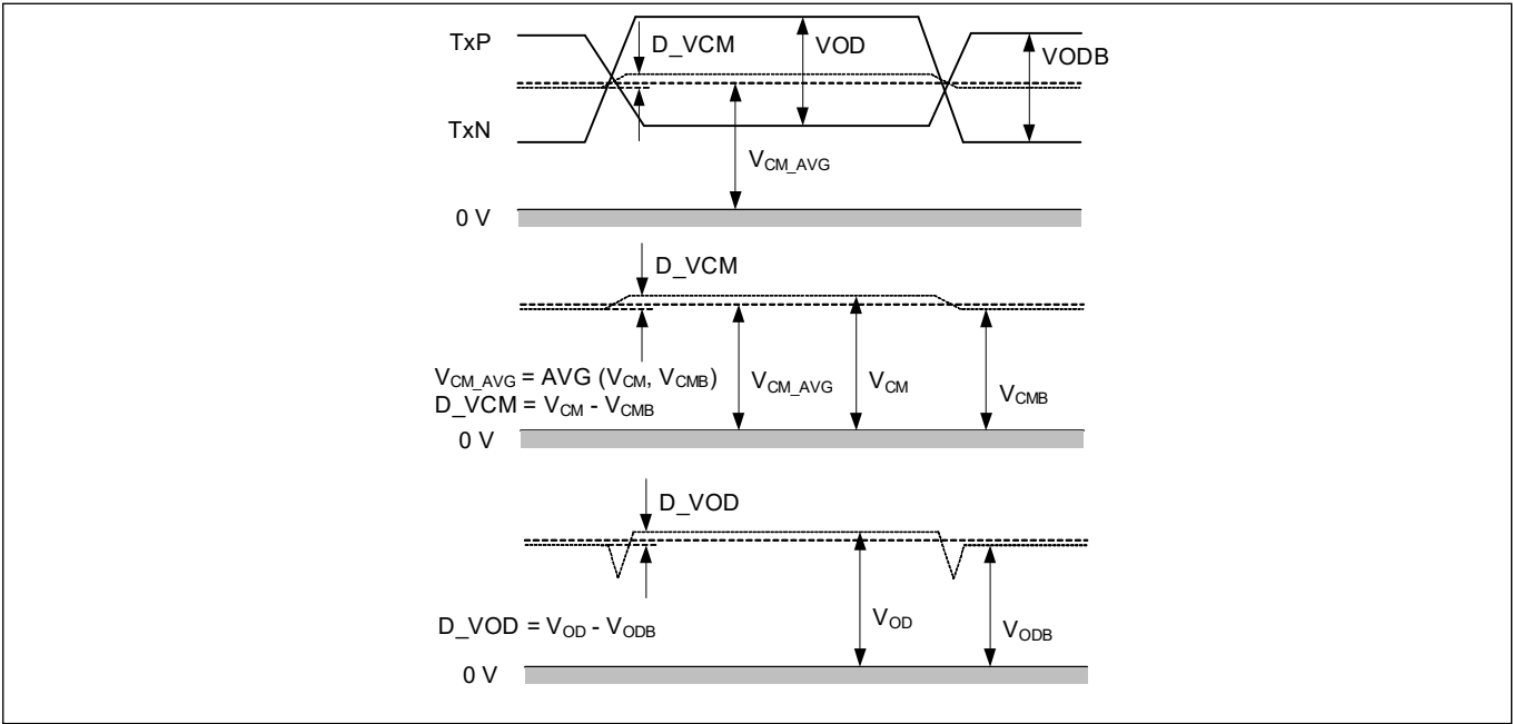
Figure 47 Skew between TxP and TxN, and steady-state differential amplitude and common-mode voltages
