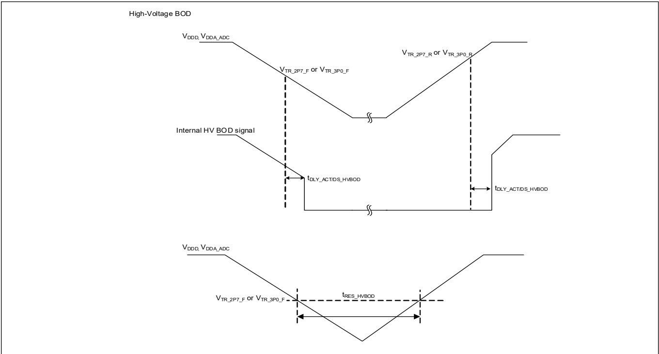
Figure 25 High-voltage BOD specifications
