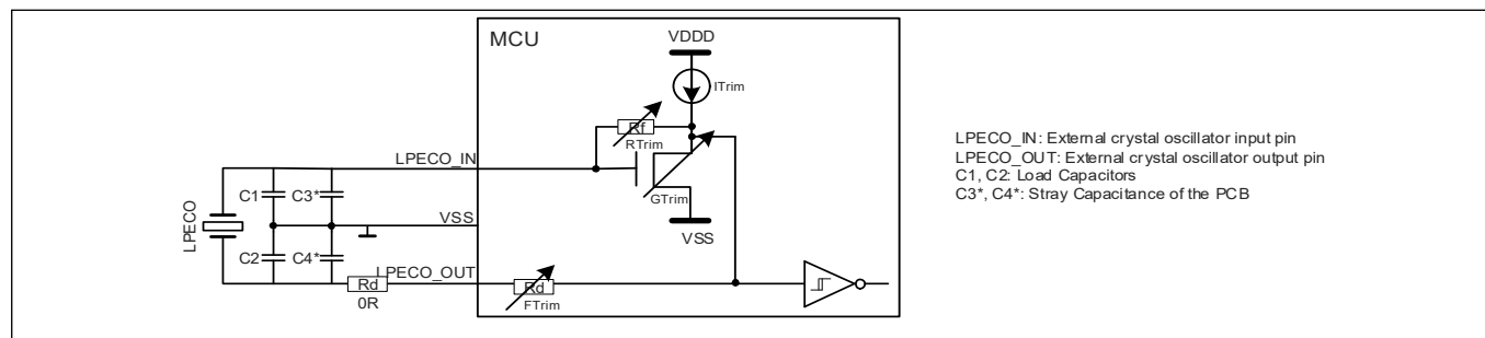
Figure 31 LPECO connection scheme [74]
