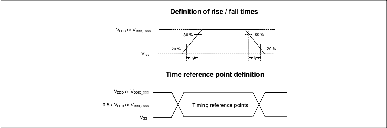
Figure 16 AC timings specifications
