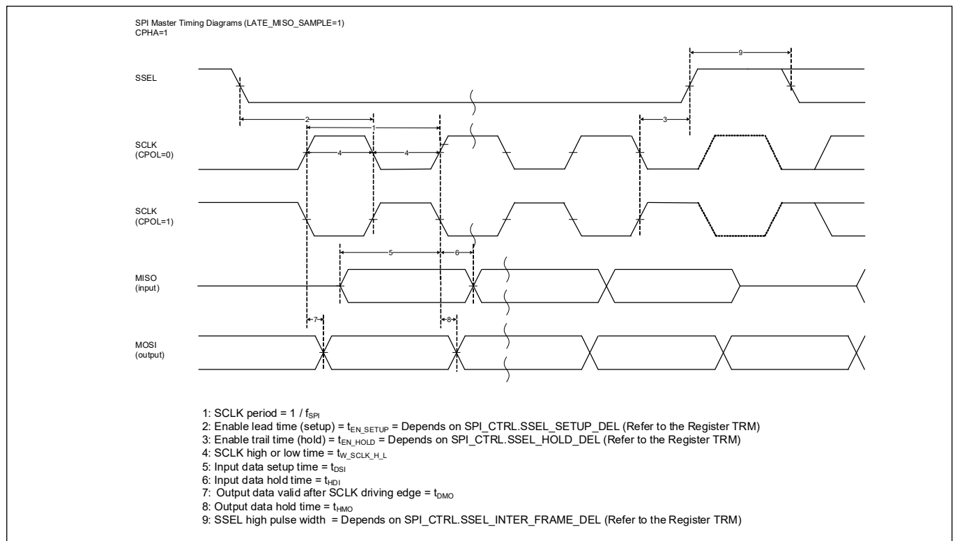
Figure 20 SPI master timing diagrams with HIGH clock phase
