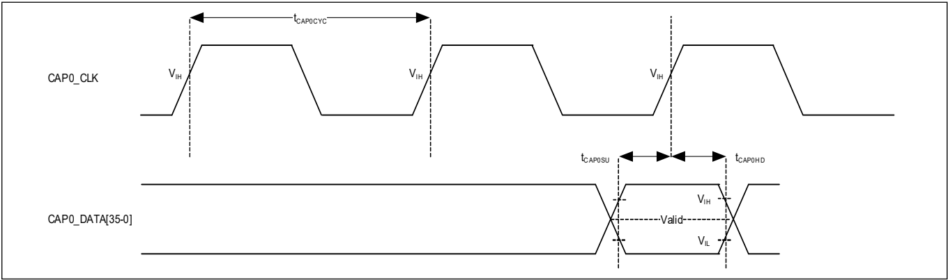
Figure 45 Video capture timing
