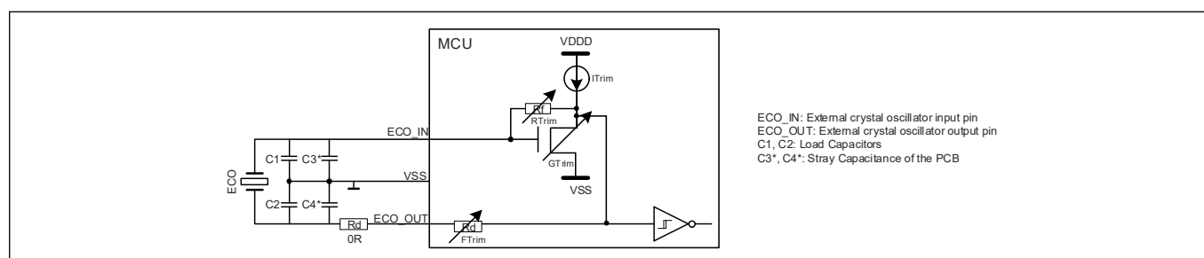
Figure 32 ECO connection scheme [74]
