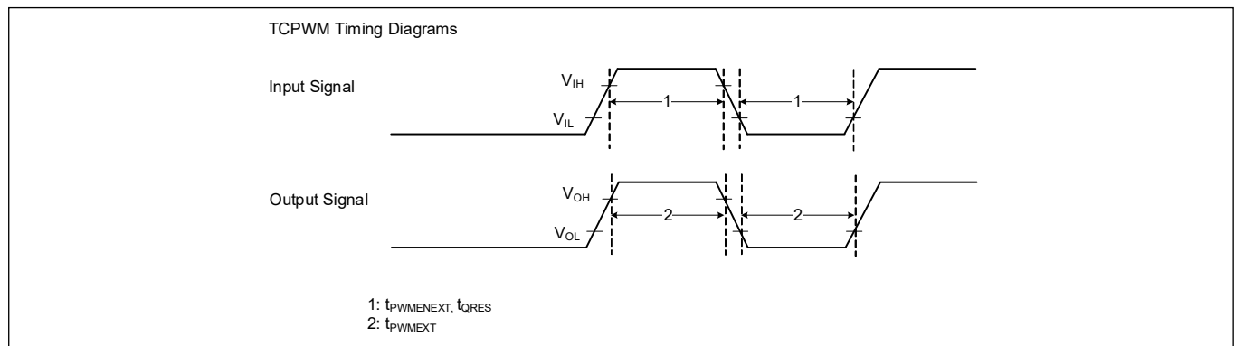
Figure 17 TCPWM timing diagrams
