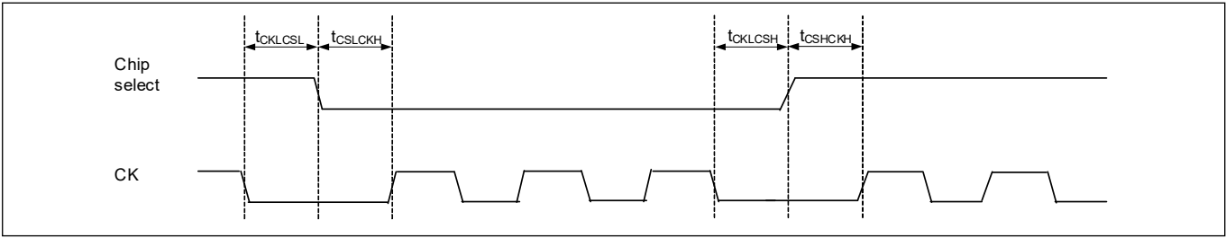
Figure 40 xSPI clock to chip select timing diagram
