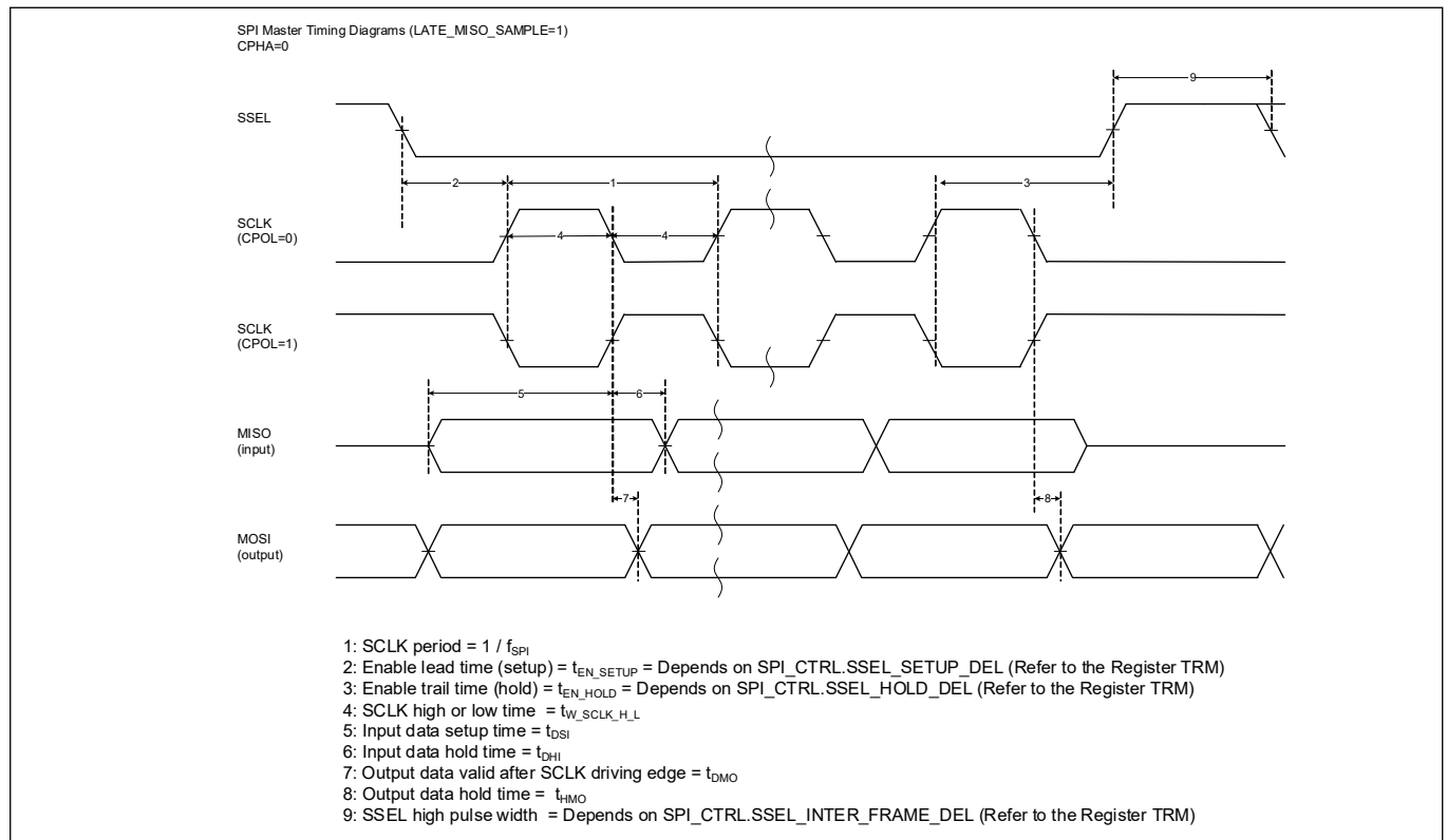
Figure 19 SPI master timing diagrams with LOW clock phase
