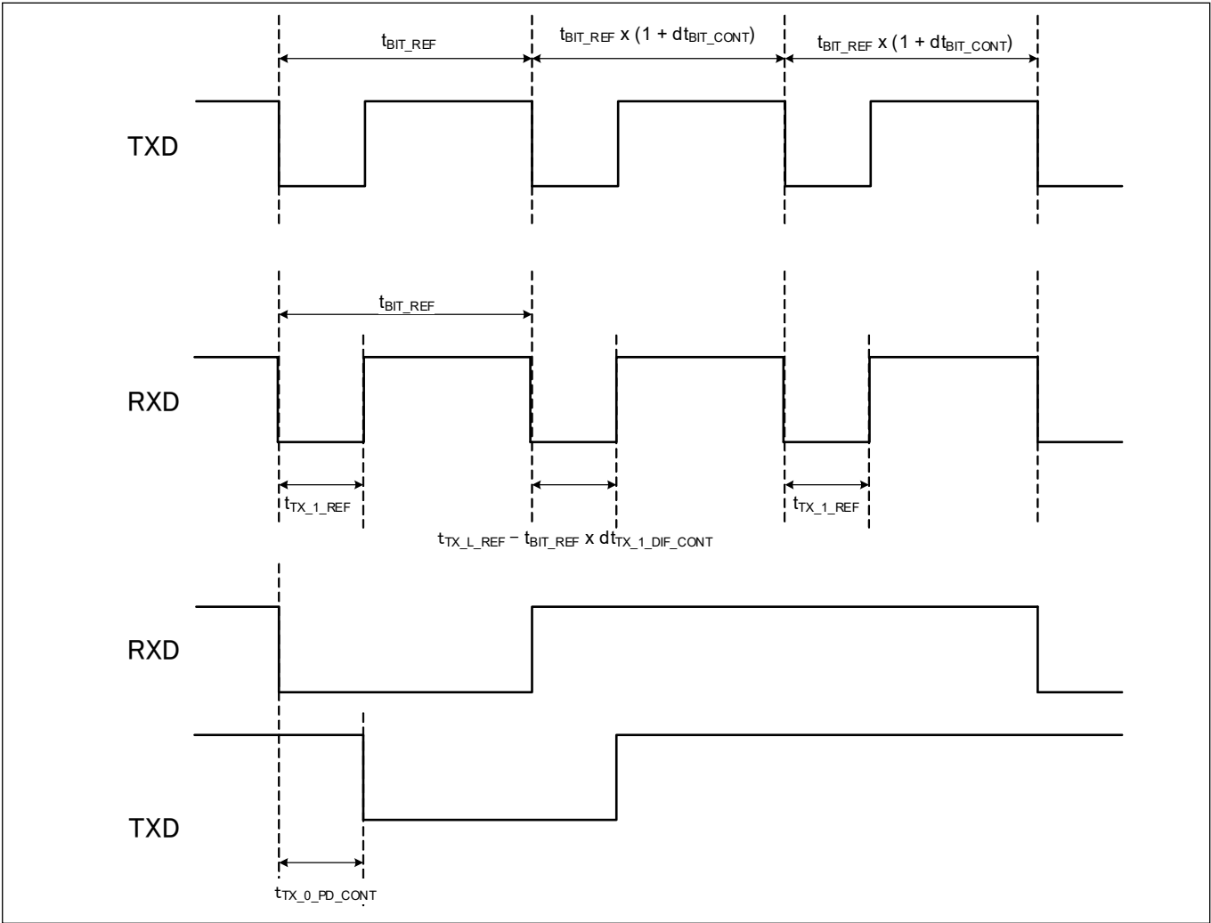
Figure 37 CXPI specifications
