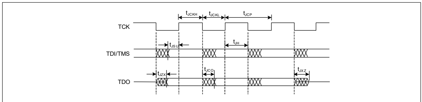
Figure 30 JTAG specifications
