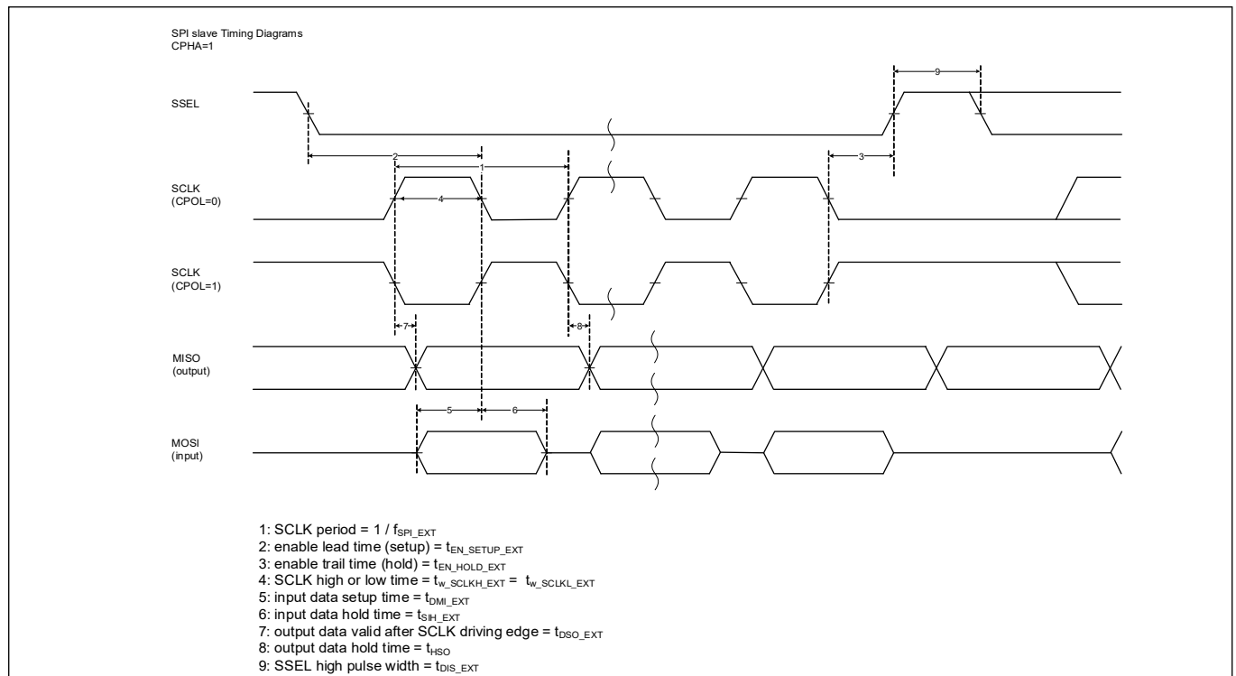
Figure 22 SPI slave timing diagrams with HIGH clock phase
