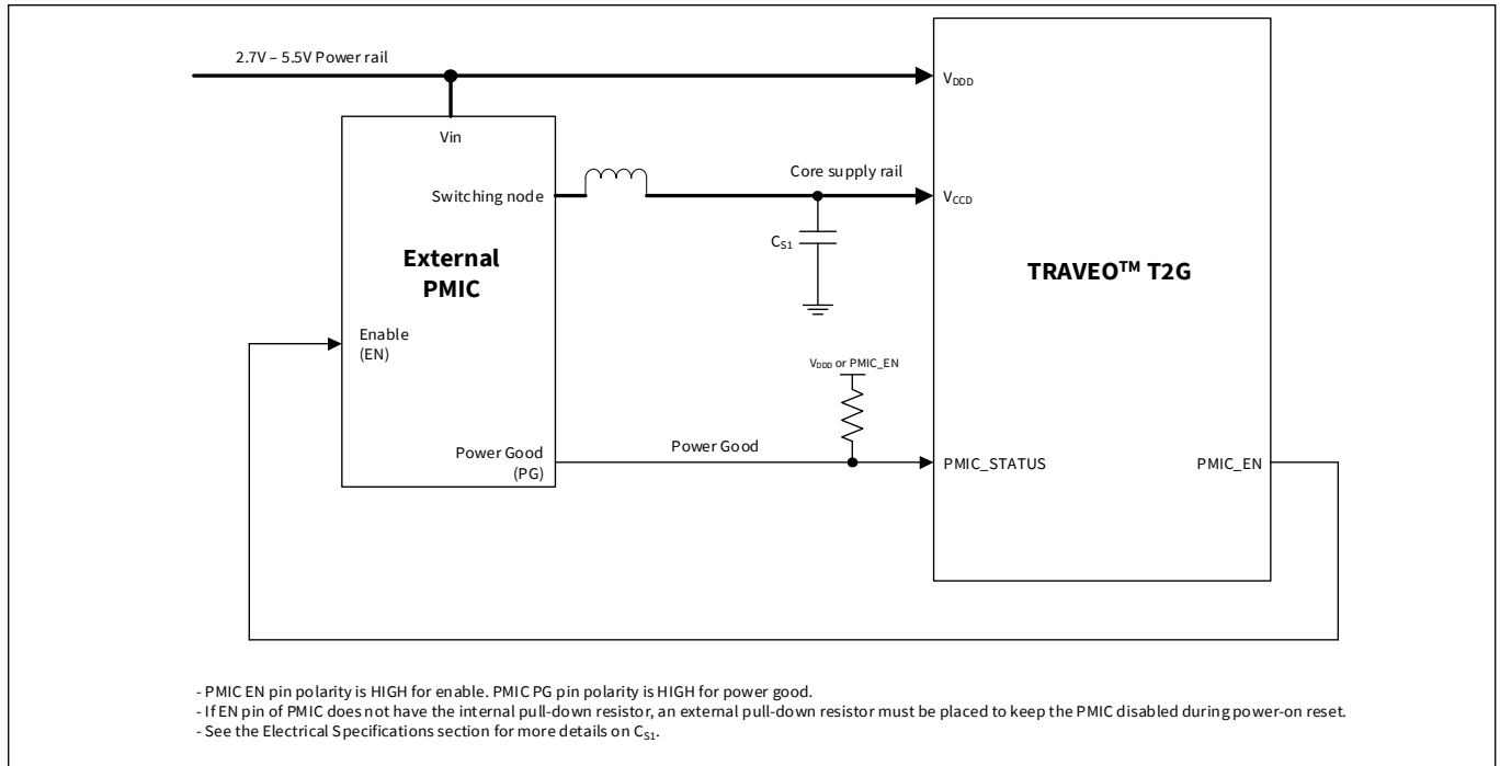
Figure 2 Sample PMIC control interface
