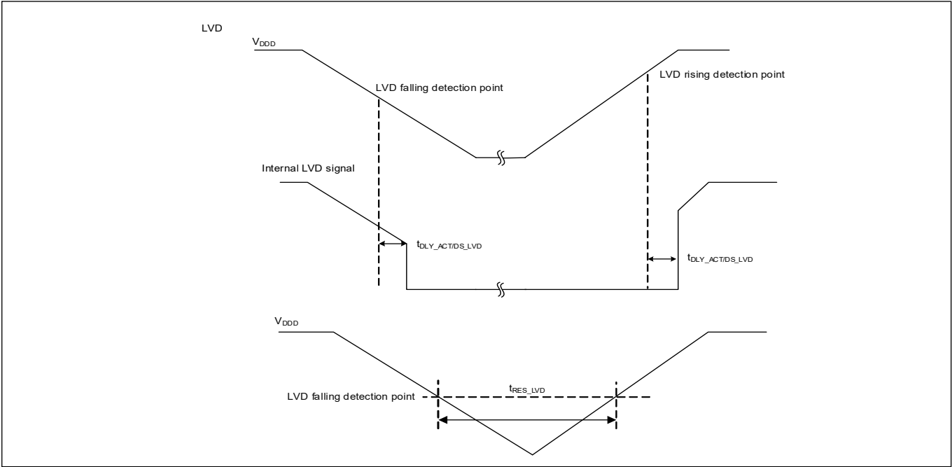
Figure 29 LVD specifications
