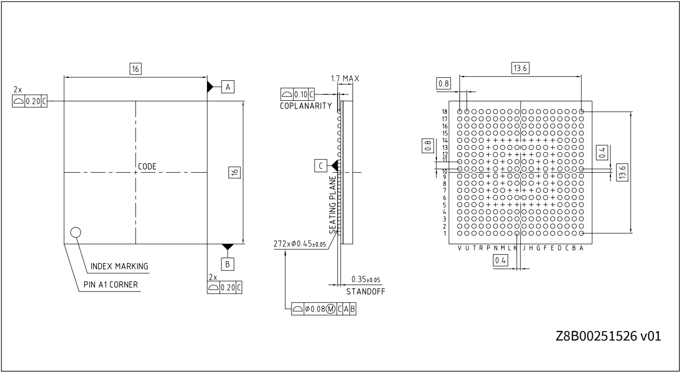
Figure 48 272-ball FBGA package outline (PG-LFBGA-272)
