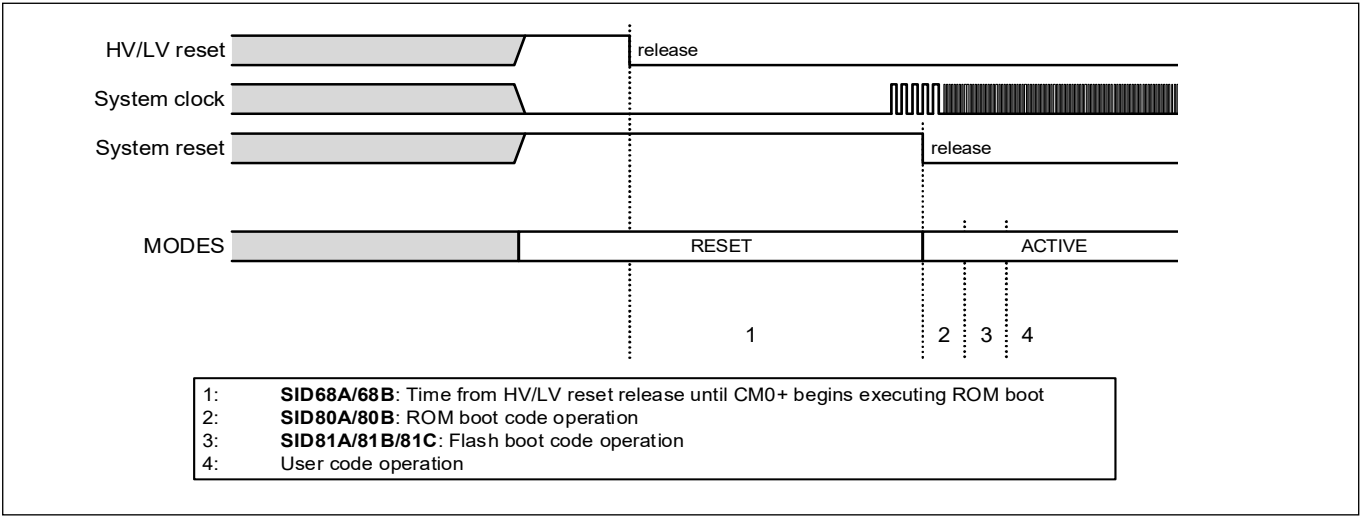
Figure 12 Reset sequence
