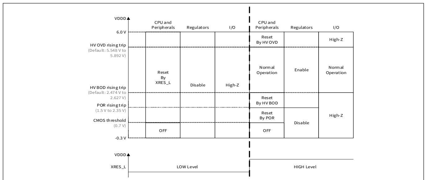
Figure 23 Device operations supply range
