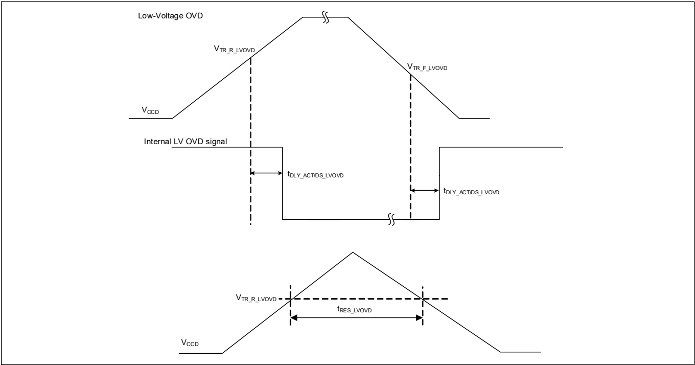
Figure 28 Low-voltage OVD specifications
