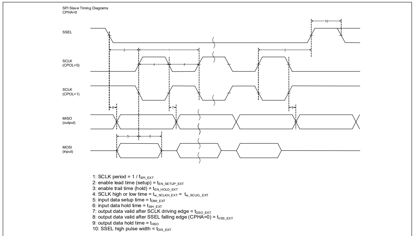
Figure 21 SPI slave timing diagrams with LOW clock phase
