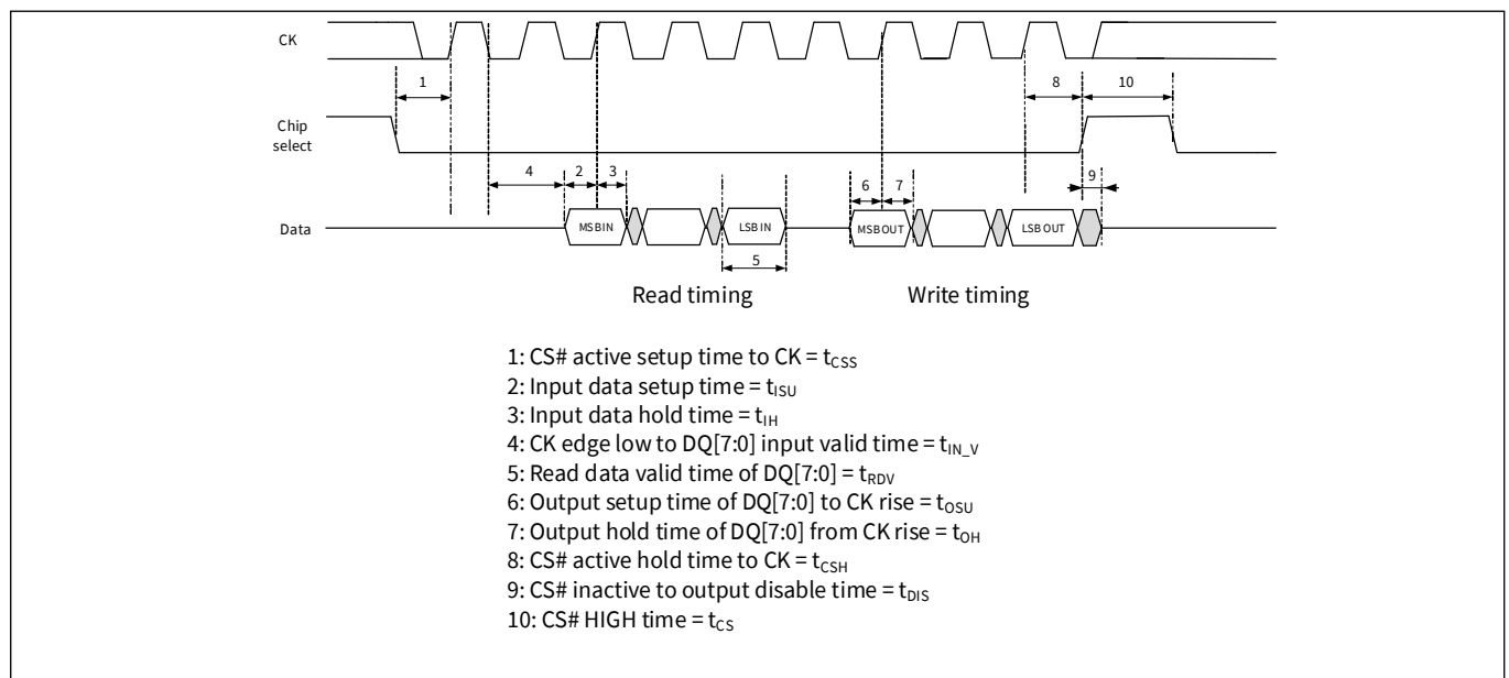
Figure 42 SDR write and read timing diagram
