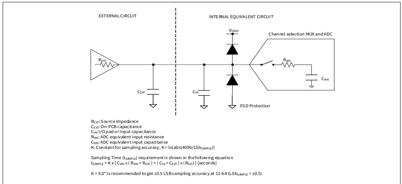
Figure 15 ADC equivalent circuit for analog input
