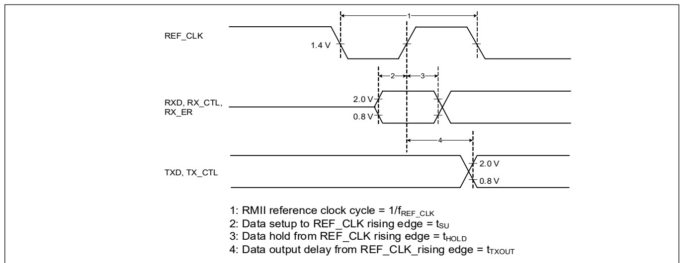
Figure 36 RMII timing diagram
