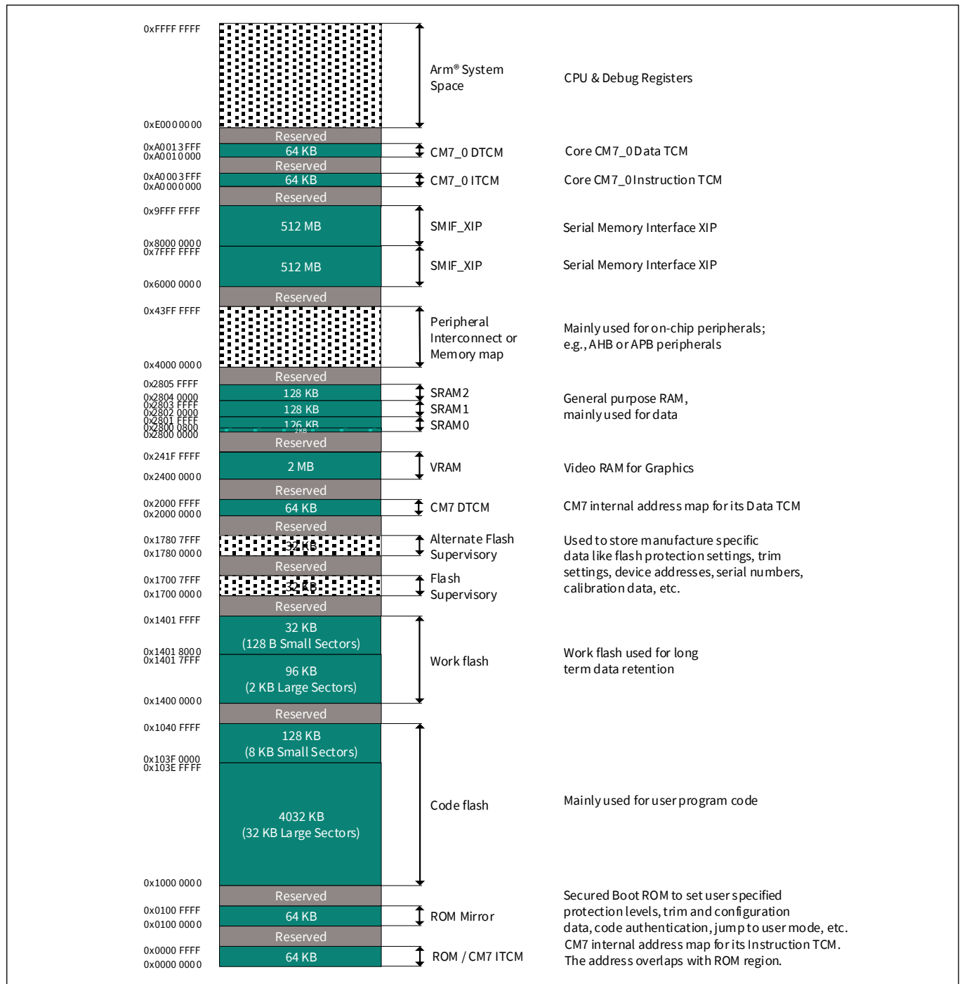
Figure 3 CYT3DL address map [17, 18]
