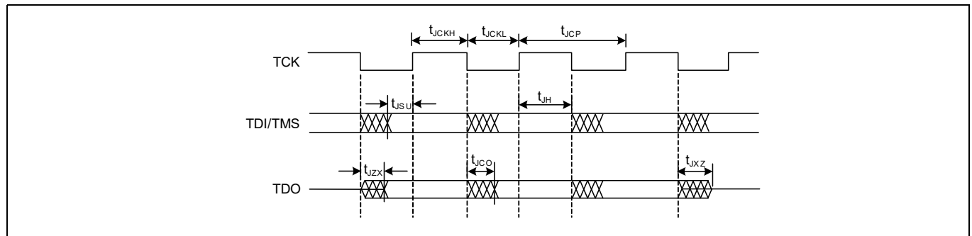
Figure 26-21 JTAG specifications
