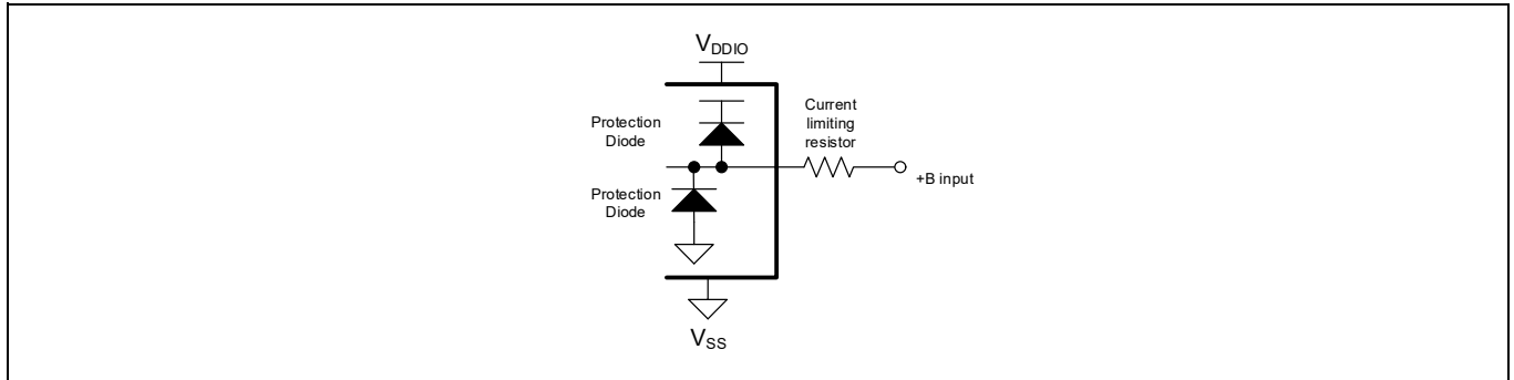
Figure 26-1 Example of a recommended circuit [56]
