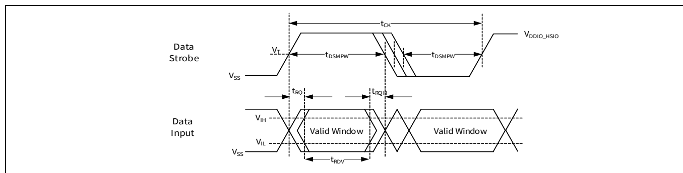
Figure 26-2 xSPI master data input timing reference level (JEDEC)
