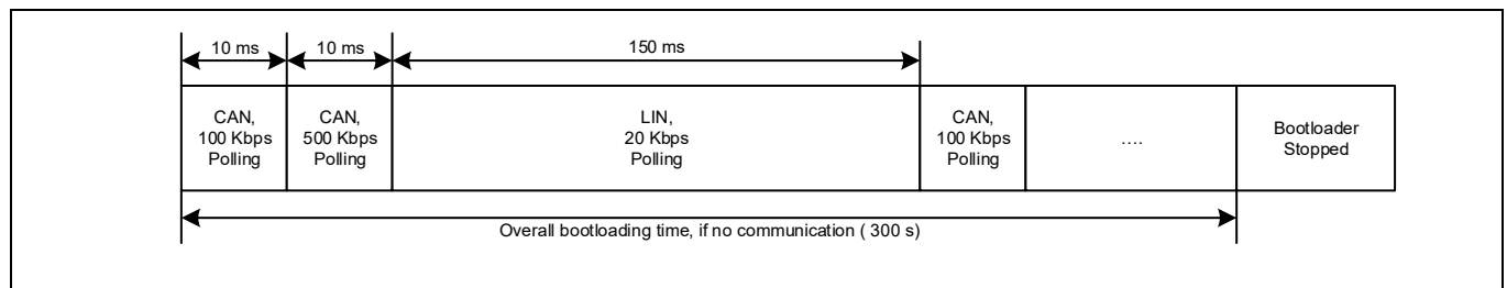
Figure 31-1 Bootloading sequence
