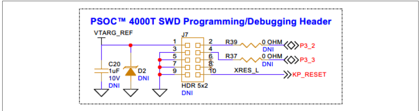
Figure 25 Schematic of the PSOC™ 4000T device 10-pin programming/debugging header
