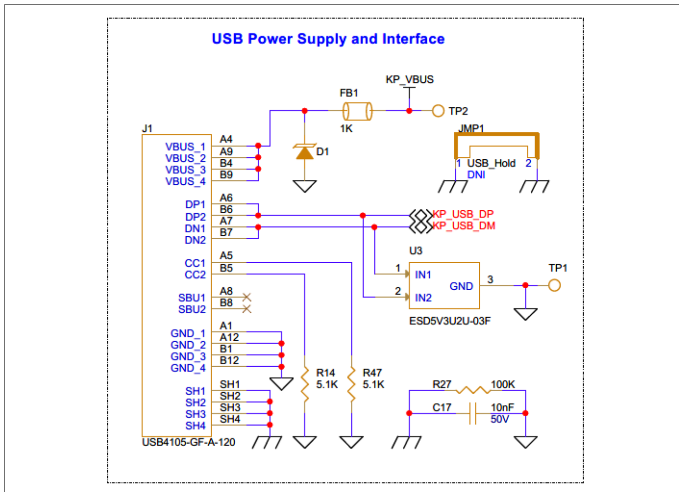
Figure 32 Schematic of the USB Type-C connector (J1) and ESD protection (D1, U3)
