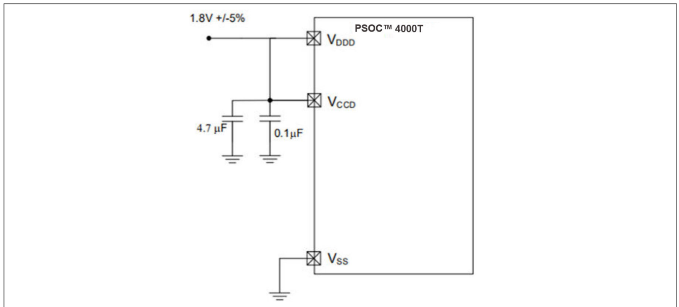
Figure 20 PSOC™ 4000T device schematic with 1.8 V \pm 5% external supply
