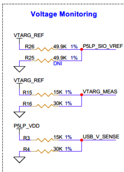
Figure 29 Schematic of KitProg3 on board target voltage monitoring circuit
