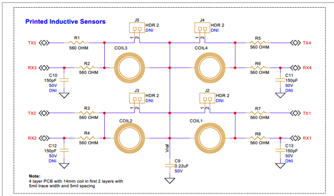
Figure 44 Inductive sensors schematic
