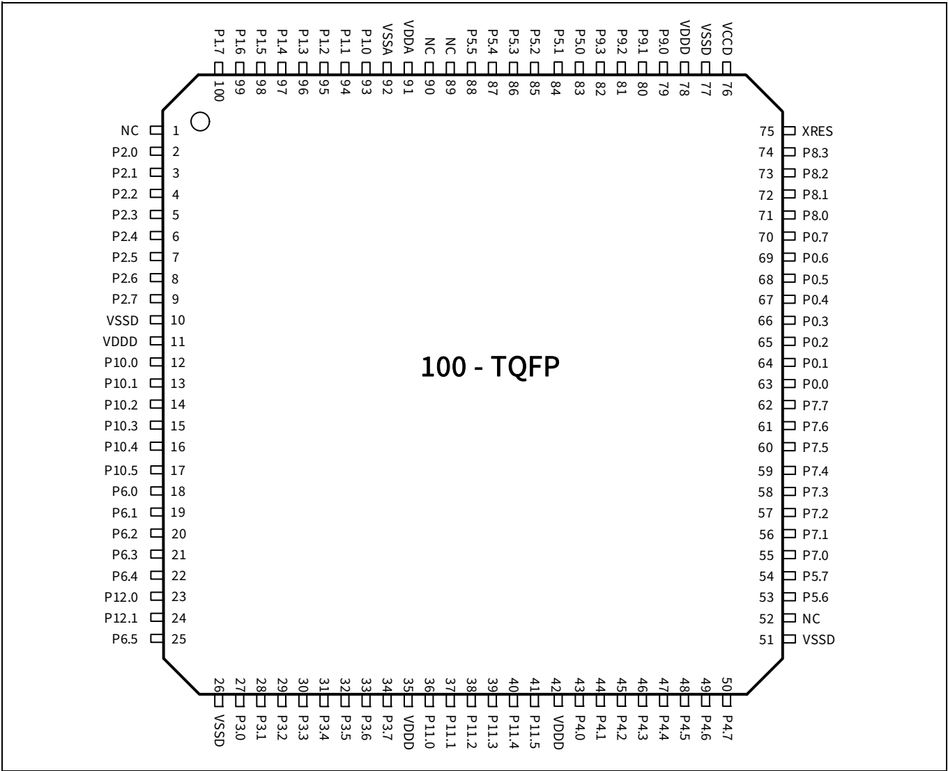
Figure 4 100-TQFP
