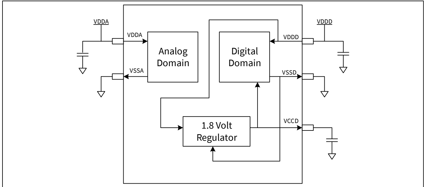
Figure 7 Power supply connections
