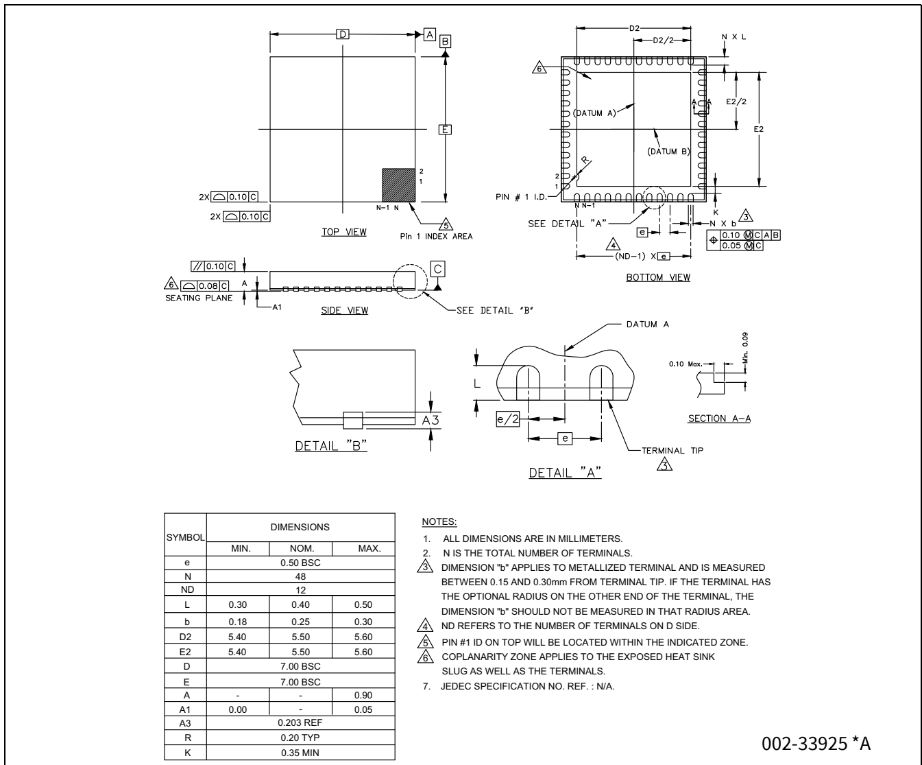
Figure 11 48-pin QFN (7 × 7 × 0.9 mm) package outline, 002-33925
