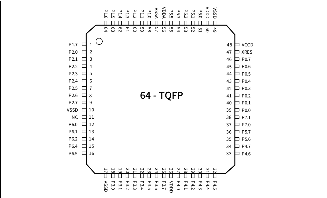
Figure 5 64-TQFP
