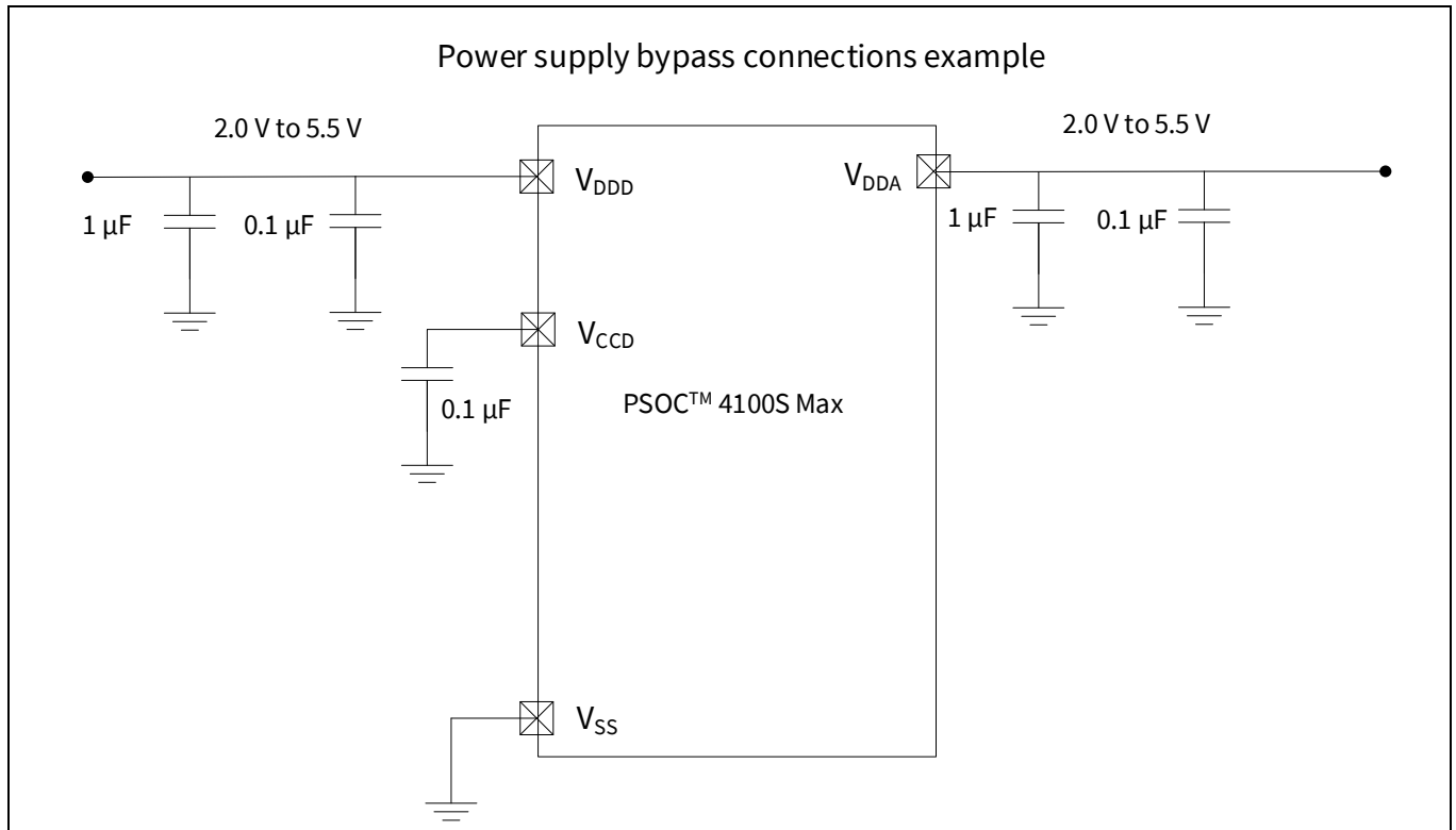
Figure 8 External supply range from 2.0 V to 5.5 V with internal regulator active
