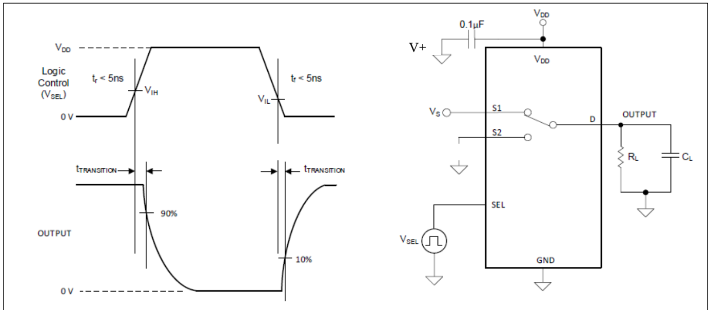
Figure 2. Transition Time
