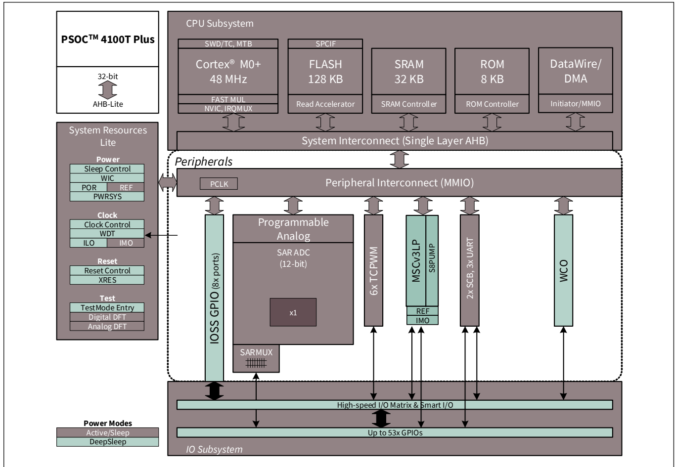
Figure 2 Block diagram
