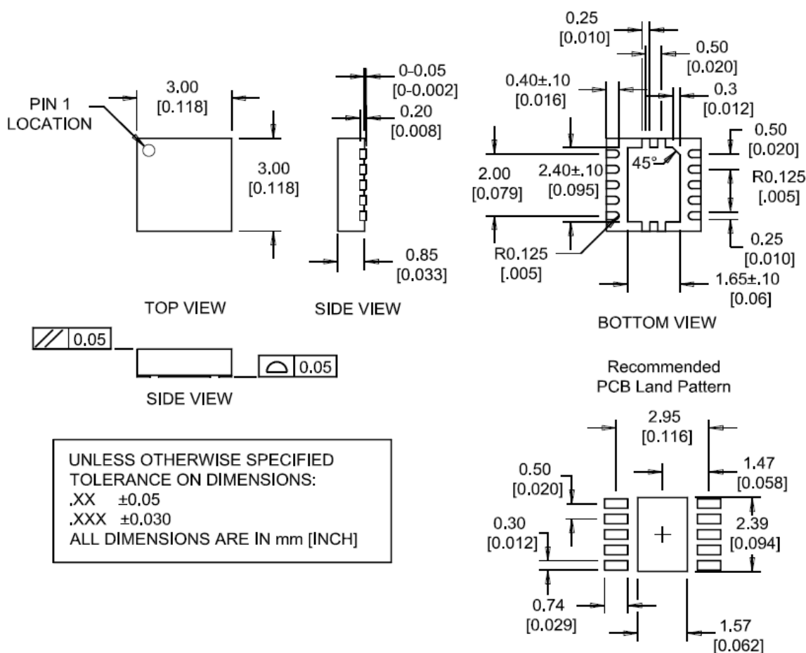
Figure 9: Package Dimensions
