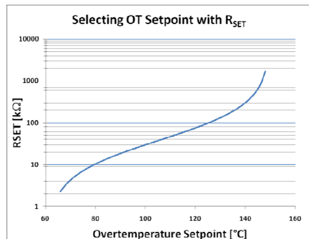
Figure 8: Choosing Overttemperature using R_{SET}
