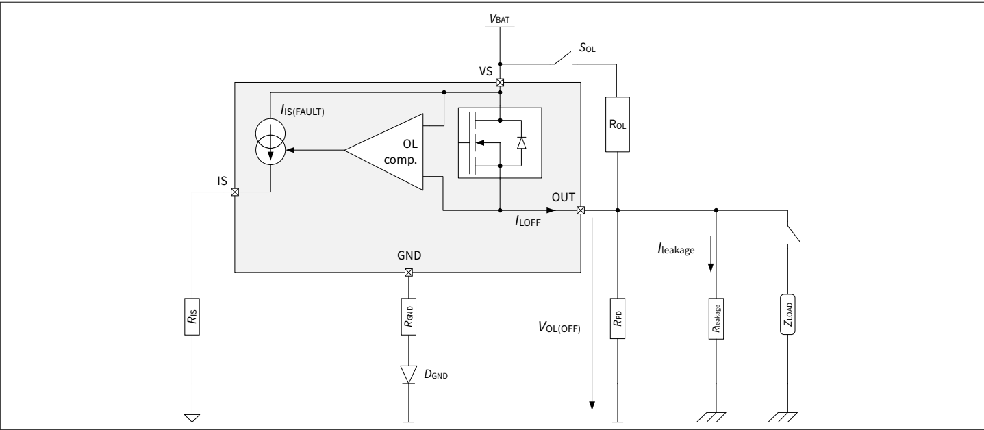
Figure 26 Open Load Detection in OFF Electrical Equivalent Circuit
