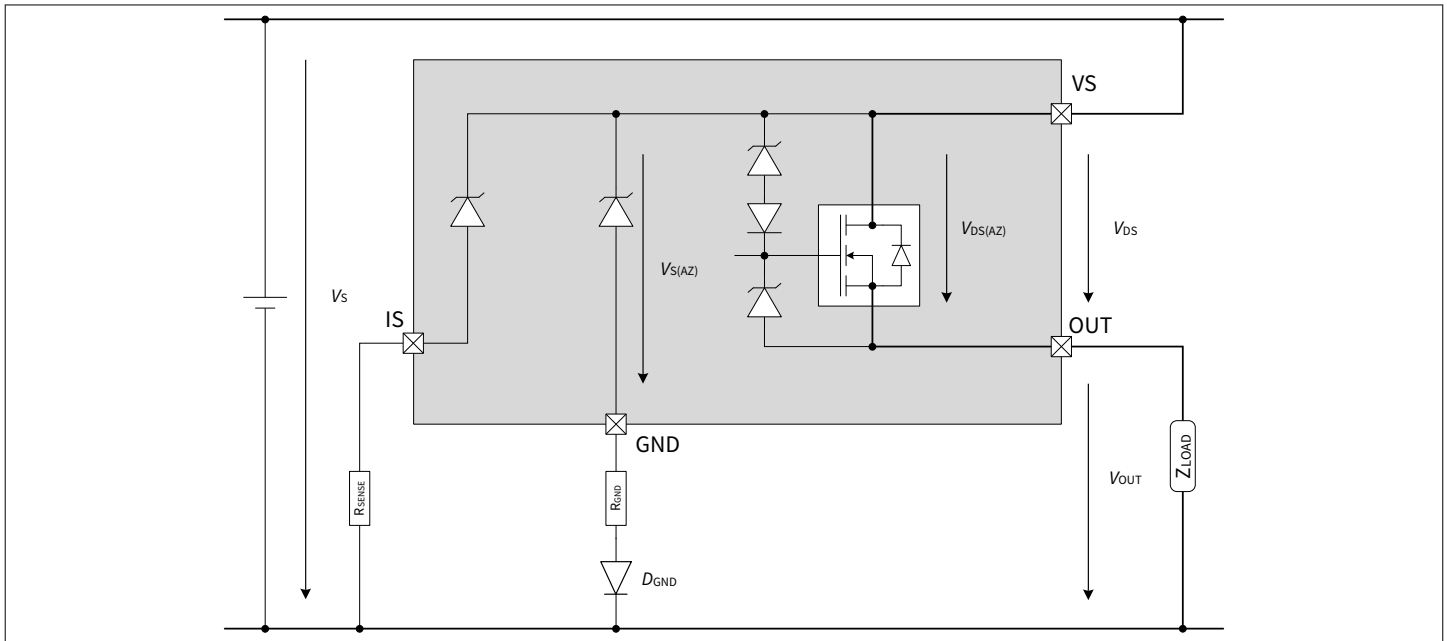
Figure 11 Output Clamp
