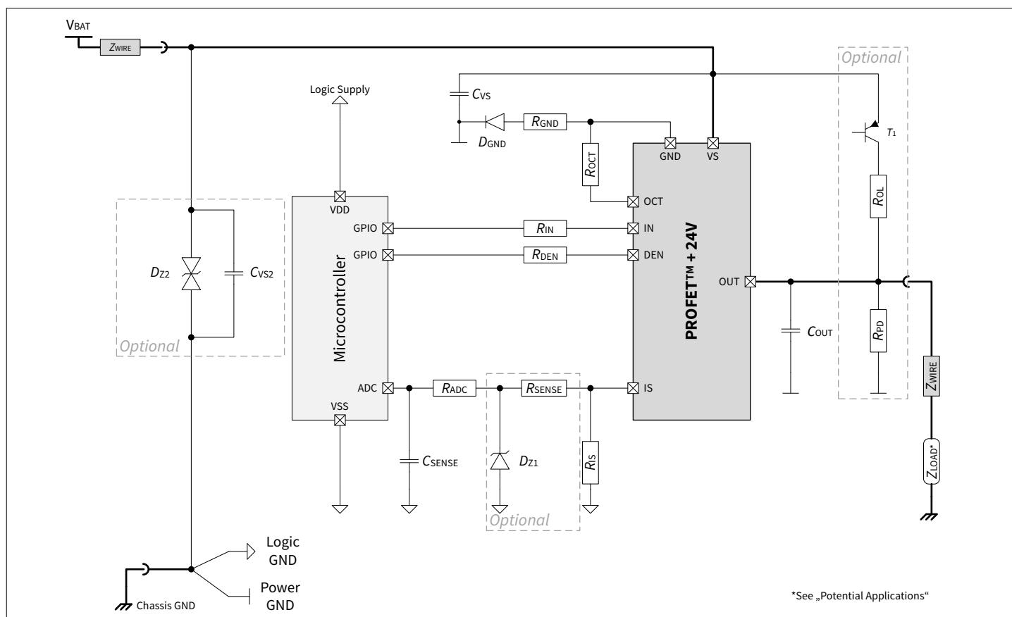
Figure 31 Application Diagram with BTT6035-1ERL
