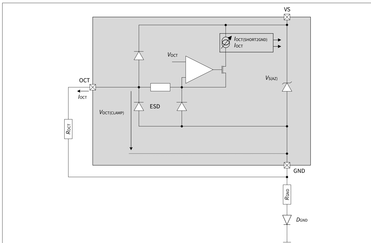
Figure 30 Overcurrent pin circuit
