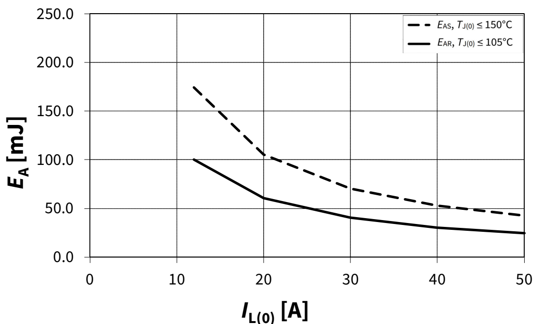
Figure 6 Maximum energy dissipation for inductive switch off, E_{AS/AR} vs. I_L
