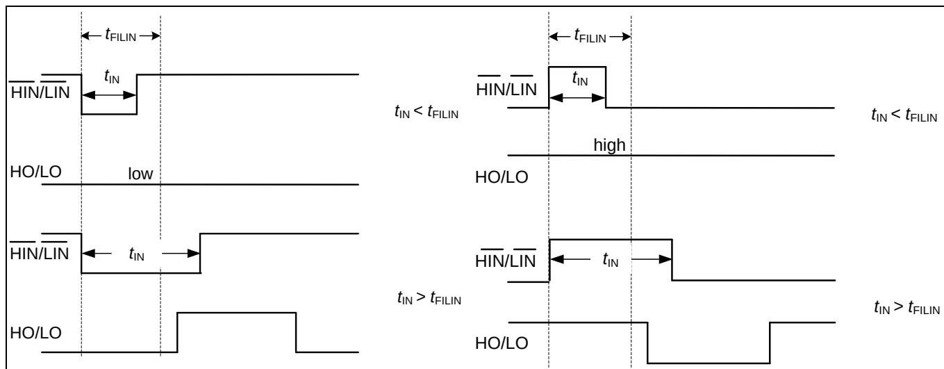
Figure 9 Timing of short pulse suppression (6EDL04I065NT)
