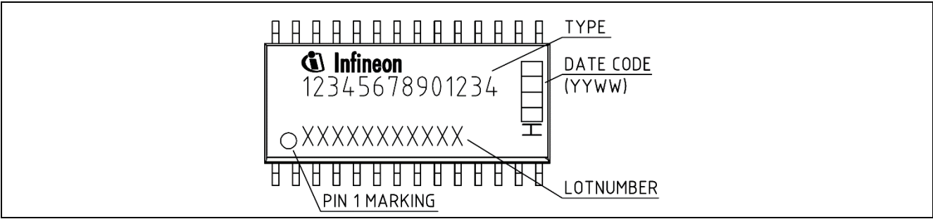
Figure 20 Package drawing
