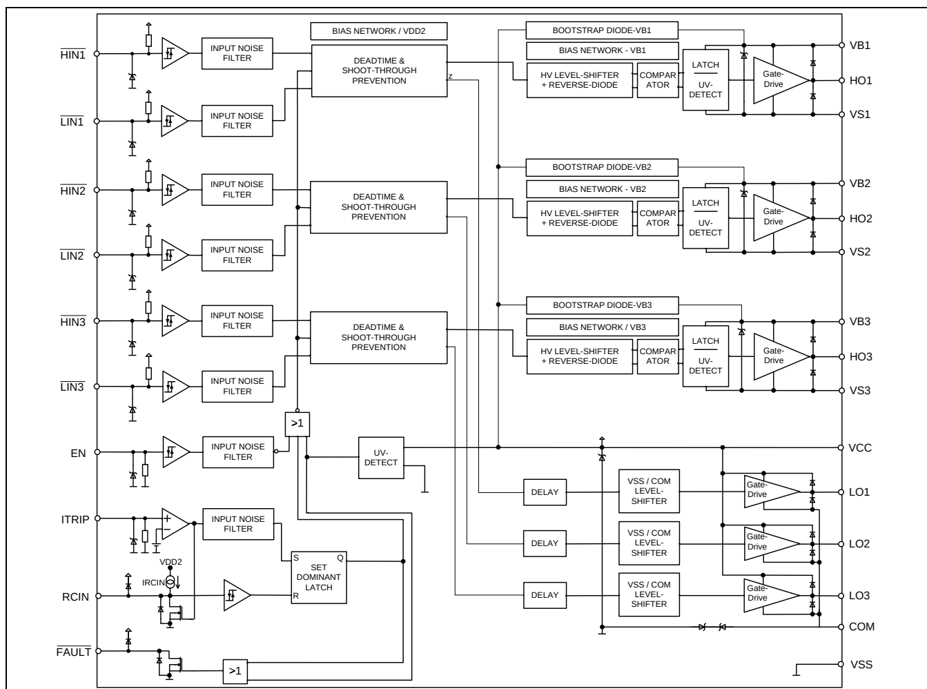
Figure 2 Functional block diagram for 6EDL04I065NR
