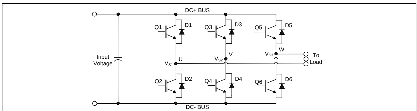
Figure 20 Three-phase inverter
