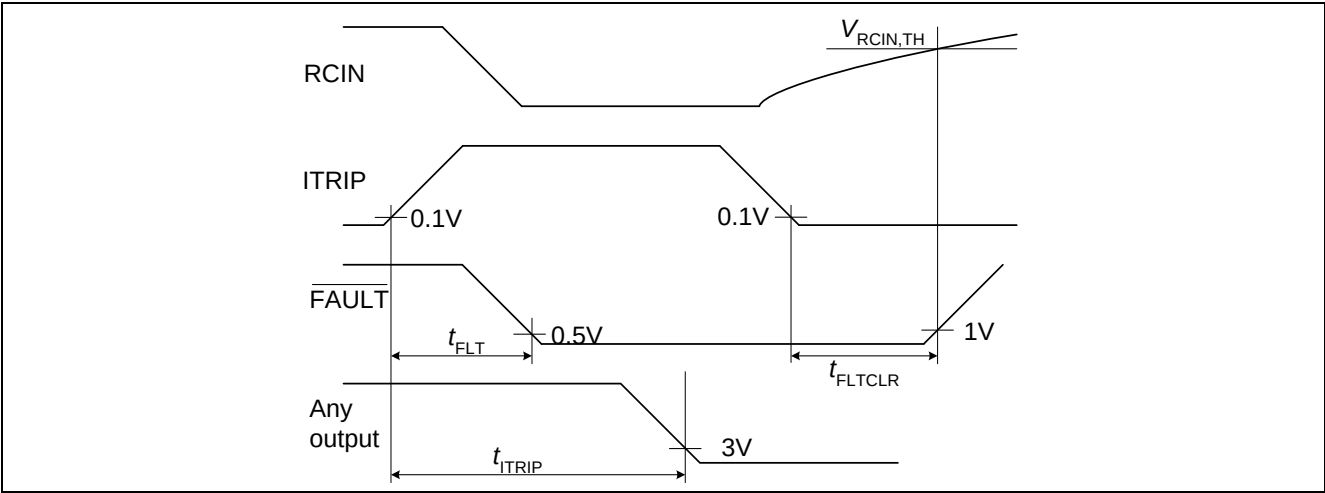
Figure 32 ITRIP timing
