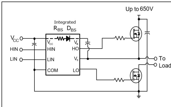
Figure 17 6EDL04 with integrated components
