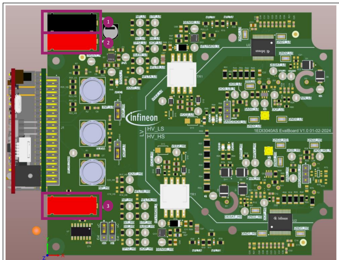
Figure 2 Connectors
