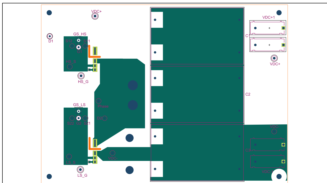
Figure 26 Bottom layer
