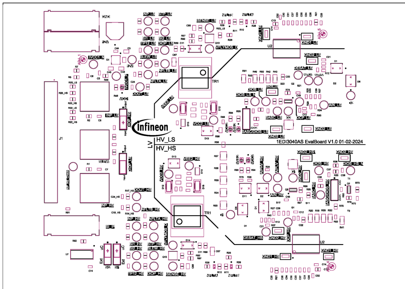
Figure 19 Top assembly
