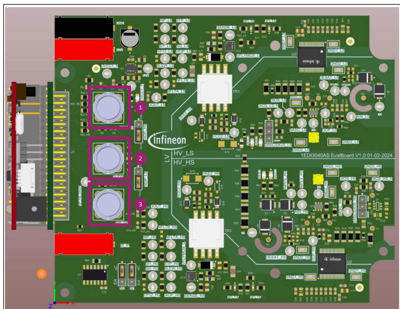
Figure 4 BNC connectors
