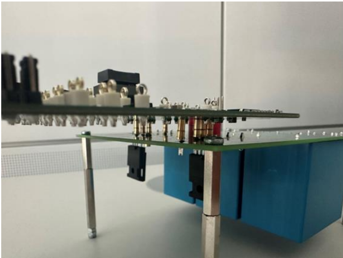
Figure 28 Connection to 1EDI3040AS TO247-4 adapter board
