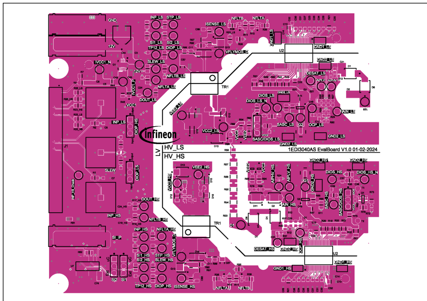
Figure 15 Top layer
