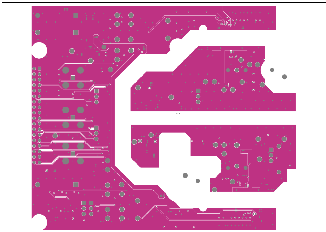
Figure 16 Layer 2
