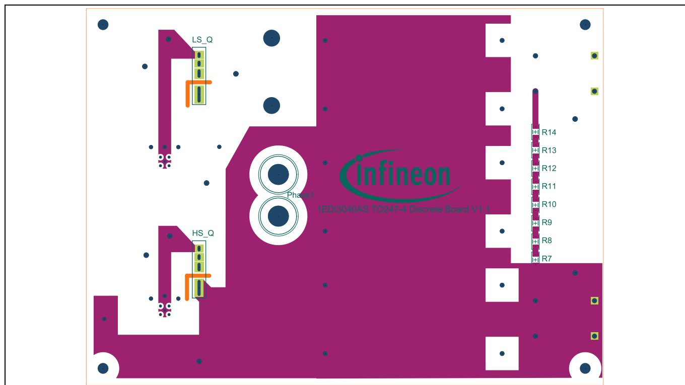
Figure 25 Top layer
