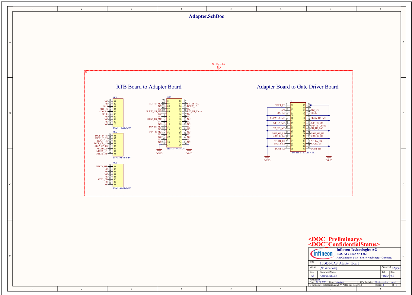
Figure 14 Adapter board schematic
