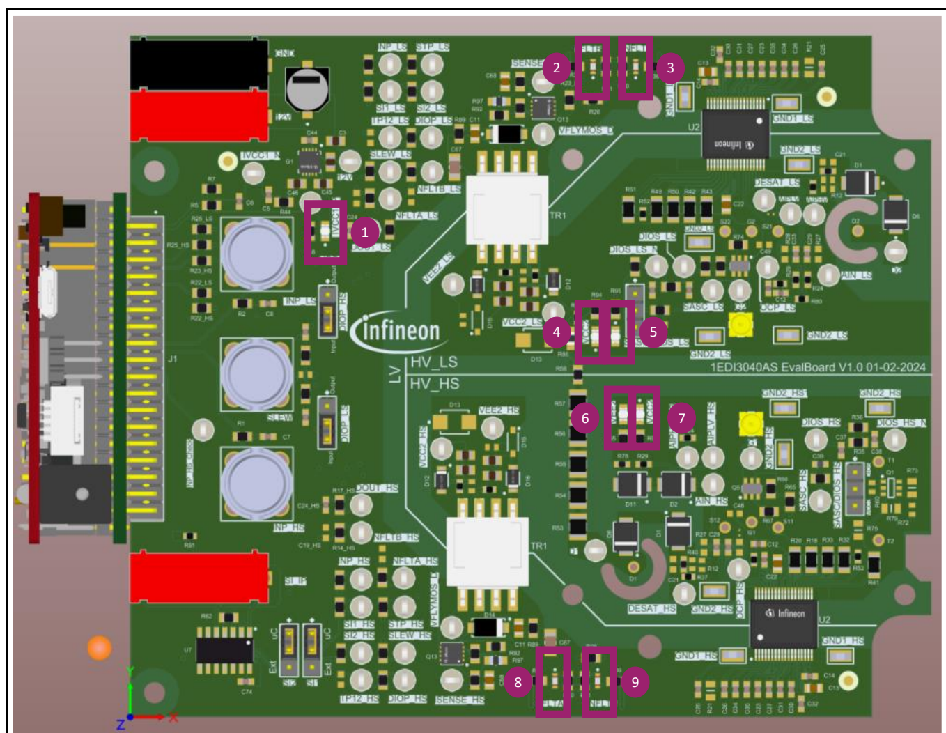
Figure 3 LED indicators
