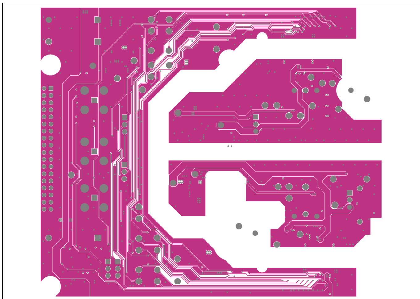
Figure 17 Layer 3
