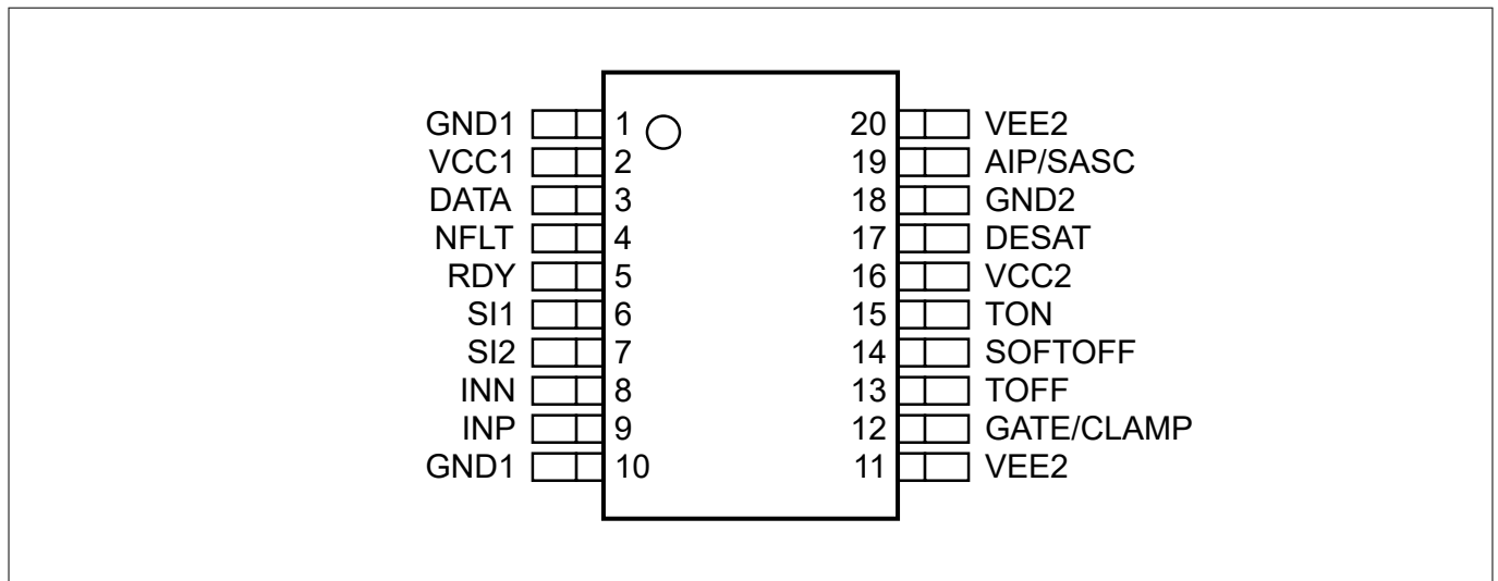
Figure 2 Pin assignment
