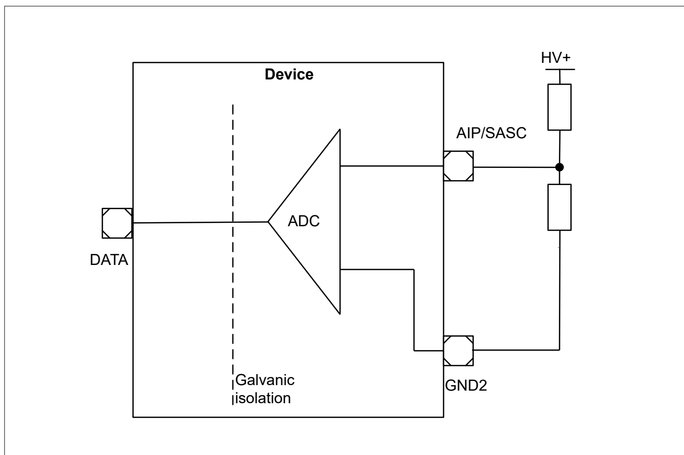
Figure 16 DC-link measurement diagram
