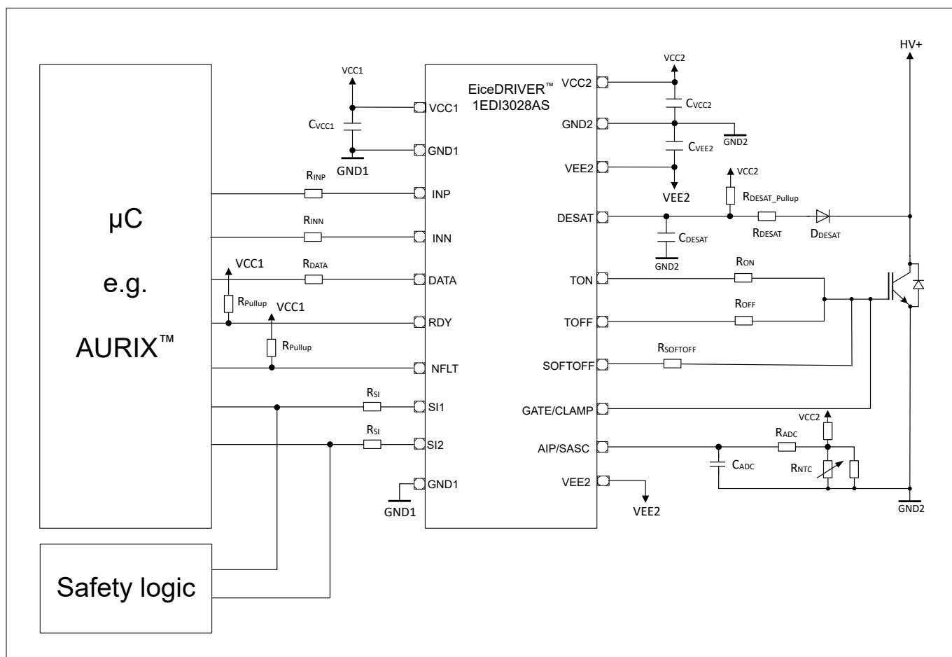
Figure 30 Typical application schematic
