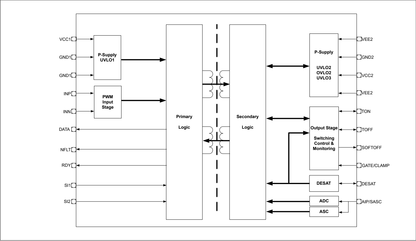
Figure 1 Block diagram
