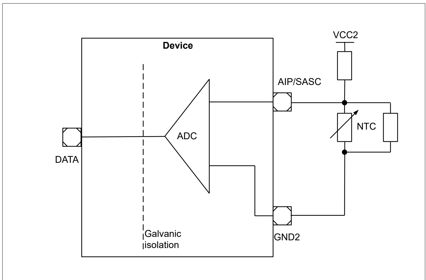
Figure 15 ADC application diagram with NTC.
