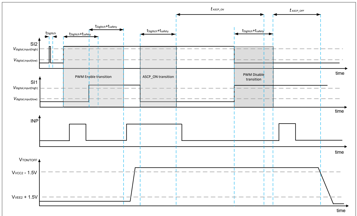
Figure 6 Safety related timing diagram
