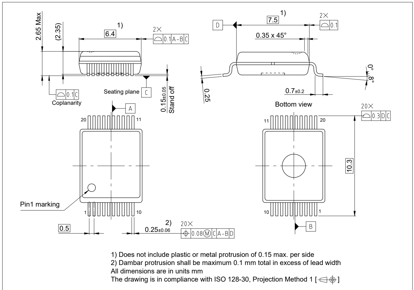
Figure 31 PG-DSO-20
