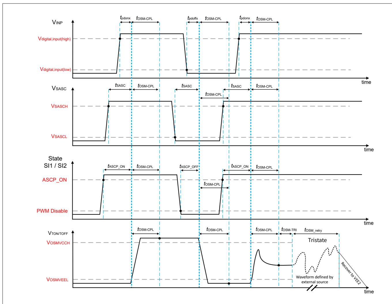
Figure 29 Dynamic output stage monitoring
