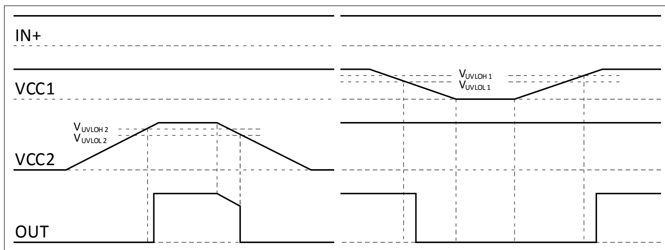
Figure 7 UVLO Behavior
