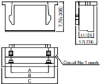
(6 circuits 5.0mm(.197") pitch)
