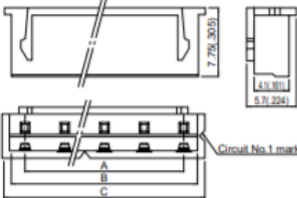
(6 circuits 5.0mm(.197") pitch)
