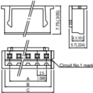
Plugged up (2 circuits 10.0mm(.394") pitch)
