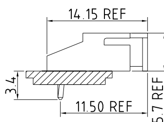
Right Angle Type
