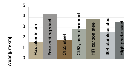
Diagram 05: Wear, rotating with different shaft materials, pressure, p = 1MPa, v = 0.3m/s
