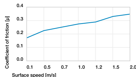
Diagram 04: Coefficient of friction as a function of the surface speed, p = 1\text{MPa}
