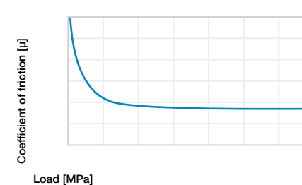
Diagram 05: Coefficient of friction as a function of the pressure, v = 0.01\text{m/s}
