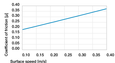
Diagram 04: Coefficient of friction as a function of the surface speed, p = 1\text{MPa}
