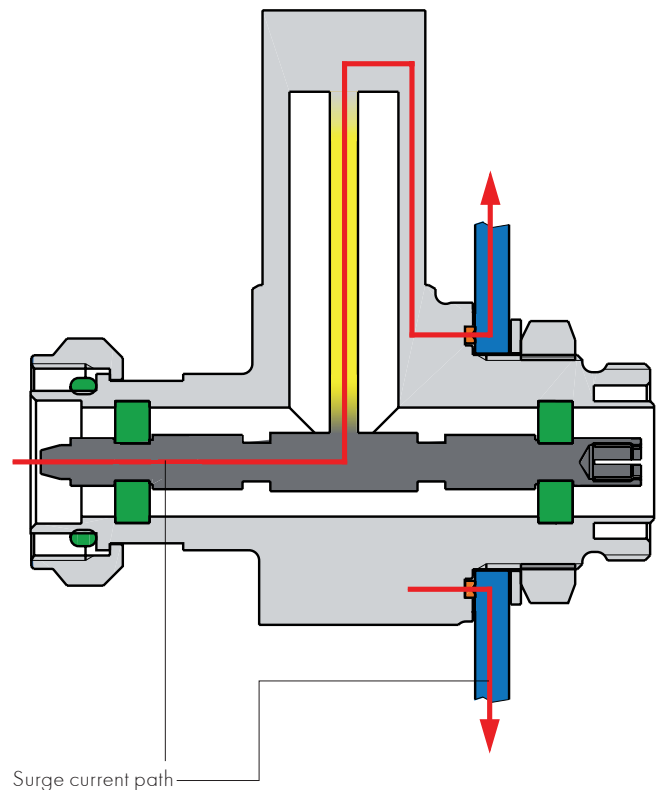
Operating principle of quarter-wave lightning EMP protectors
