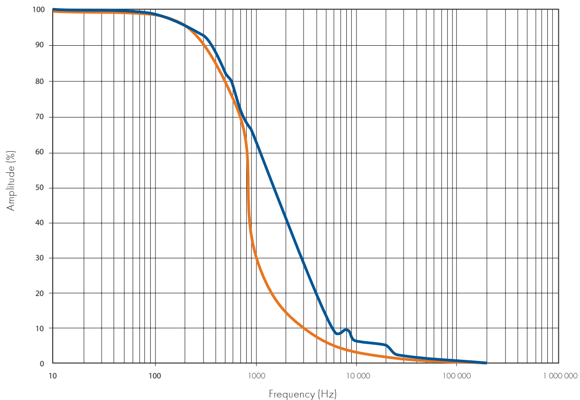
Comparison of the frequency spectra of a genuine lightning current surge (blue – according to K. Berger) and a test current surge 10/350 μs (red – according to IEC 62305)
