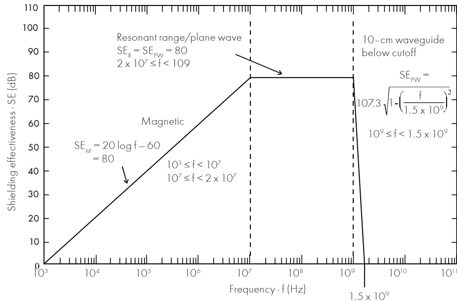
Minimum HEMP shielding effectiveness requirements acc. MIL-STD-188-125 part 1 and part 2
