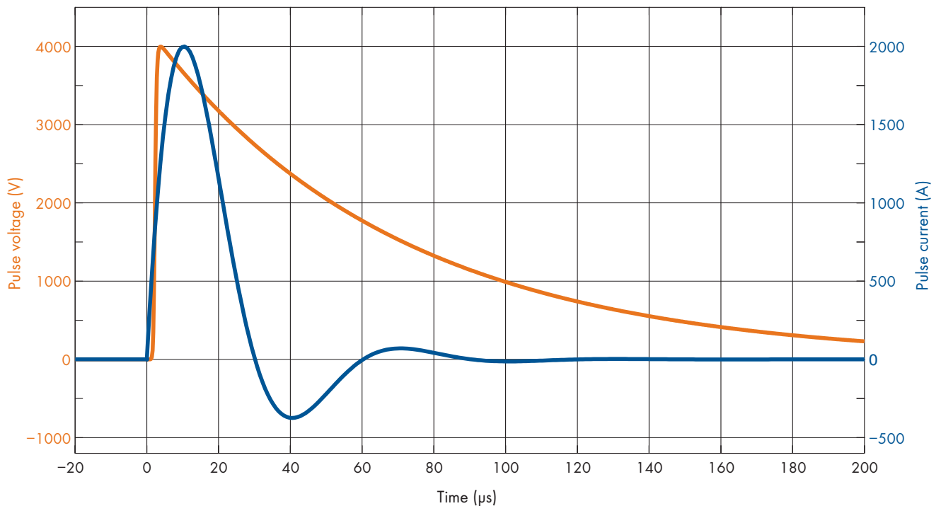
Input surge pulse of a combined surge voltage / current generator
