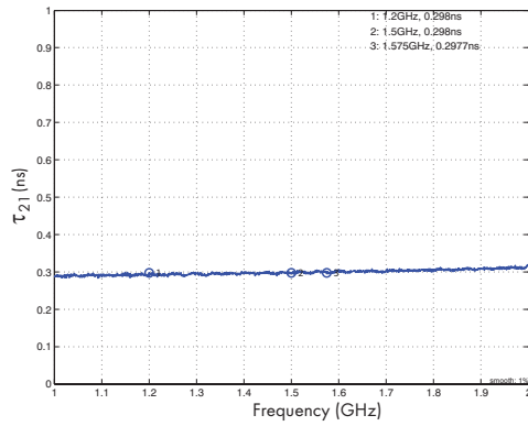
Group delay
