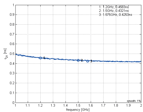
Group delay
