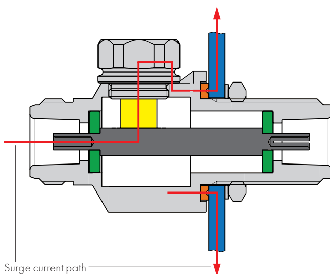
Operating principle of GDT lightning EMP protectors
