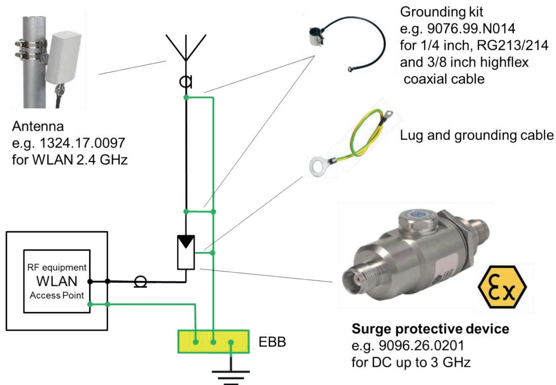
Figure 1: Wireless LAN equipment arrangement, from access point to the antenna with surge protective device
