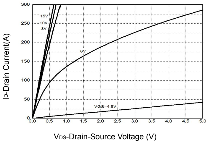
Figure 5: Output Characteristics
