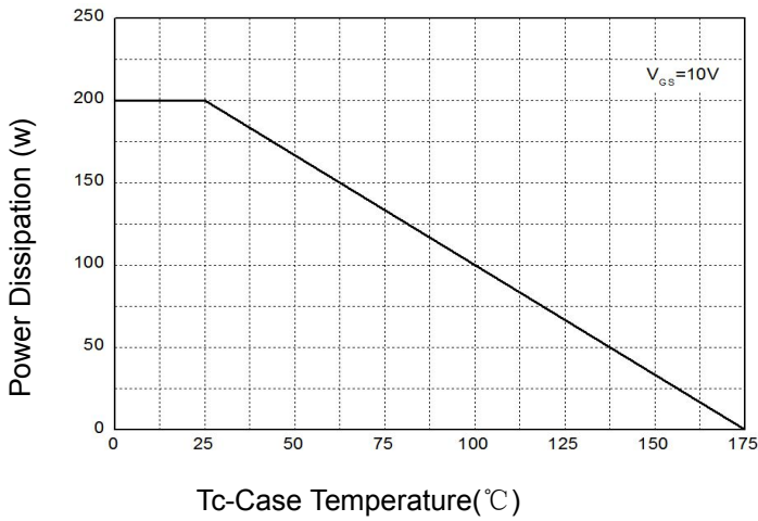
Figure 1: Power Dissipation
