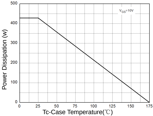
Figure 1: Power Dissipation
