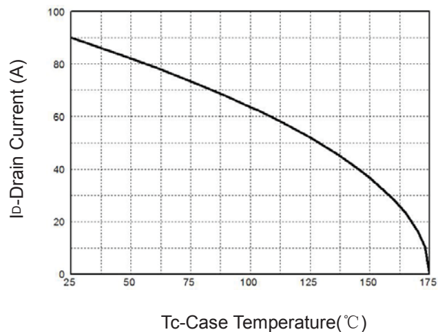
Figure 2: Drain Current
