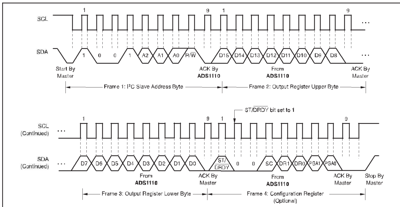
Figure 2. Timing Diagram for Reading From the HT8110A
