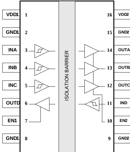
Figure 2. CMT8041x Pin List
