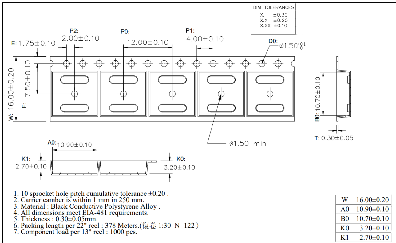
Figure 16. CMT804X WB SOIC-16 Tape and Reel Information
