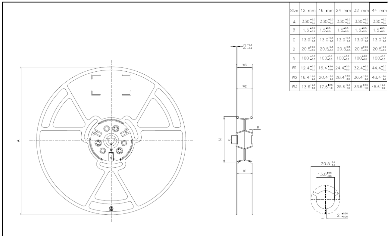
Figure 15. CMT804X WB SOIC-16 Tape and Reel Information
