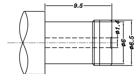
Matching Plug
