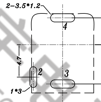
PCB HOLES(THE PATTERN SIDE) T=1.6
