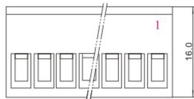
HX39603-NA (5271/3.96)
