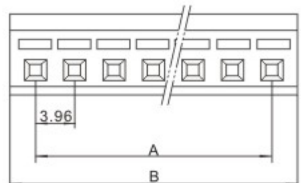
HX39606-Y (5195)
