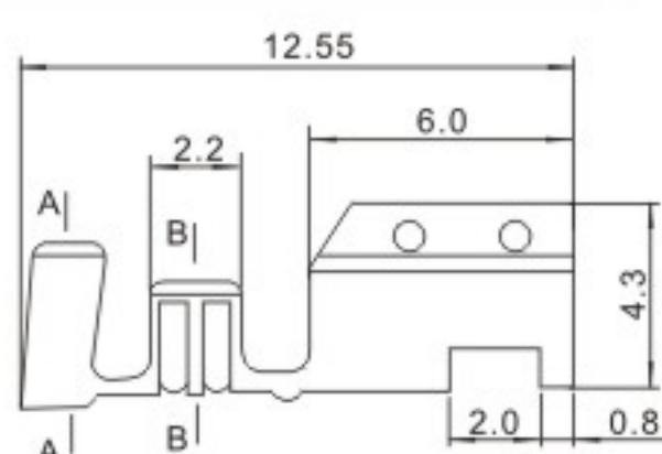
HX39606-Y (5195)
