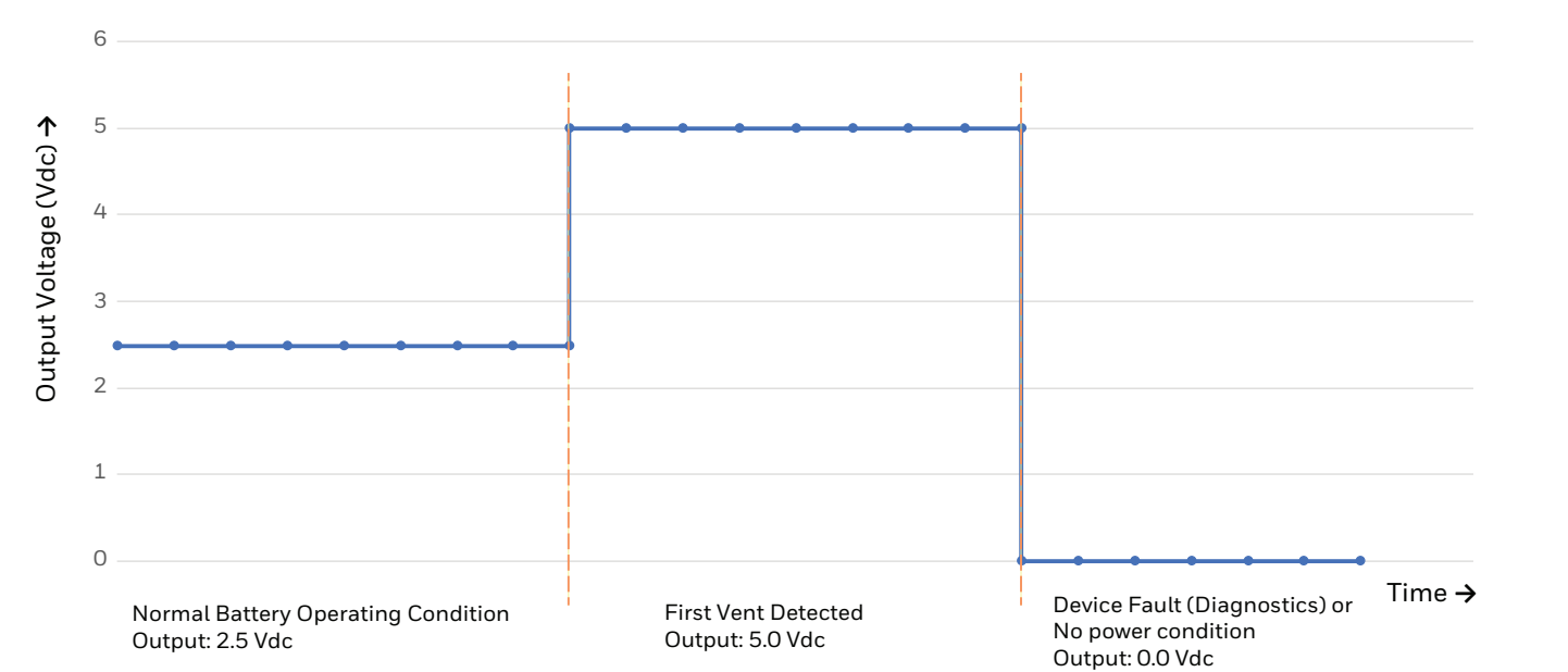
Figure 3. Output Signal During Normal Battery Operating Condition and When First Vent is Detected
