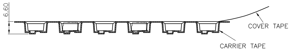
SECTION P-P
