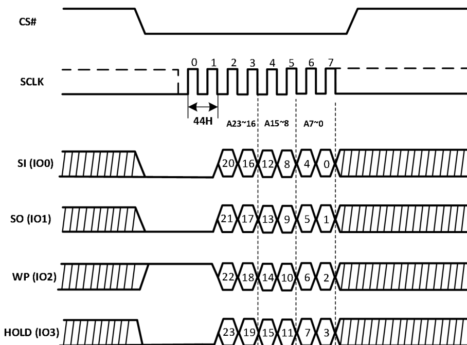
Figure-47. Erase Security Register Sequence Diagram (QPI)
