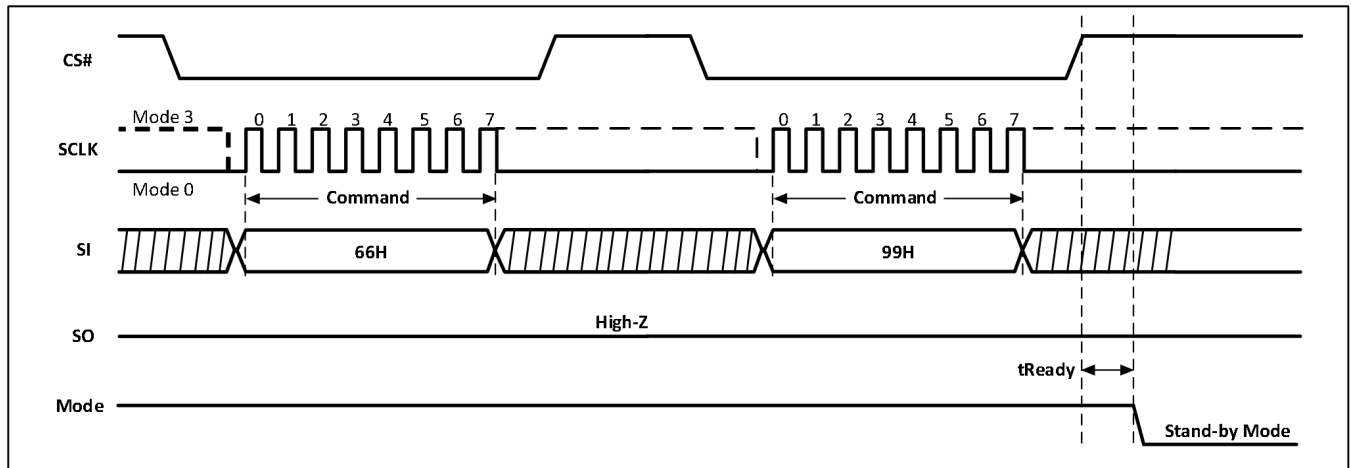
Figure-81. Reset Enable and Reset Sequence Diagram
