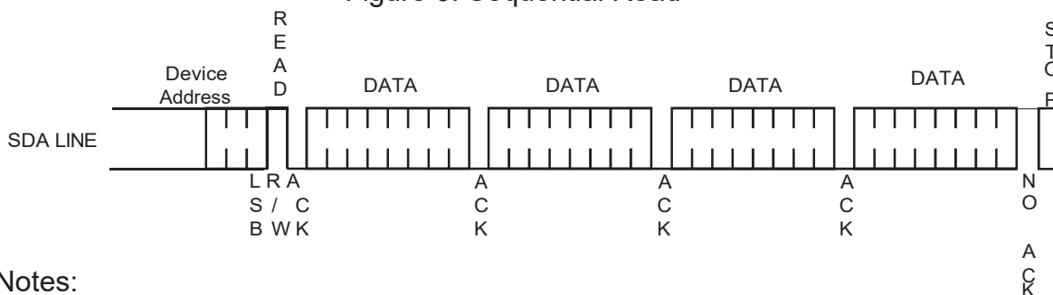
Figure 6: Sequential Read
