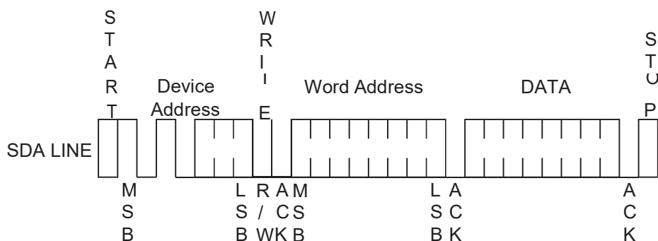
Figure 3: Byte Write
