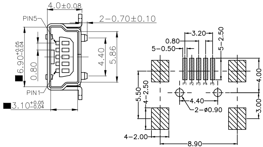
RECOMMENDED PCB LAYOUT(TOP VIEW) GENERAL TOLERANCES:±0.05
