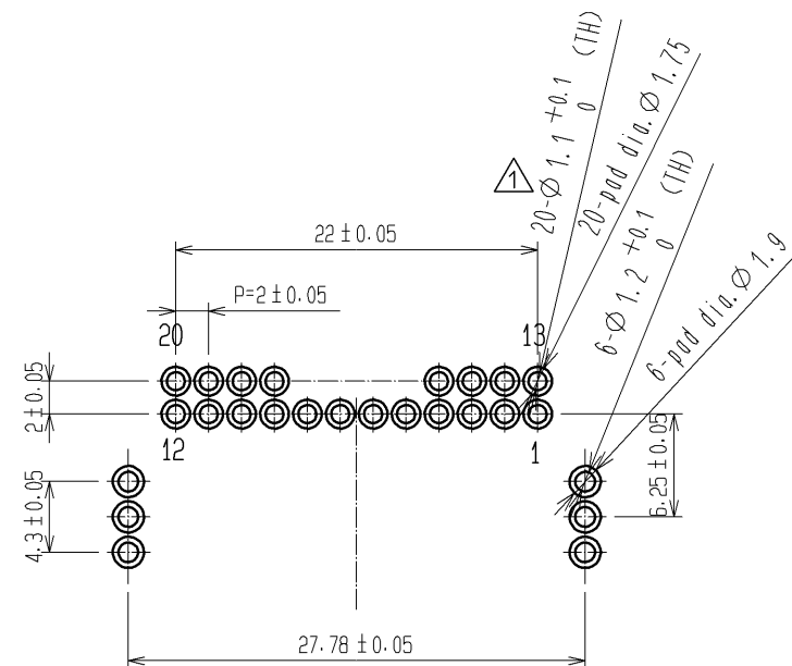
RECOMMENDED PC BOARD PATTERN (CONNECTOR SIDE) AND PIN No.
