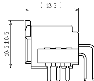
MATED CONNECTORS
