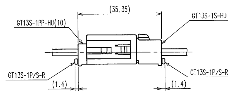
MATED CONNECTORS
