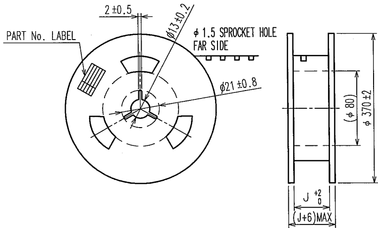
SYTLE AND DIMENSION OF REEL
