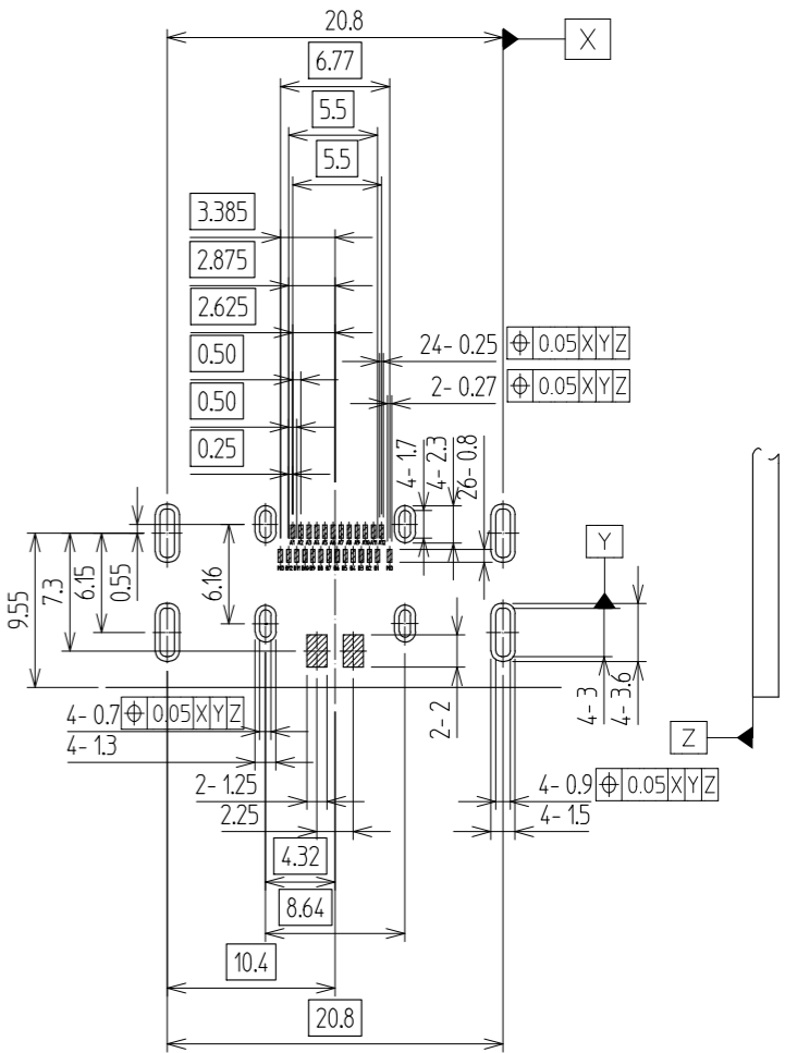
⑥ RECOMMENDED PCB LAYOUT (TOP-VIEW) (GENERAL TOLERANCE : ±0.05)
