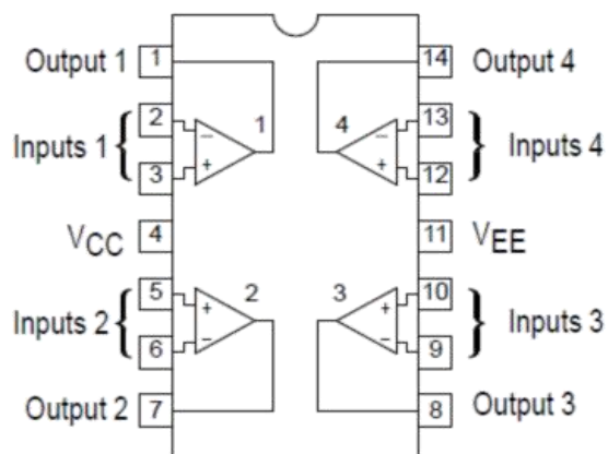
DIP-14/SOP-14/TSSOP-14
