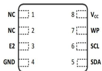
DFN-8 2*3
