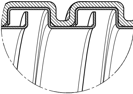
Detail X (Prinzip/principle)
