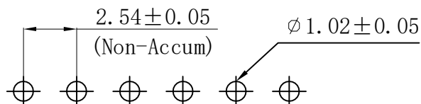
PCB LAYOUT
