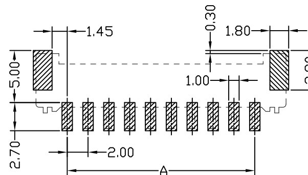
PCB LAYOUT
