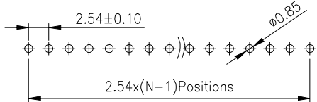
Recommended P.C.B Layout(Top Side) (PCB BOARD TOLERANCE±0.05)
