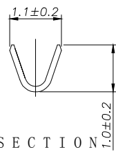
SECTION A - A
